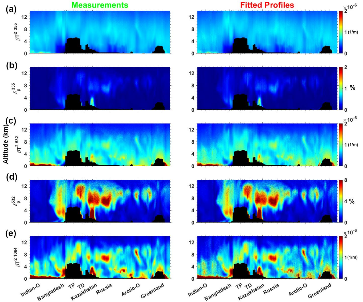
Figure 6. Comparison of Lidar pseudo-observations (left) and fitted profiles (right): Attenuated Backscatter ( \beta_T ) at (a) 355 nm, (c) at 532 nm, and (e) at 1064 nm, and Particle-Volume Depolarization ( \delta ) at (b) 355 nm, (d) 532 nm across the selected transect. (The black shading area indicates the elevation.)
