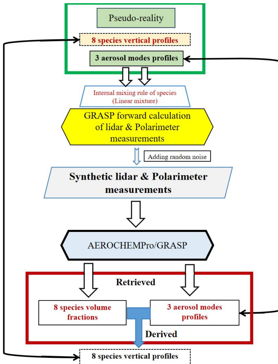
335 Figure 4. Steps to simulate Lidar and Polarimeter synthetic measurements.
