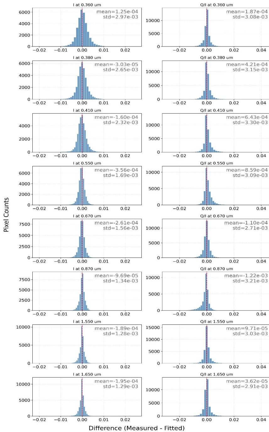
Figure 7. Histograms of Residuals (Measured – Fitted) for AOS polarimeter observations in 8 wavelengths across all scattering angles and pixels of the selected transect.
