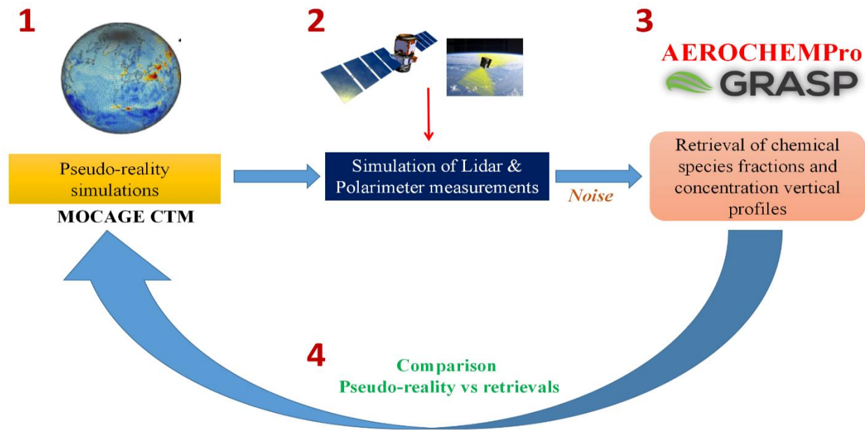
150 Figure 1. Scheme of the full observing system simulation experiment implemented for evaluating the performance of AEROCHEMPro.
