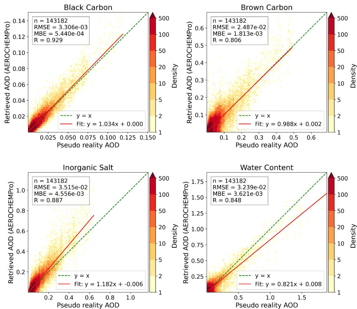
Figure 12. Comparison of aerosol optical depth (AOD) at 532 nm for fine particles (black carbon, brown carbon, inorganic 845 salt) and AOD contribution by water uptake, covering the entire globe.
