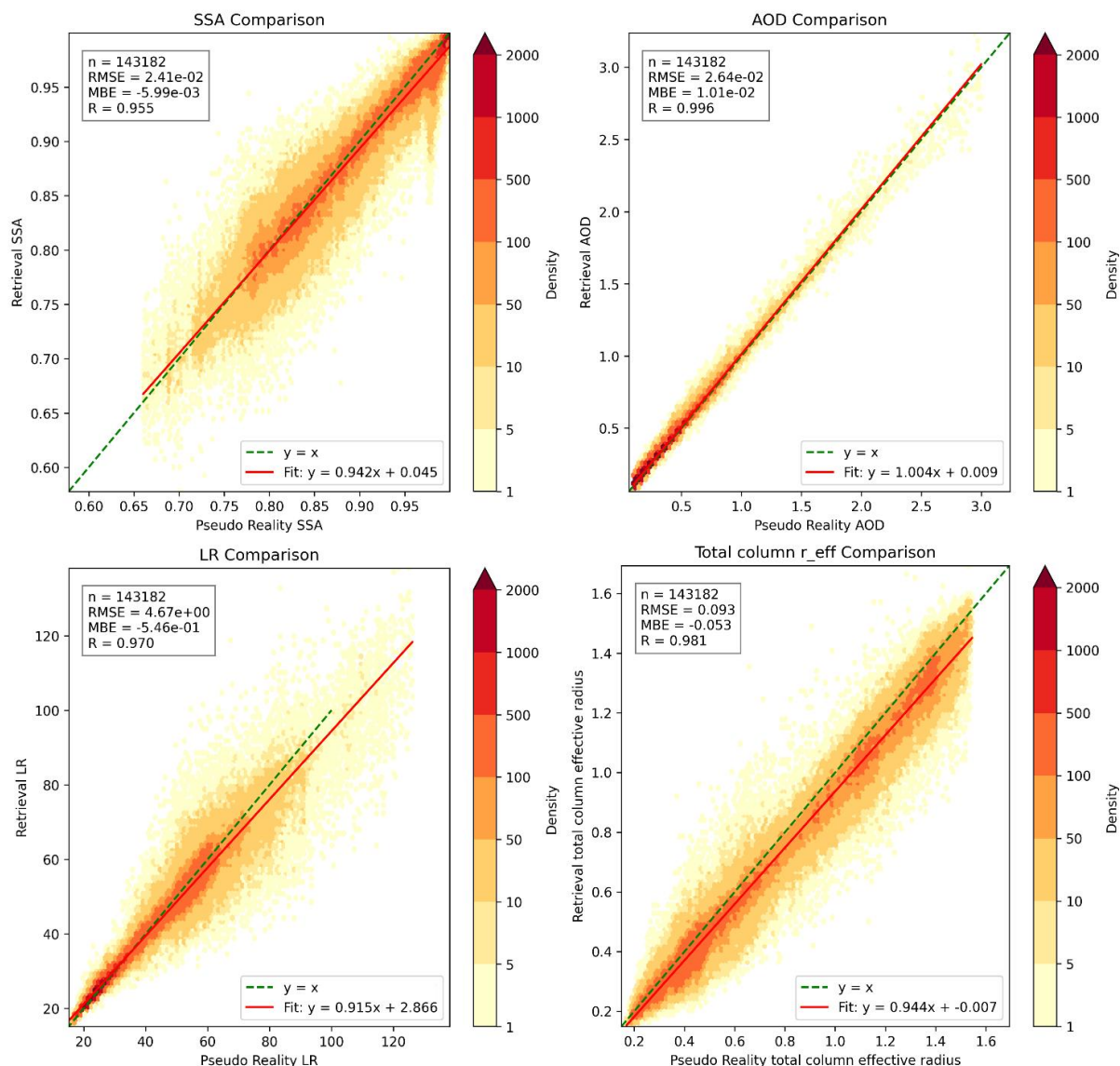
Figure 11. Comparison of column-integrated aerosol optical properties at 532 nm (Single Scattering Albedo (SSA), Aerosol Optical Depth (AOD), Lidar Ratio (LR), and Total column effective radius ( r_{\text{eff}}^{\text{TC}} )) covering the entire globe.
