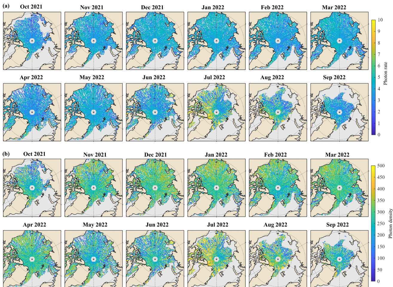
815 Figure A5. Monthly distributions of HRFM classification features from October 2021 to September 2022. (a) Monthly mean photon rate and (b) monthly mean photon density on the 25 km Arctic grid.
