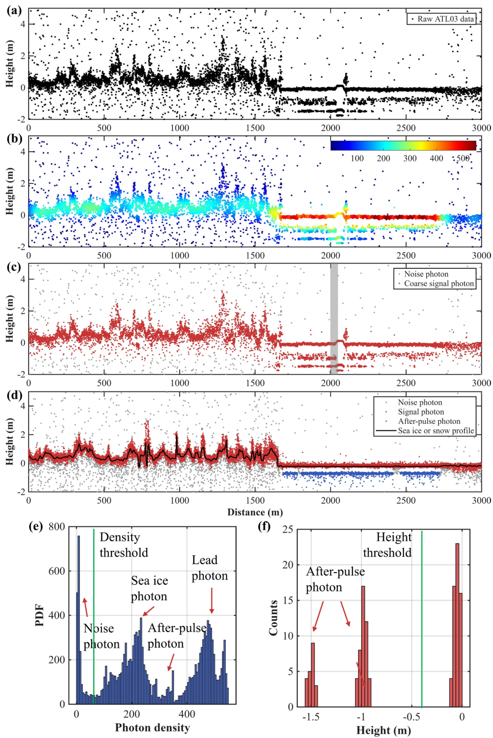
805 Figure A1. Same as Figure 3, but for the weak beam of ATL03_20190526002946_08820304_006_02 over the Lincoln Sea.
