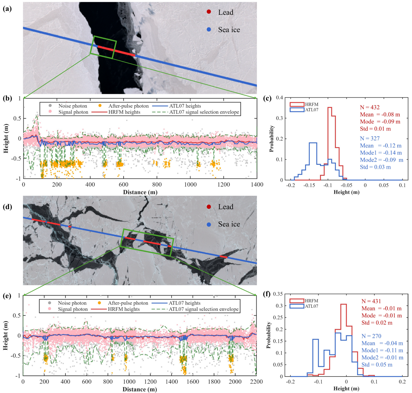
510 Figure 8. Surface-height retrieval over open-water leads and comparison between HRFM and ATL07 for 515 ATL03_20220424135203_04961504_006 and ATL03_20220510145813_07411505_006. (a, d) Coincident Sentinel-2 imagery showing the ICESat-2 ground tracks and HRFM surface-type classification. Red and blue points indicate lead and sea-ice segments, respectively, and the green boxes mark the enlarged regions shown in the photon-profile panels. (b, e) Along-track ATL03 photon clouds and surface-height retrievals within the selected lead regions. Gray, pink, and orange points denote background, signal, and after-pulse photons identified by HRFM, respectively. The green dashed lines represent the ATL07 signal-selection envelope. The
