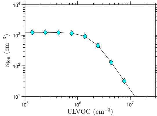
Figure 6. Ion concentrations vs ULVOC. Negative and positive ions have the same concentration; each is near 1200 \text{ cm}^{-3} at low ULVOC. Ion induced nucleation depletes the primary ions for \text{ULVOC} > 10^6 \text{ cm}^{-3} .
