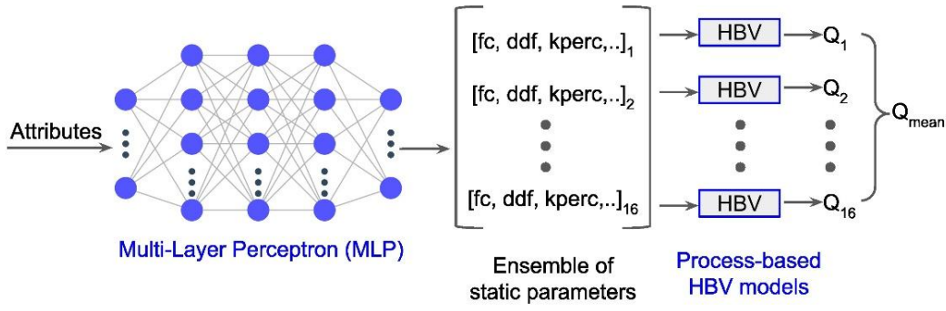
200 Figure 2: Schematic of differentiable MLP with ensemble HBV architecture with 16 independent modules.
