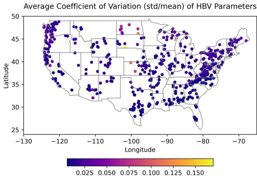
Figure 6: Spatial distribution of the average coefficient of variation of HBV parameters between input sequences estimated by the LSTM+HBV differentiable model. Each dot represents a study basin, with color intensity indicating the magnitude of the average temporal variability of the parameter set.
