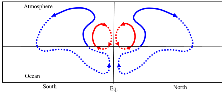
165 Figure 2: Schematic representation of coupled ocean–atmosphere “Latent cells”. Dotted lines denote non-gaseous- phase mass transport associated with the hydrological cycle, terminating at regions of net evaporation in the subtropics. These regions act as sources of atmospheric mass, where water vapour enters the atmosphere. Solid lines denote gaseous source–sink flows that originate at these evaporative sources and terminate at regions of net phase change and precipitation (high latitudes and the equator) that remove atmospheric mass and add freshwater to the ocean. Together, 170 these linked source–sink flows form closed circuits across the ocean–atmosphere system. Tropical branches are shown in red and extratropical branches in blue. Adapted from Dey and Döös (2019).
