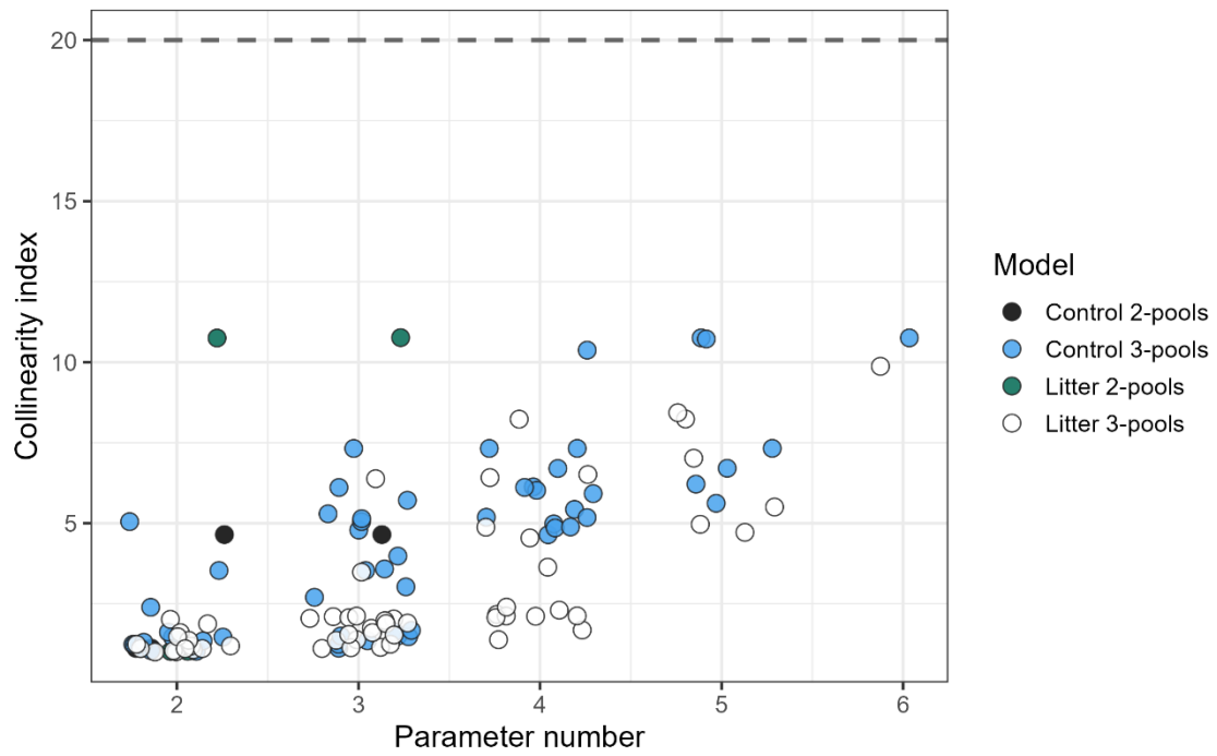
Supplementary Fig. 1: Collinearity index as a function of the number of parameters estimated by the different models. The dashed line indicates the upper limit for acceptable collinearity. All estimated collinearity indices were below 20 across models.
