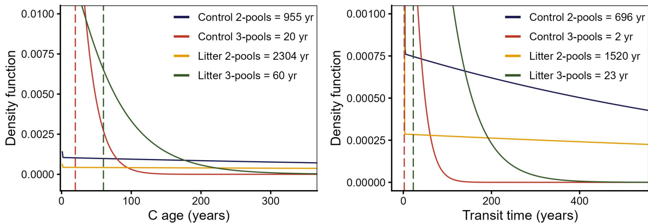
295 Figure 4. Solid lines show the probability density distribution and dashed lines show the mean values of C age and transit time for the 2-pool model that best fitted respiration data and 3-pool models applied to control soils and litter-addition treatments. The 2-pool models that best fitted C contents are not shown, as their C ages and transit time estimations were the order of tens of thousands of years.
