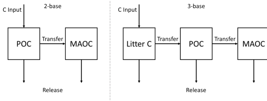
Figure 1. 2-Base and 3-Base models. The arrows represent the respiration fluxes (downwards arrows) and transfers processes (rightwards arrows) and not the full mathematical expressions.
