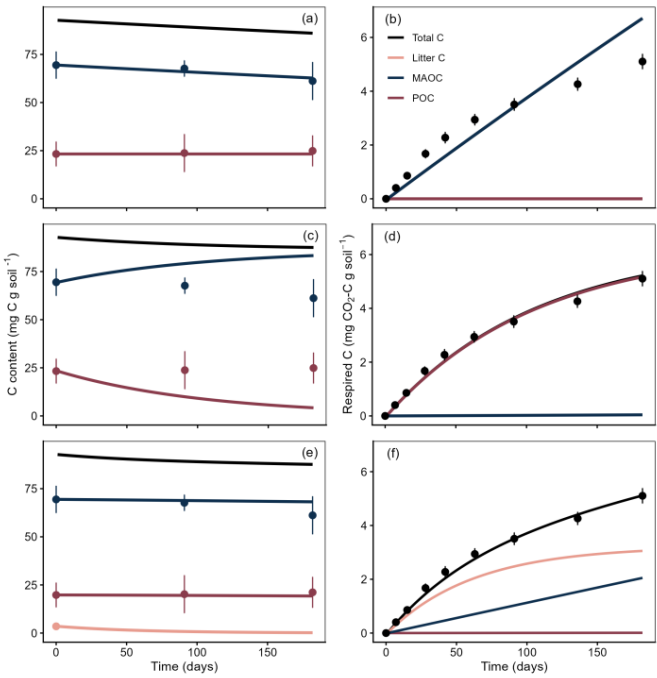
370 Figure 3. C content (left panels) and respired C (right panels) in each C pool and total in litter-addition treatments. In black, Total C; in dark blue, MAOC; in dark red, POC; in pink, Litter C. The lines represent the model estimations, while the points represent the observed data. (a) and (b) 2-pool models that best fitted C pools content. (c) and (d) 2-pool models that best fitted the respiration. (e) and (f) 3-pool model.
