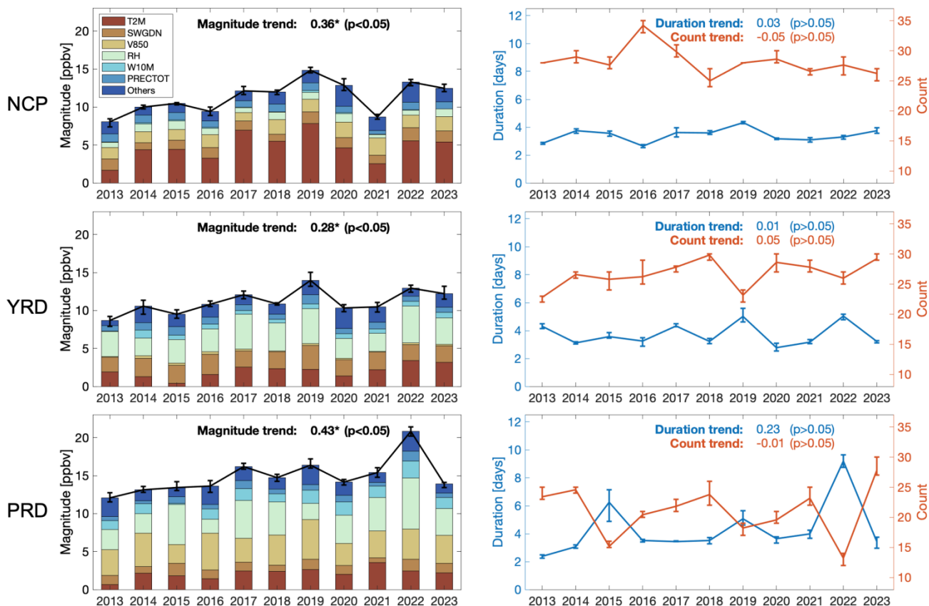
Figure 5. Left column: Magnitude of positive MOA events during warm seasons from 2013 to 2023 for NCP (top), YRD (middle), and PRD (bottom). Bars represent contributions from individual meteorological variables. Trends in unit of ppbv/year are shown inset. Right column: Duration and count of positive MOA events over the same period. Results are averaged across five ML models, with error bars indicating the range among models.
