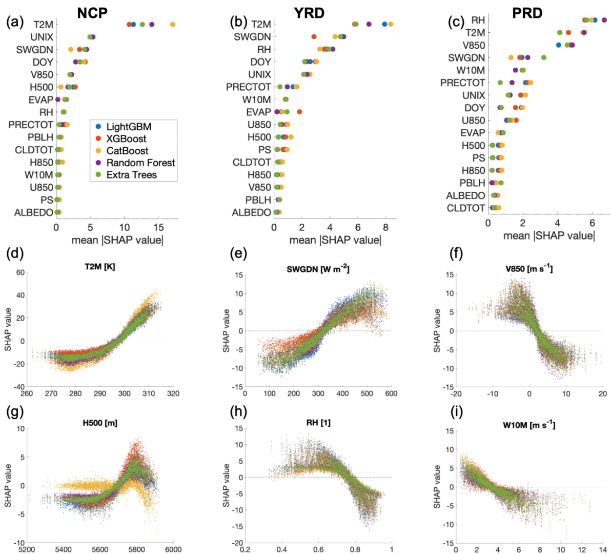
245 Figure 2. (a)–(c): Global feature importance for the three regions: North China Plain (NCP, left column), Yangtze River Delta (YRD, middle column), and Pearl River Delta (PRD, right column), calculated by averaging the absolute SHAP values across all days. (d)–(i): Scatter plots of selected meteorological variables versus their SHAP values, illustrating local explainability. Each point represents a daily observation, and different colors correspond to different ML models.
