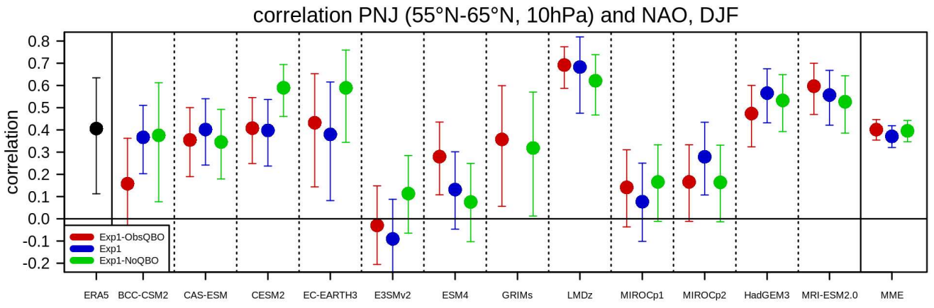
Figure 10: Correlation between the strength of the polar night jet (55°N-65°N, 10 hPa) and the NAO index in DJF for the models and ERA5. The error bars denote the 95% confidence interval of the correlation.
