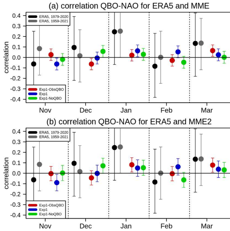
Figure 11: Pearson correlation between the QBO phase (5°S-5°N, 50 hPa) and strength of the NAO index from November to March for (a) the multi-model mean MME simulations and (b) the multi-model mean MME2 of only those simulations which exhibit a statistically significant HT effect on the PNJ in DJF, compared to ERA5. Error bars denote the 95% confidence interval of the correlation calculated across all simulations (i.e. models and ensemble members) contributing to the MME and MME2.
