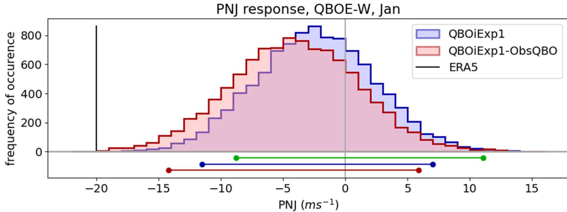
Figure 5: Distribution of PNJ values when sub-sampling the multi-model ensembles with a QBOE-W sample size equivalent to observations. The distributions shown use Monte-Carlo random sub-sampling-with-replacement with 10,000 iterations for clarity, whereas the statistics given in the main text uses the more statistically robust sub-sampling-without-replacement. The distributions for Exp1-ObsQBO (red) and Exp1 (blue) are accompanied by horizontal lines of similar colours beneath the graph indicating the \pm 2\sigma range. The \pm 2\sigma range for the Exp1-NoQBO distribution (distribution not shown for clarity) is included as the green line. The vertical black line towards the left represents the observed PNJ response. 310
