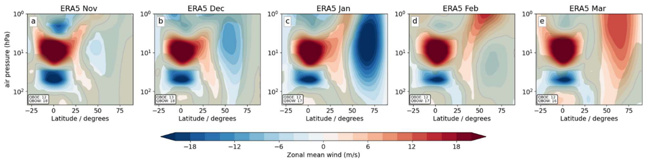
255 Figure 3: Monthly evolution of ERA5 zonal-mean zonal wind, composited by QBOE minus QBOW conditions for November – March over the period 1979 - 2020. Regions not significant at the 2-sided 90% level (5% - 95%) are shaded in olive-green. QBOE and QBOW sample sizes are noted in the bottom left corner of each panel.
