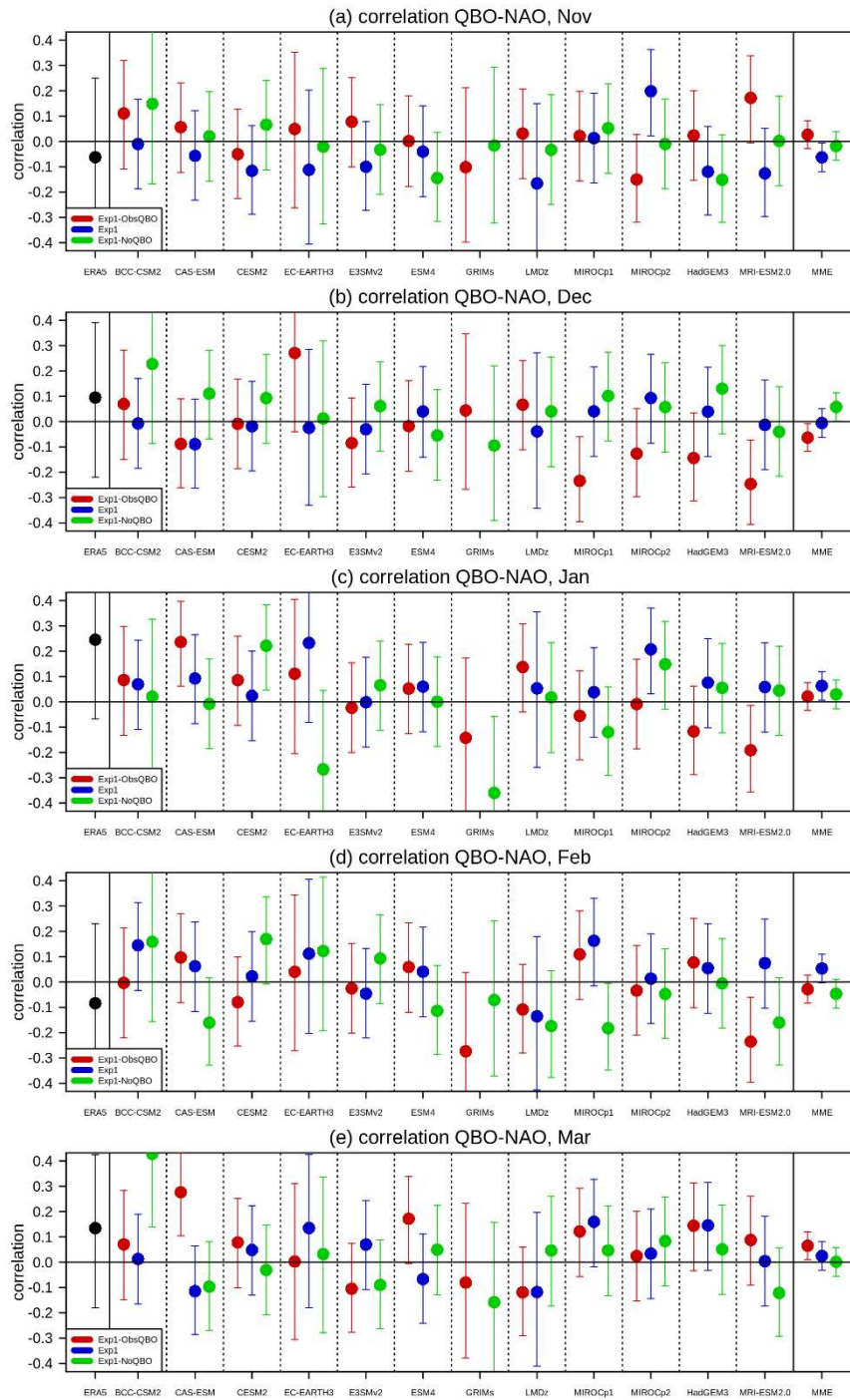
725 Figure A3: Correlation between the QBO (5°S-5°N and 50 hPa) and the NAO index in (top to bottom) November, December, January, February and March for ERA5, all models, and the MME for each experiment.
