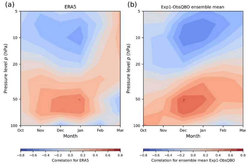
240 Figure 2: Correlation of the zonal-mean zonal wind at 60°N with the equatorial zonal-mean zonal winds from 100 hPa to 5 hPa for October through to March in (a) the ERA5 dataset 1979 – 2020, and (b) the Exp1-ObsQBO multi-model ensemble mean.
