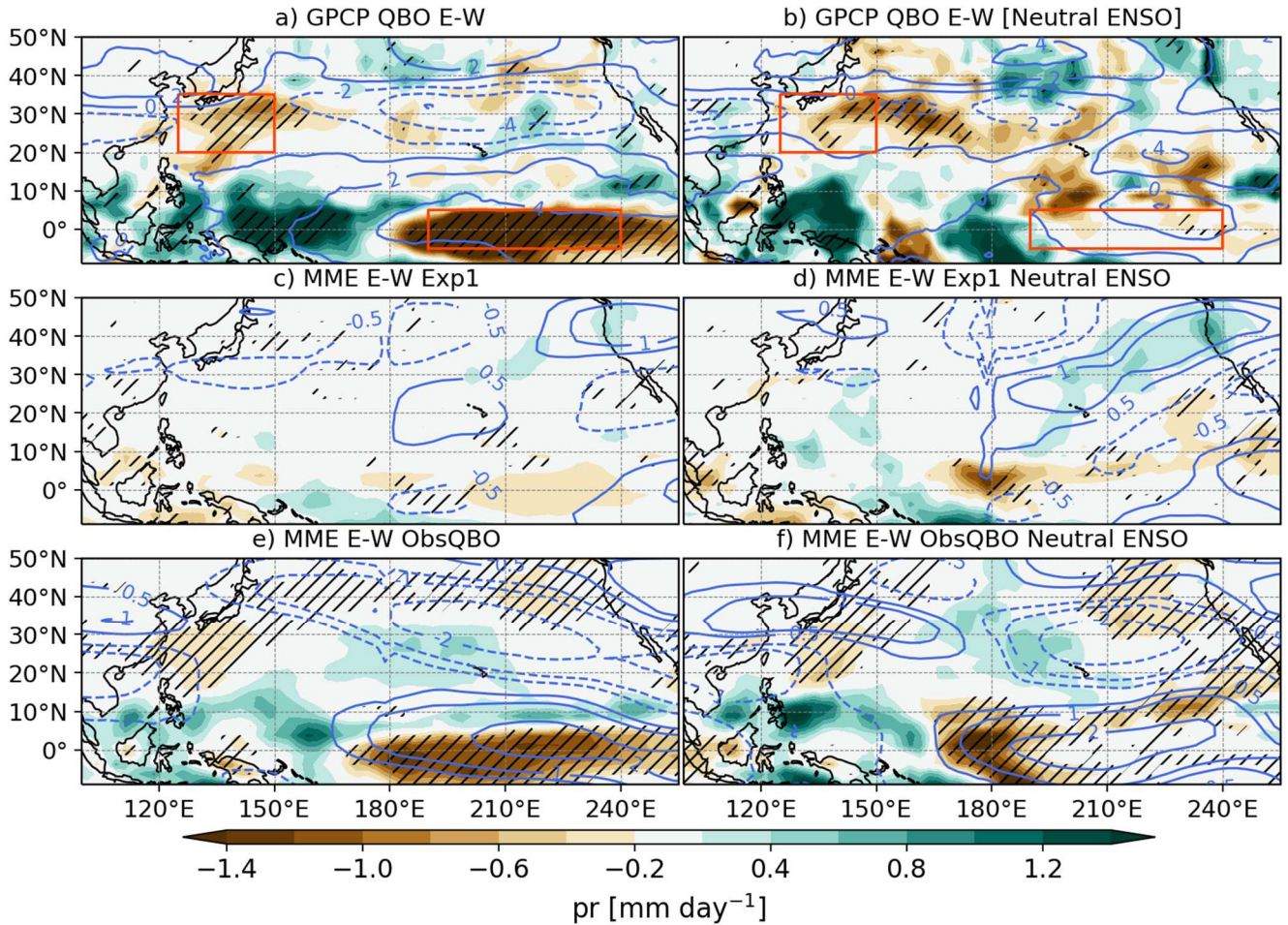
Figure 13: DJF mean differences (QBO E-W) in precipitation (shading in \text{mm day}^{-1} ) and zonal wind at 200 hPa (contours in \text{m s}^{-1} ). Results are shown for observations considering a) all cases and b) only neutral ENSO conditions. QBOi MME of the experiments (c-d) Exp1 and (e-f) Exp1-ObsQBO. Hatching in (a-b) denotes statistical significance of the precipitation differences to the 95% confidence level according to a bootstrap test whereas in (c-f) the hatching shows where at least 70% of the models agree on the sign of the difference.
