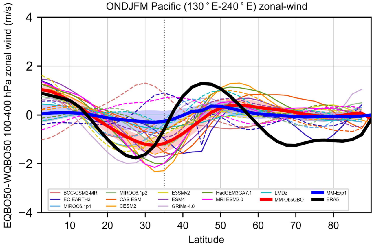
575 Figure 12: October-March QBOE minus QBOW 100 – 400 hPa pressure-weighted zonal-mean zonal wind anomalies, averaged over the North Pacific (130°E – 240°E) for the period October 1979 to March 2020. The zonal wind for each ensemble member (within a given model and experiment) is deseasonalized to produce anomalies. These anomalies are then composited by QBOE and QBOW phases before subtraction. Each model's zonal-wind anomalies are shown with a characteristic colour, which is used to denote its Exp1 response (dashed line) and its Exp1-ObsQBO response (solid line). The thick black curve shows the ERA5 580 anomalies over the experiment period and the thick blue and red curves show multi-model averages of the Exp1 and Exp1- ObsQBO ensembles, respectively; we average across a model's respective ensemble members before computing the multi-model averages so that each model is given equal weight in the multi-model average. 2.5 and 97.5 percentile confidence intervals, denoted by shading, are computed about Exp1 and Exp1-ObsQBO by resampling the model ensemble means 10,000 times with 585 replacement. The vertical dashed line denotes the latitude of the climatological STJ from October-to-March across all years over the Pacific in ERA5.
