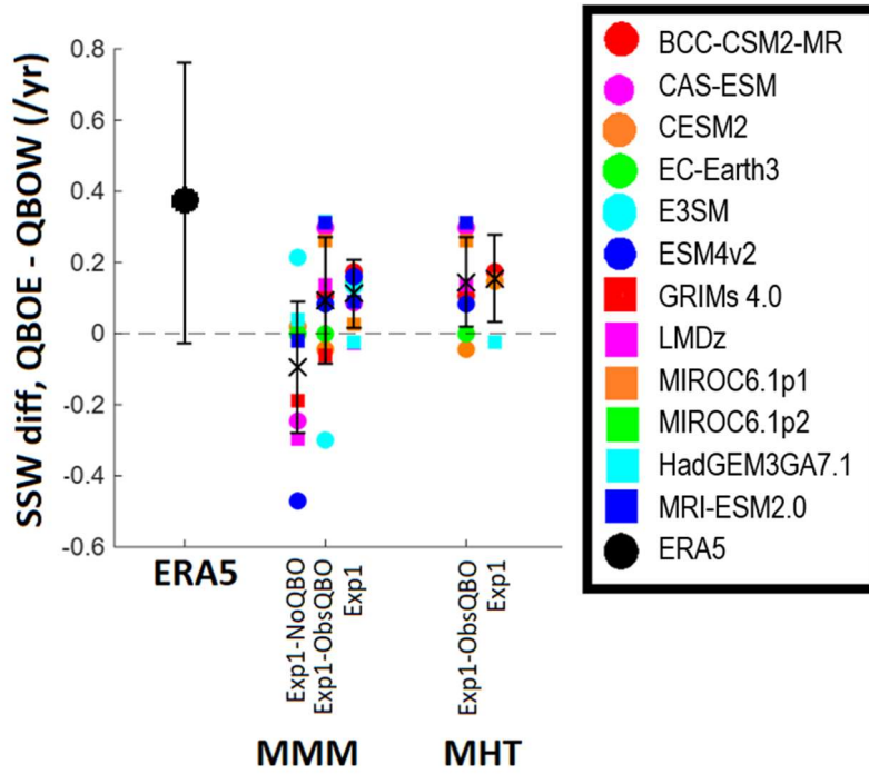
440 Figure 8: The QBOE-W difference in SSW frequencies in each experiment and ERA5 data. Model results are grouped together to show the results from across all models (MMM) and those found to have significant HTE (MHT = Mean Holton-Tan). In MMM, Exp1-NoQBO is also shown, where the QBOE-W years are the same as in Exp1-ObsQBO and ERA5. Individual model means, calculated across ensemble members, are indicated by circles/squares, and the multi-model means and standard deviations are indicated by black crosses and error bars respectively. For ERA5, the Poisson uncertainty, \frac{\sqrt{N}}{T} where N is the number of SSW's and T is the number of years, is used.
