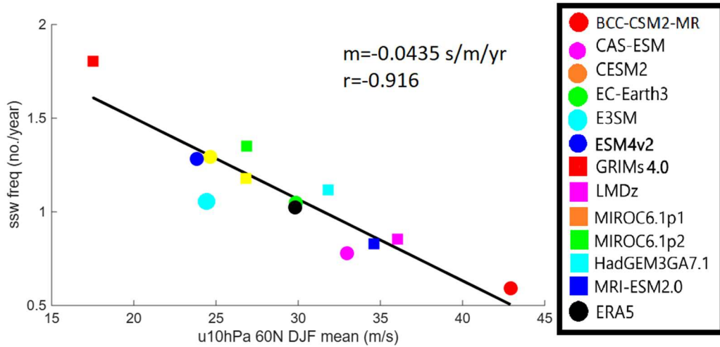
Figure 7: Scatter plot showing the regression between DJF PNJ strength (x-axis) and Sudden Stratospheric Warming (SSW) frequency (y-axis) across the different models in the Exp1-ObsQBO experiment, and also for the ERA5 reanalysis. Slope ( m ) and correlation coefficient ( r ) are calculated from the model values only.
