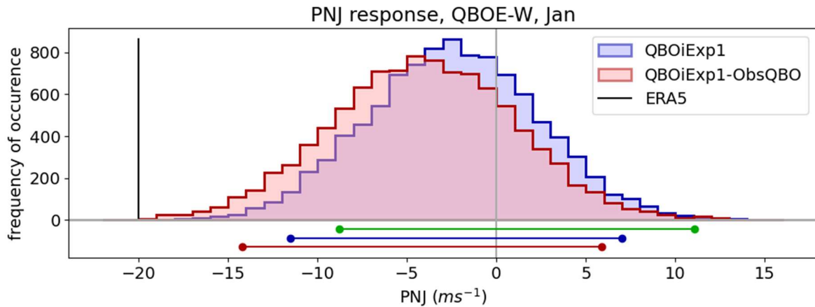
Figure 5: Neither the Exp1 nor Exp1-ObsQBO experiments capture the magnitude of the observed January PNJ response to QBO. Distribution of PNJ values when sub-sampling the multi-model ensembles with a QBOE-W sample size equivalent to observations. The distributions shown use Monte-Carlo random sub-sampling-with-replacement with 10,000 iterations for clarity, whereas the statistics given in the main text uses the more statistically robust sub-sampling-without-replacement. The distributions for Exp1-ObsQBO (red) and Exp1 (blue) are accompanied by horizontal lines of similar colours beneath the graph indicating the \pm 2\sigma range. The \pm 2\sigma range for the Exp1-NoQBO distribution (distribution not shown for clarity) is included as the green line. The vertical black line towards the left represents the observed PNJ response.
