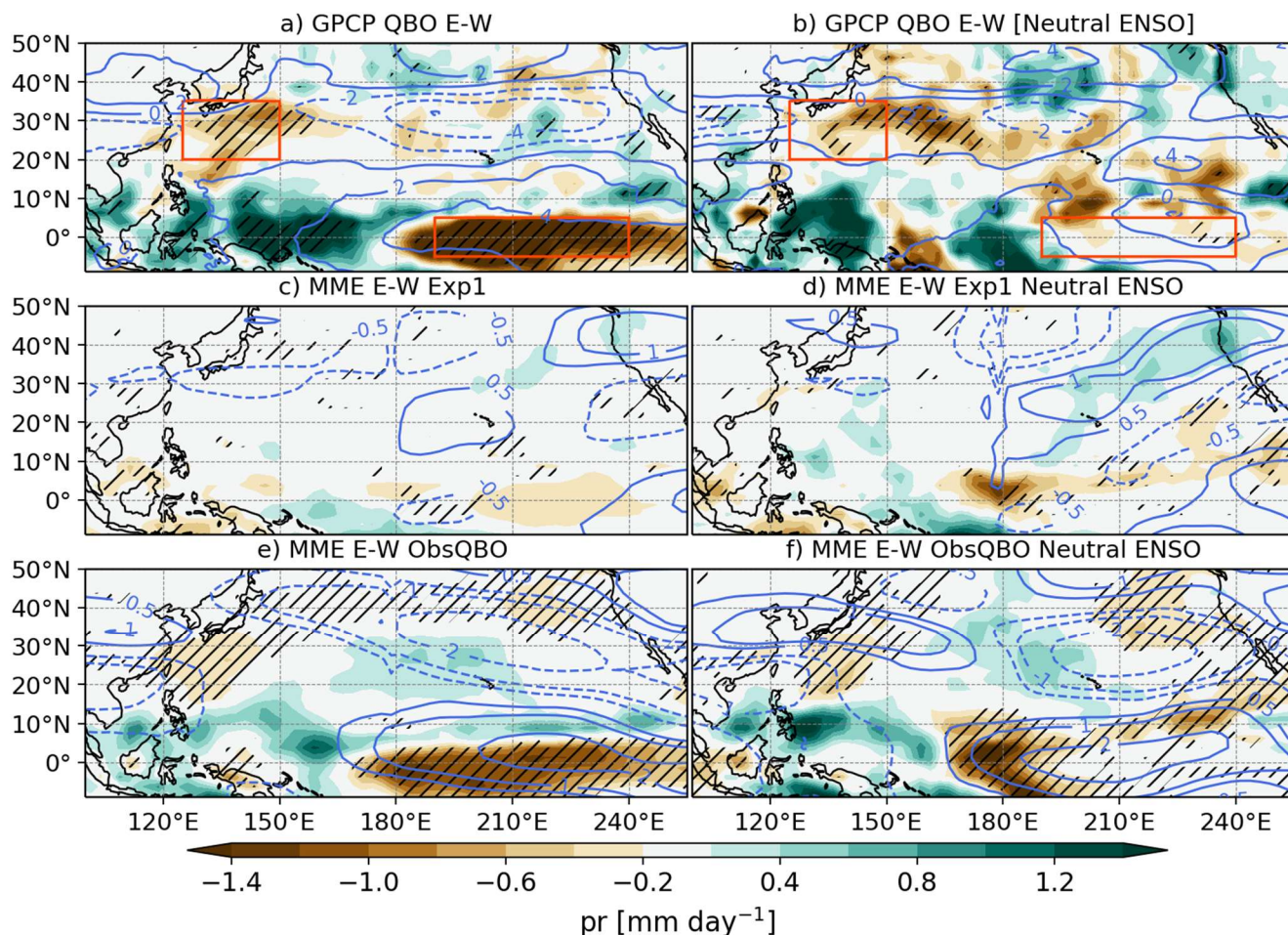
Figure 13: Nudging modifies the tropical precipitation and subtropical upper level wind response to the QBO. DJF mean differences (QBO W-EE-W ) in precipitation (shading in \text{mm day}^{-1} ) and zonal wind at 200 hPa (contours in \text{m s}^{-1} ). Results are shown for observations considering a) all cases and b) only neutral ENSO conditions. QBOi MME of the experiments (c-d) Exp1 and (e-f) Exp1-ObsQBO. Hatching in (a-b) denotes statistical significance of the precipitation differences to the 95% confidence level according to a bootstrap test whereas in (c-f) the hatching shows where at least 70% of the models agree on the sign of the difference.
