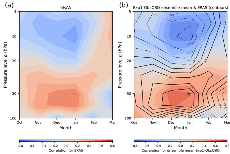
Figure 2: Correlation of the zonal-mean zonal wind at 60^{\circ}\text{N} with the equatorial zonal-mean zonal winds from 100 hPa to 5 hPa for From NovemberOctober through to JanuaryMarch The strongest correlation between the Polar Night Jet (zonal-mean zonal wind at 60^{\circ}\text{N} , 10 hPa) correlates most strongly with and the equatorial QBO zonal mean zonal winds in the QBO region over early-mid boreal winter occurs at around 50 hPa in (a) the ERA5 dataset 1979 – 2020, and (b) the Exp1-ObsQBO multi-model ensemble mean. The ERA5 contour lines are overlaid onto (b) for comparison.
