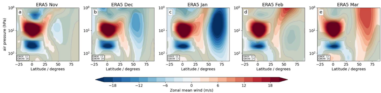
Figure 3: Monthly evolution of The observed PNJ response to the equatorial QBO at 50 hPa peaks in January. Panels show ERA5 zonal-mean zonal wind, composited by QBOE minus QBOW conditions for QBOE-W monthly evolution, (a-e) November – March over, for, the period 1979 - 2020. Regions not significant at the 2-sided 90% level (5% - 95%) are shaded in olive-green.
