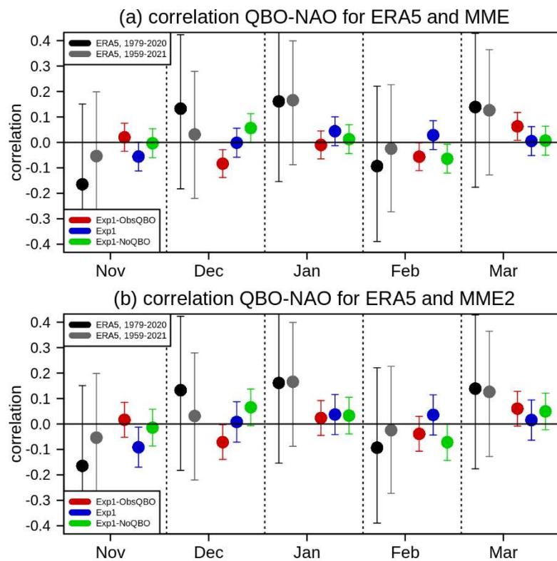
Figure A4: Same as Figure 11 but using a two-station sea level pressure difference NAO index (Ponta Delgado 37.7 N, 25.7 W and Reykjavik 64.1 N, 21.9 W).
