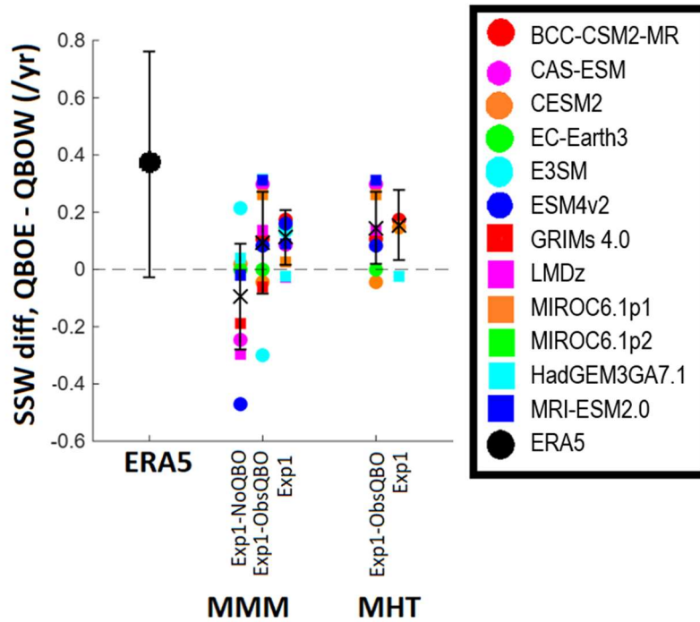
Figure 8: The influence of the QBO phase on the SSW frequency seen in observations is weakly captured by the Exp1 and Exp1-ObsQBO experiments. The plot shows the QBOE-W difference in SSW frequencies distribution of average SSW frequencies during each QBO phase in each experiment and ERA5 data. Model results are grouped together to show the results from across all models (MMM) M = multi-model ensemble mean and those found to have significant HTE (MHT = Mean Holton-Tan). In MMM, Exp1-NoQBO is also shown, where the QBOE-W years are the same as in Exp1-ObsQBO and ERA5, and those with a relatively strong NH polar vortex (SVMM=Strong Vortex Model Mean): a list of models used in the SVMM is provided in Table A3. The ERA5 and model results are also filtered to show the results across all boreal winters (All ENSO) and using La Niña winters only. Individual model means, calculated across ensemble members, are indicated by crosses/circles/squares, and the multi-model means and standard deviations are indicated by filled squares/black crosses and error bars respectively. For ERA5, the Poisson uncertainty, \frac{\sqrt{N}}{T} where N is the number of SSW's and T is the number of years, is used.
