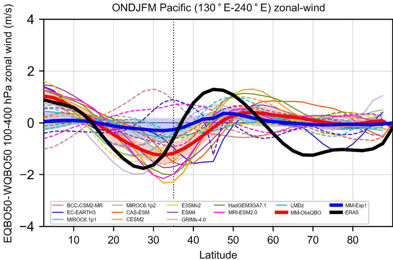
Figure 12: The response of the STJ to QBOW-E is smaller and shifted northwards compared to observations. October-March QBO EW minus QBO WE 100 – 400 hPa pressure-weighted zonal-mean zonal wind anomalies, averaged over the North Pacific ( 130^{\circ}\text{E} - 240^{\circ}\text{E} ) for the time period October 1979 to March 2020. The zonal wind for each ensemble member (within a given model and experiment) is deseasonalized to produce anomalies. These anomalies are then composited by QBOE and QBOW phases before subtraction. The QBOW and QBOE groups are each deseasonalized before subtraction. Each model's zonal-wind anomalies are shown with a characteristic colour, which is used to denote its Exp1 response (dashed line) and its Exp1-ObsQBO
