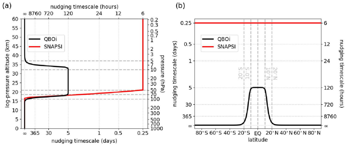
245 Figure 1: Spatial dependence of nudging timescale in (a) the vertical and (b) meridional directions for the QBOi phase-2 nudging experiments Exp1-ObsQBO and Exp1-NoQBO (black curves). The mathematical expressions corresponding to the QBOi profiles shown in (a) and (b) are detailed in Anstey et al., ( in-prep2026 ). Vertical and meridional profiles of nudging timescale from the SNAPSI protocol (Hitchcock et al., 2022) are shown in red for comparison with the QBOi profiles (see Anstey et al., in-prep2026 , Appendix A for further details of the QBOi-SNAPSI comparison).
