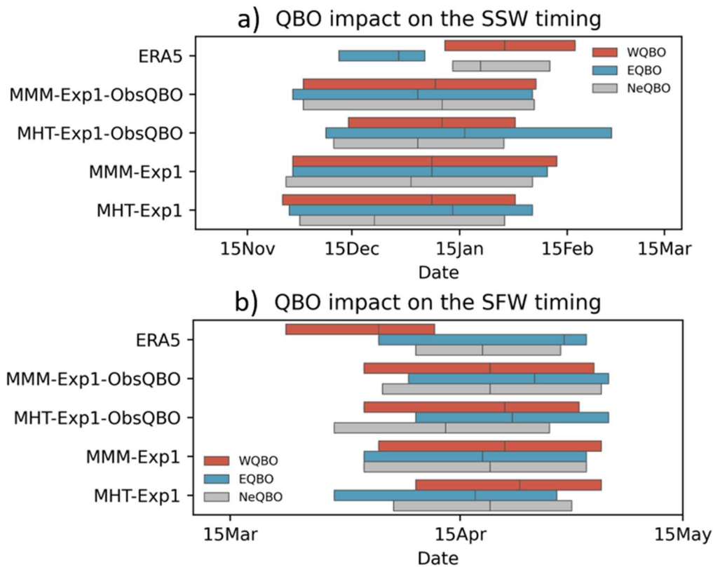
Figure 9: Experiments are unable to capture the significant variations of SSW and SFW timing seen in observations. (a) Timing distribution of (a) mid-winter SSWs and (b) the stratospheric final warming (SFW) dates for easterly (blue), westerly (red), and neutral (grey) QBO years in ERA5, the multi-model mean (MMM) and the Mean Holton-Tan (MHT) subset in Exp1-ObsQBO and Exp1. Colour bars extend from the 25 th to 75 th percentile with the mean indicated by a vertical line.
