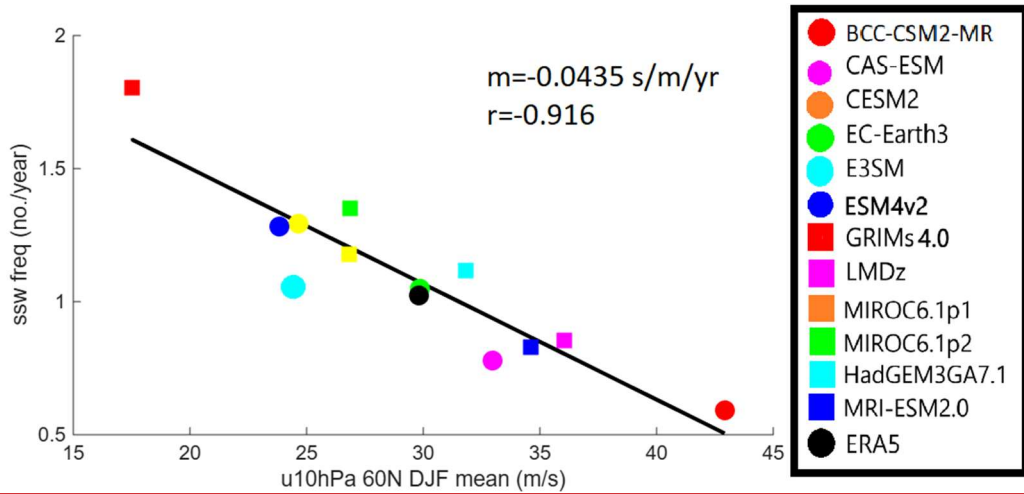
Figure 7: Scatter plot showing the regression between DJF PNJ strength (x-axis) and Sudden Stratospheric Warming (SSW) frequency (y-axis) across the different models in the Exp1-NoQBO-ObsQBO experiment, and also for the ERA5 reanalysis. Slope ( m ) and correlation coefficient ( r ) are calculated from the model values only and displayed inside the scatter plot.
