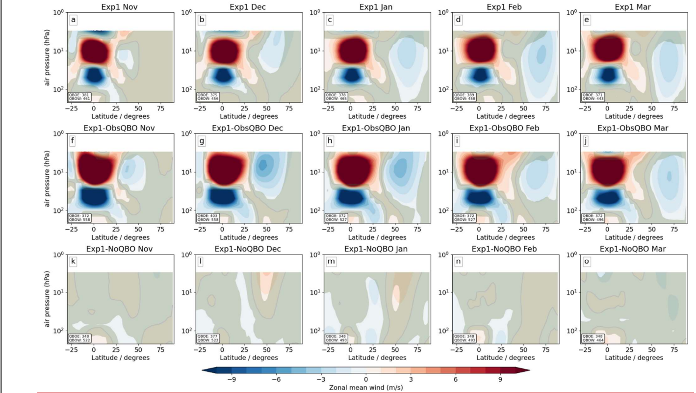
325 Figure 4: As Fig. 3, but for the three experiments. There is a significant PNJ response to the QBO in Exp1 which increases in magnitude in Exp1-ObsQBO. MME zonal-mean zonal wind monthly evolution, November—March (1 st —5 th columns) for each experiment; Exp1 (a – e), Exp1-ObsQBO (f – j), and Exp1-NoQBO (k – o). The colour scale is half that of Fig. 3 in order to reveal the detail in the stratospheric polar vortex.
