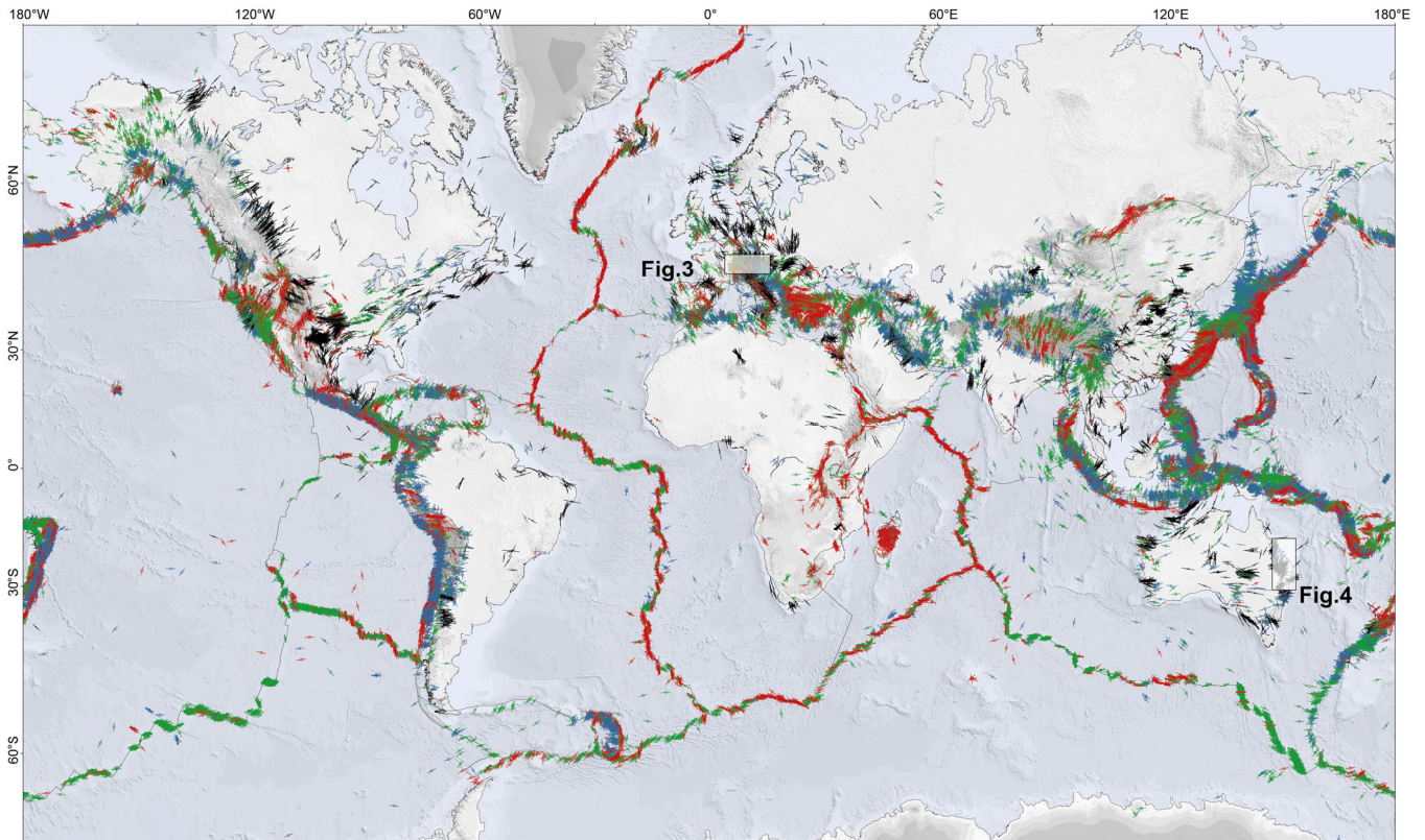
Figure 1. World Stress Map 2025. Lines indicate the orientation of maximum horizontal stress ( S_{Hmax} ). Colours of the lines indicate normal faulting stress regime (red), strike-slip stress regime (green), thrust faulting stress regime (blue), and black for unknown stress regime. Displayed are the 77,365 data records with A-C quality. Grey lines are the plate boundaries from the global tectonic model PB2002 of Bird (2003). Topography and bathymetry is taken from Tozer et al. (2019). Plotting order of the data is from deep to shallow.
