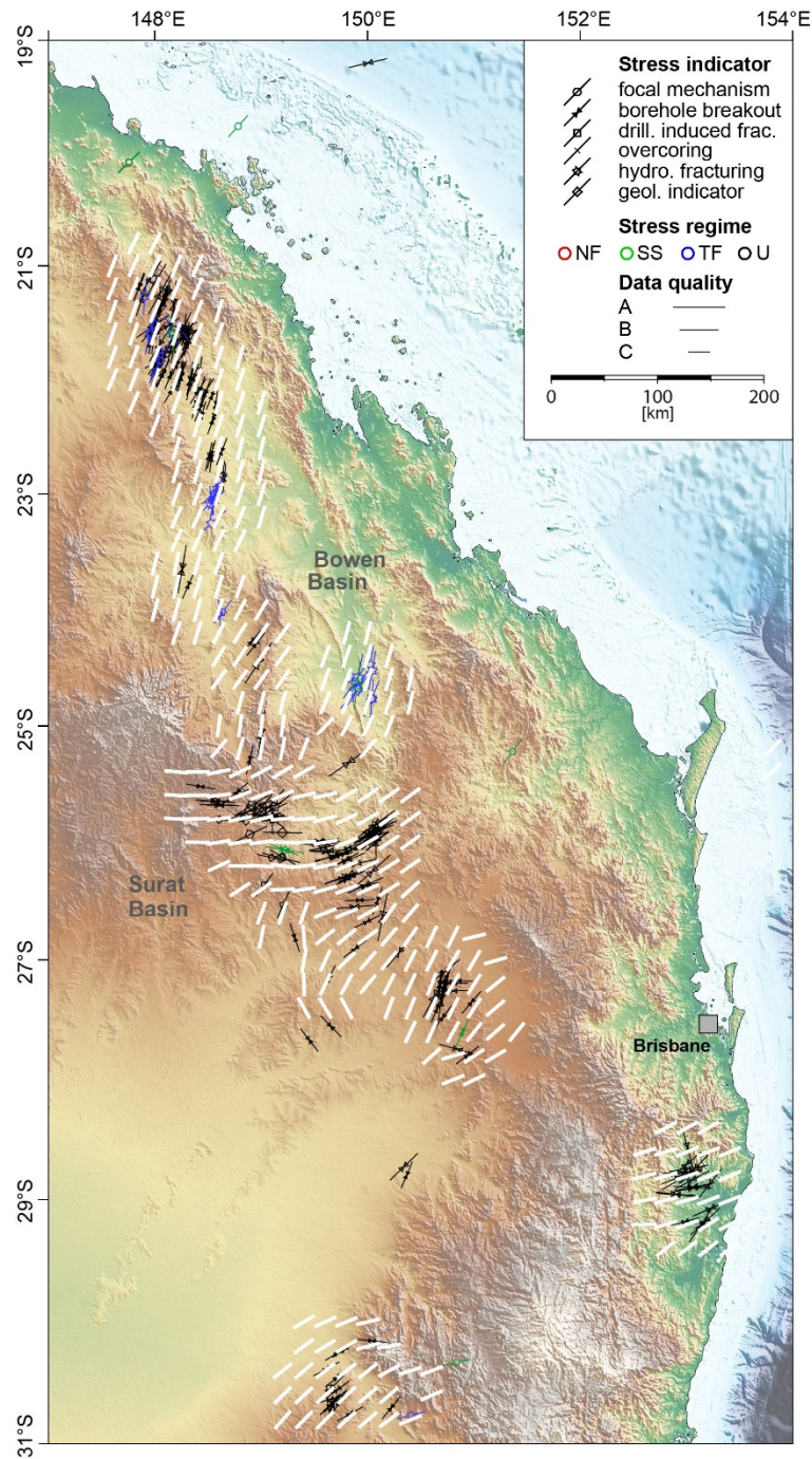
Figure 4. Stress map of north-eastern to eastern Australia. Black and coloured lines indicate the data records of the orientation of maximum horizontal stress ( S_{Hmax} ) with A-C quality. Line length is according to data quality and their colours mark the stress regime with red for normal faulting (NF), green for strike-slip faulting (SS), blue for thrust faulting (TF), and black for unknown stress regime (U). White bars on the 0.2° grid show the dataset of the mean S_{Hmax} orientation with a search radius of 50 km.
