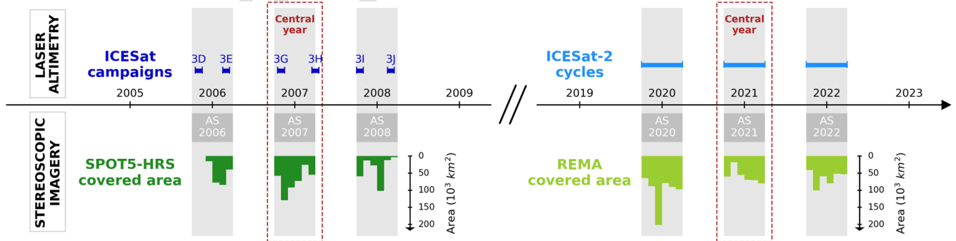
Figure 2. Timeline of the elevation datasets. For the first epoch (2006–2008), monthly SPOT5-HRS covered area is indicated in dark green and ICESat campaigns duration in dark blue. For the second epoch (2020–2022), monthly REMA covered area is indicated in light green and the ICESat-2 extracted periods in light blue. AS stands for austral summer.
