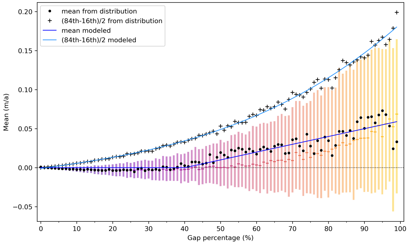
Figure A10. Relationship between the gap size in percentage of the total area and metrics of the mean difference between original and artificially voided dh/dt maps. For each gap size percent, the boxplot (median, 1 st and 3 rd quartiles) of the means is plotted in color. The mean is shown as a black dot and the robust dispersion metric (84 th percentile - 16 th percentile)/2 as a black cross. The piecewise-defined function fitted to the series of mean is shown in dark blue and the 3-degree polynomial function fitted to the robust dispersion metric series in light blue.
