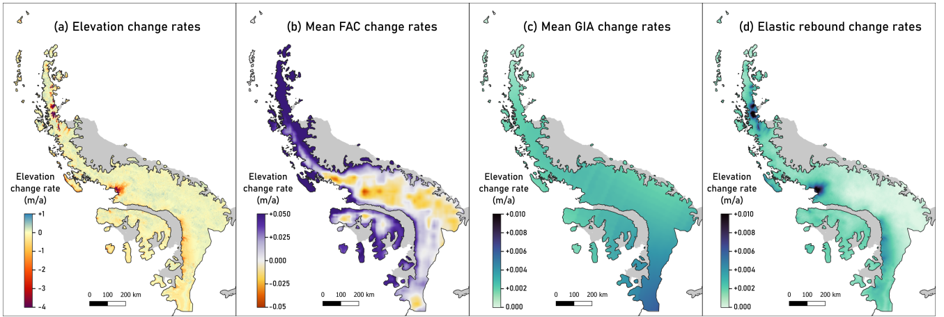
Figure 5. Complete elevation change rates map and the elevation corrections applied, 2007–2021. (a) Interpolated elevation change rates map, (b) Mean FAC changes obtained from the four firm densification models, (c) Mean GIA changes calculated from the three GIA models, (d) Solid earth elastic rebound changes computed with LoadDef. The GIA correction is the only one that is not specific to the period 2007–2021. SIL20 outlines are indicated in black and ice shelves (Pritchard et al., 2025) in grey.
