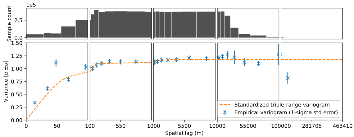
Figure A9. REMA variogram computed from the 23 REMA coincident pairs. The empirical variogram and the associated 1- \sigma standard deviation error is plotted in blue crosses. The modeled variogram based on the sum of three functions (two gaussians and a spherical) is shown in orange. The range and sill of the three ranges modeled are the following: range 1 =71 m, sill 1 = 0.71 (spherical), range 2 =217 m, sill 2 = 0.38 (gaussian) and range 3 =3 342 m, sill 3 = 0.07 (gaussian).
