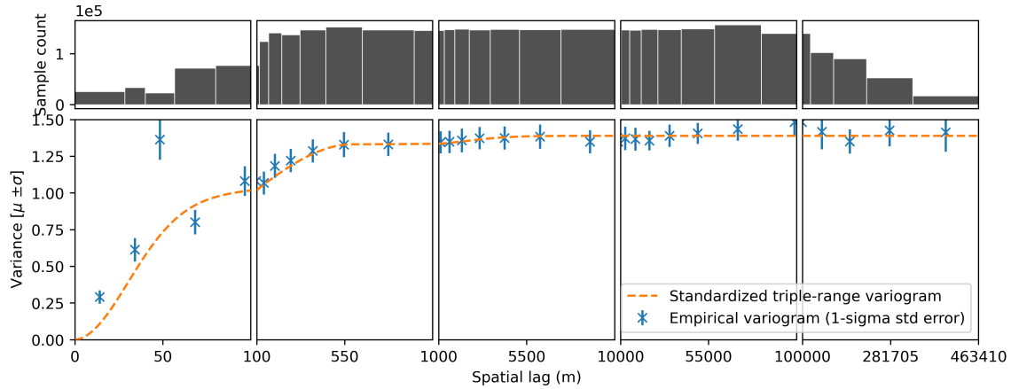
Figure A8. HRS variogram computed from the 13 HRS coincident pairs. The empirical variogram and the associated 1- \sigma standard deviation error is plotted in blue crosses. The modeled variogram based on the sum of three functions (two gaussians and a spherical) is shown in orange. The range and sill of the three ranges modeled are the following: range 1 =86 m, sill 1 = 0.92 (spherical), range 2 =596 m, sill 2 = 0.41 (gaussian) and range 3 =6 523 m, sill 3 = 0.06 (gaussian).
