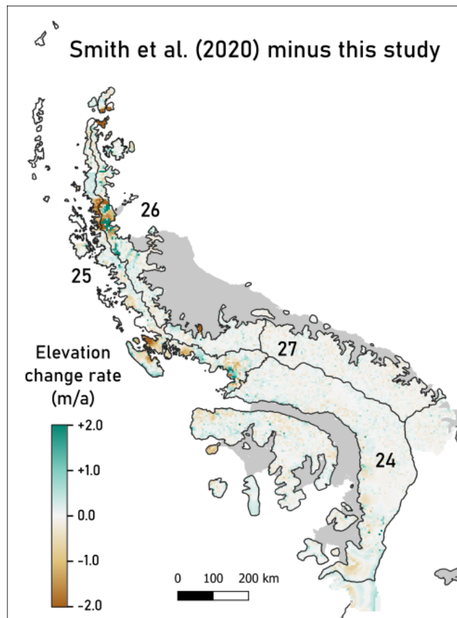
Figure A12. Elevation change rate difference between the elevation change map from Smith et al. (2020) and the one from this study. The ZWA12 outlines are plotted in black and the numbers correspond to the associated subregion number (24 to 27). The RGI outlines are plotted in black.
