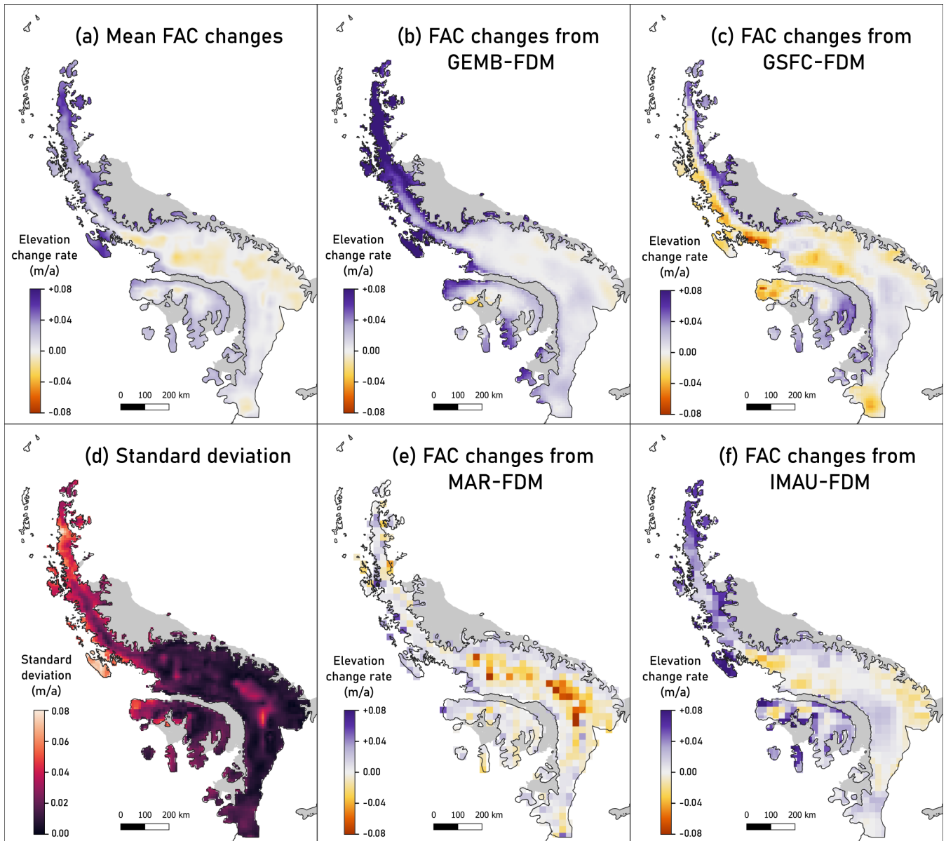
Figure A6. FAC elevation change rates from firn densification models (2007–2021). The mean FAC elevation change rate is shown on the (a), the standard deviation on (d) and the FAC elevation change rates coming from the different FDMs are plotted on (b), (c), (e) and (f).
