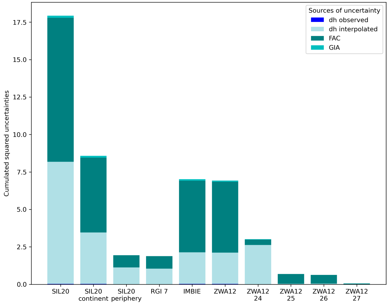
Figure A13. Contributions of sources of uncertainty for the main regions of the AP. For each outline, the different sources of uncertainties are plotted as a cumulative barplot.
