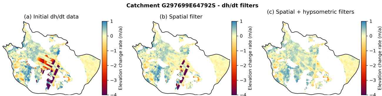
Figure A5. Effects of dh/dt filters on an example catchment. (a) Initial dh/dt data, (b) dh/dt data after spatial filtering, (c) dh/dt data after spatial and hypsometric filters.
