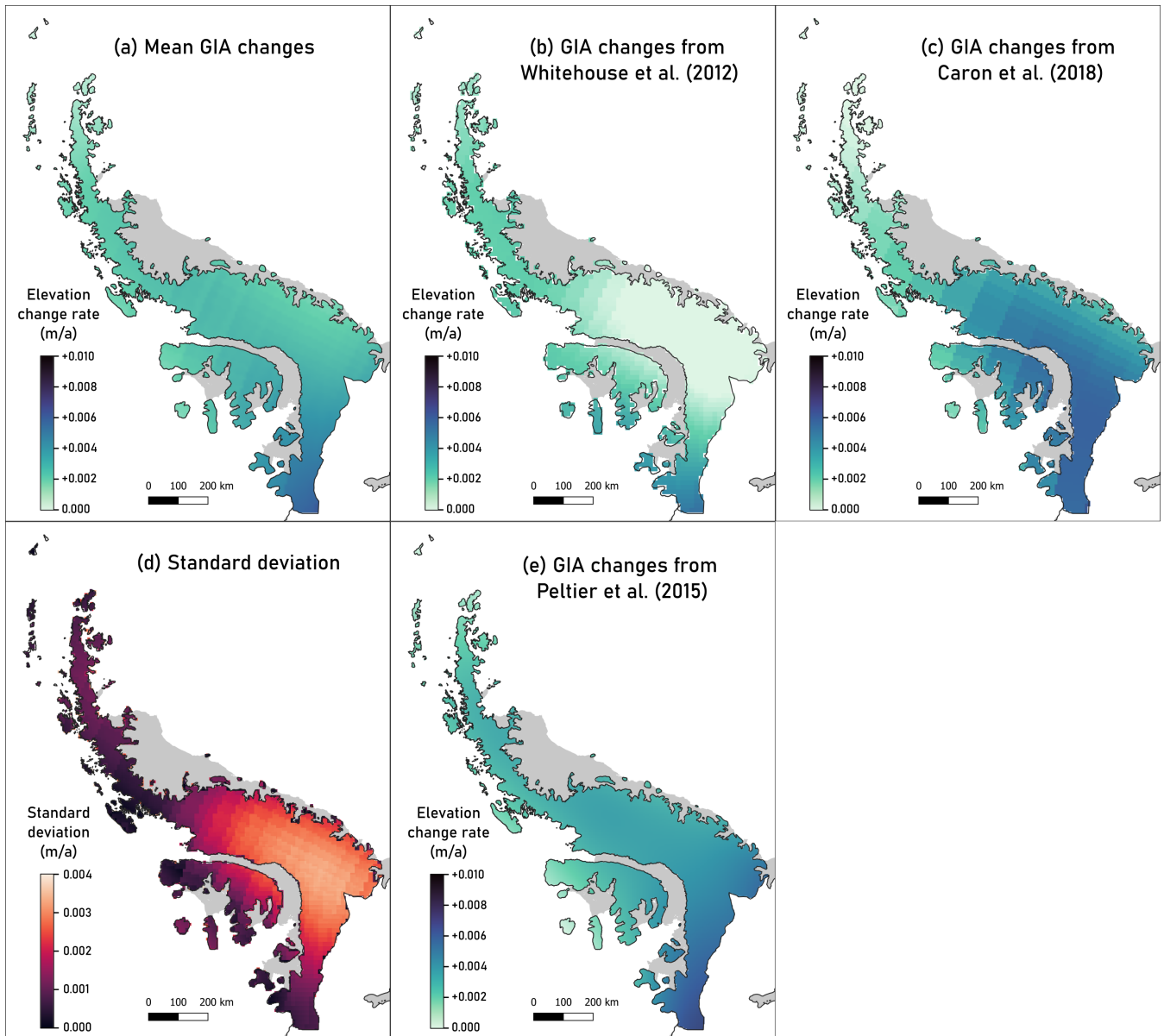
Figure A7. Elevation change rates from GIA models (2007–2021). The mean GIA elevation change rate is shown on (a), the standard deviation on (d) and the elevation change rates coming from the different models are plotted on (b), (c) and (e).
