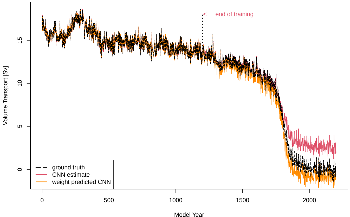
Figure 3. As Fig. 1, but with a sub-optimal example of child model performance. Still, the predicted child model (orange) outperforms the parent model (red) beyond the EOT threshold in the RMSE sense.
