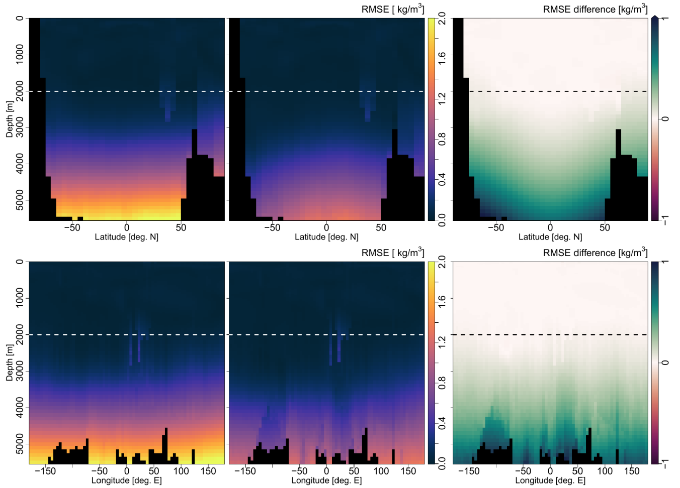
Figure 5. Depth-dependent zonally-averaged* (upper panels) and meridionally averaged* (lower panels) RMSE of NN-based sea water density estimation after training above the dashed line only. Left panels: Performance of the parent model. Middle panels: Performance of weight-predicted child model. Right panels: RMSE differences (parent minus child; the green color represents improvements by the child model). *: In giving every global output location equal weight, these averages represent a data-centered view and do not follow oceanographic standards.
