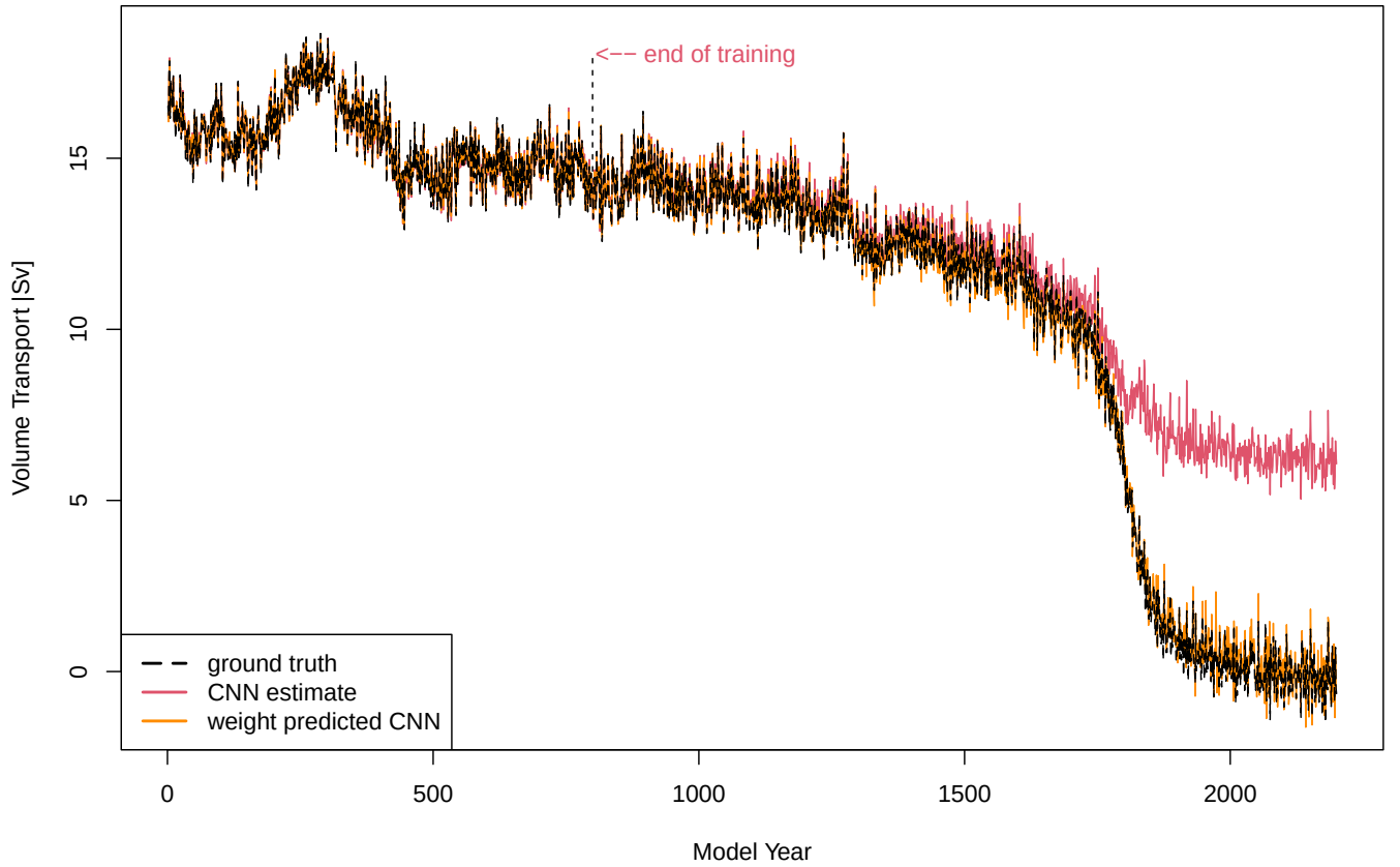
Figure 1. AMOC strength and an example of good performance of the weight-prediction method. Black Line: AMOC overturning decay and tipping, i.e., the target ground truth values. Red Line: Output of parent model trained until the dashed end of training (EOT) line. Orange Line: Output of weight-predicted child model. Online learning and subsequent fitting of EOF-to-weight relations used only data before the dashed EOT line.
