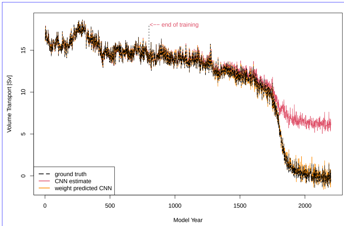
Figure 1. AMOC strength and an example of good performance of the weight-prediction method. Black Line: AMOC overturning decay and tipping, i.e., the target ground truth values. Red Line: Output of parent model trained until the dashed end of training (EOT) line. Orange Line: Output of weight-predicted child model. Online learning and subsequent fitting of EOF-to-weight relations used only data before the dashed EOT line.
