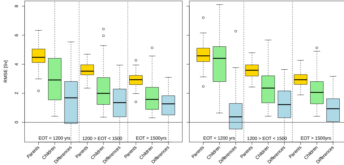
Figure 4. Impact of EOT on the RMSE of a fixed target-application range (1800yrs,2000yrs]. Polynomials of order 1 (left panel) and order 2 (right panel) where were fitted to the leading 4 principal components of the input variable (i.e., the meridional velocity maps). Yellow Boxes: RMSE of unperturbed-parent models. Green Boxes: RMSE of weight-predicted-child models. Blue Boxes: Pairwise RMSE differences (i.e., unperturbed "parent" model minus corresponding weight-predicted "child" model). Positive values represent improvements due to the presented weight-prediction approach. Each box bases-is based on 100 parents/children/pairs.
