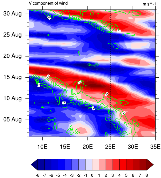
Figure X: Longitude - time (Hovmöller) diagram of 700 hPa meridional wind (shaded, m.s -1 ) and relative vorticity (contours, 10 -5 s -1 ) averaged over the Saharan band (16°N - 24°N) during August 2024. Dashed vertical lines delimit the core study domain (13°E - 25°E).
