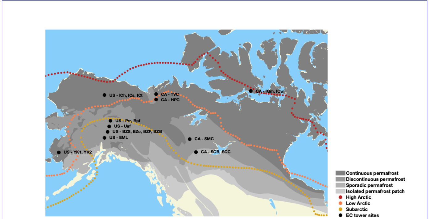
Figure 1. Locations of the 20 eddy covariance (EC) towers providing measurements of net ecosystem CO 2 exchange ( NEE_{EC} ), NEE-derived gross primary production ( GPP_{EC} ) and ecosystem respiration ( ER_{EC} ) from April 2015 to December 2022. The High Arctic, Low Arctic and Subarctic zones were delineated following the Conservation of Arctic Flora and Fauna (CAFF) working group of the Arctic Council, using Moderate Resolution Imaging Spectroradiometer (MODIS) and Landsat imagery (Potapov et al., 2008). The permafrost extent is estimated in percent areal coverage (Brown et al., 2002): continuous (>90-100% areal extent), discontinuous (>50-90%), sporadic (10-50%) and isolated patches (<10%). Due to overlapping, a single color dot may represent up to four EC towers on the map. Information for each EC tower is listed in Table 1. The figure was inspired by Madelon et al. (2025) and Mavrovic et al. (2023a).
