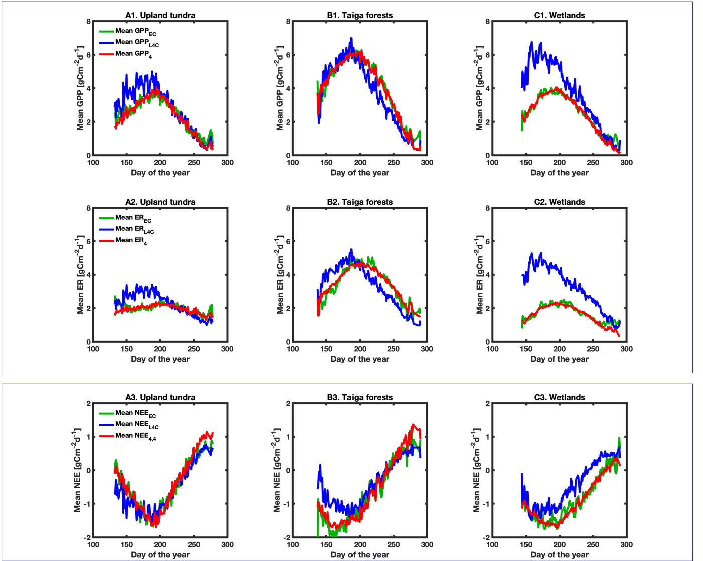
Figure B3. Mean seasonal cycle of daily averaged gross primary production (GPP), ecosystem respiration (ER), and net ecosystem CO 2 exchange (NEE) across eddy covariance tower sites for upland tundra, taiga forests, and wetlands. GPP EC , ER EC , and NEE EC denote eddy covariance data. GPP L4C , ER L4C , and NEE L4C represent outputs from the original L4C model, whereas GPP 4 , ER 4 , and NEE 4,4 (i.e., ER 4 – GPP 4 ) correspond to outputs from the Arctic–Subarctic adapted formulations using test case 4 for both GPP and ER (Sections 3 and 4.1). The data shown represent the growing season after applying the filtering criteria described in Section 4.2.
