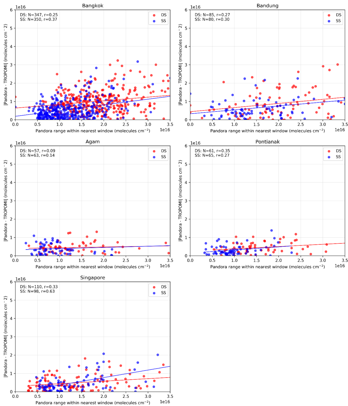
525 Figure 12. Relationship between absolute TROPOMI–Pandora HCHO bias and short-timescale Pandora variability within nearest-time matching at five Southeast Asian stations. The x-axis represents the range of Pandora HCHO columns observed within the collocation window as a proxy for local temporal heterogeneity, while the y-axis shows the magnitude of the satellite–ground bias. Red and blue markers denote direct-sun (DS) and sky-scan (SS) retrieval geometries, respectively. Linear regression lines and corresponding correlation coefficients are shown for each retrieval mode.
