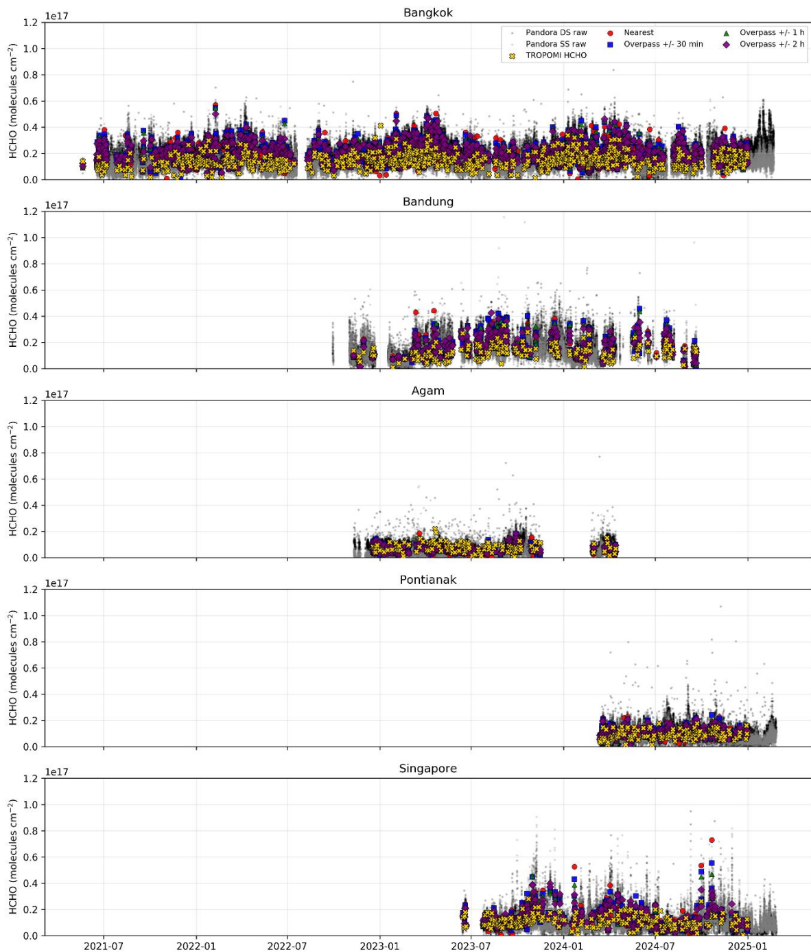
515 Figure 10. Time series of Pandora HCHO column measurements (DS and SS) and temporally collocated TROPOMI observations at five Southeast Asian stations. TROPOMI-Pandora data are shown for four collocation approaches: nearest-time matching and overpass-centred averaging windows of \pm 30 min, \pm 1 h, and \pm 2 h.
