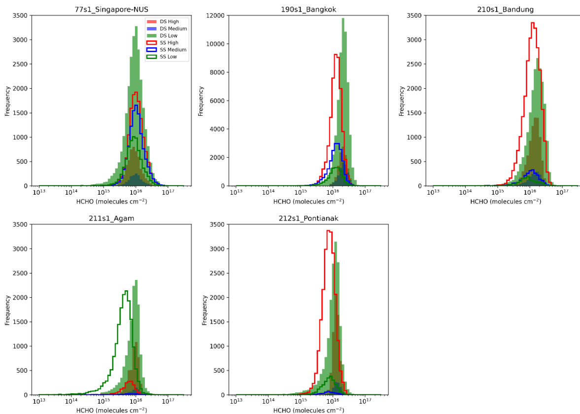
435 Figure 6. Frequency distributions of filtered HCHO vertical column densities (molecules \text{cm}^{-2} ) for direct-sun (DS; shaded histograms) and sky-scan (SS; solid line histograms) observations across five stations. Each panel corresponds to a station, with HCHO data grouped by quality flag: high quality (red; QF = 0, 10), medium quality (blue; QF = 1, 11), and low quality (green; QF = 2, 12). The x-axis is shown on a logarithmic scale to capture the wide dynamic range of HCHO values. The y-axis 440 represents the frequency of observations, with consistent limits applied across stations except for Bangkok, which has a higher observation count.
