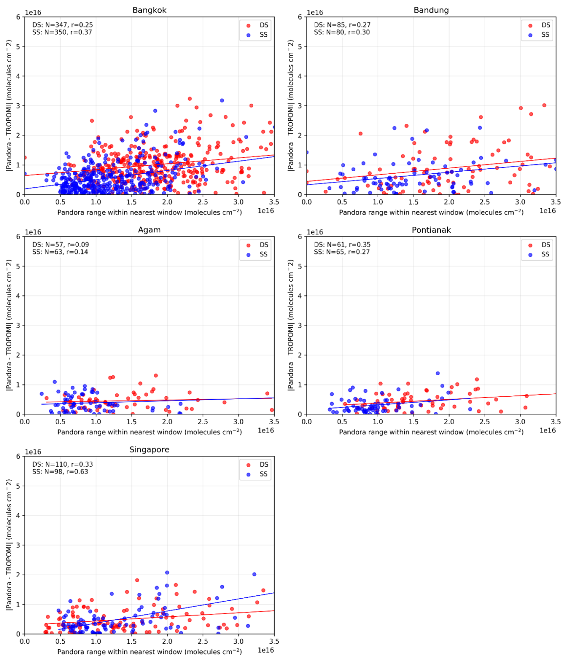
535 Figure 12. Relationship between absolute TROPOMI–Pandora HCHO bias and short-timescale Pandora variability within nearest-time matching at five Southeast Asian stations. The x-axis represents the range of Pandora HCHO columns observed within the collocation window as a proxy for local temporal heterogeneity, while the y-axis shows the magnitude of the satellite–ground bias. Red and blue markers denote direct-sun (DS) and sky-scan (SS) retrieval geometries, respectively. Linear regression lines and corresponding correlation coefficients are shown for each retrieval mode.
