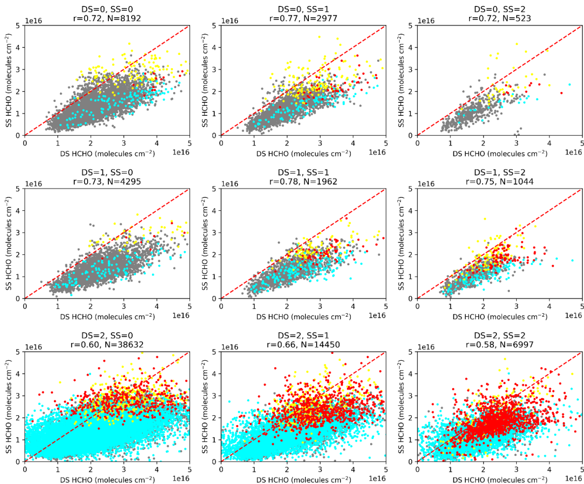
370 Figure 3. Nine-panel plot of correlation between contemporaneous Pandora HCHO column amounts: direct-sun (DS) vs sky-scan (SS) for each quality category, following the Rawat et al. (2025, AMT) QC method at Bangkok station. Panels are organized by DS and SS quality categories (0 = high, 1 = medium, 2 = low). Each panel shows the scatter of DS vs SS HCHO (molecules cm -2 ), with points color-coded by uncertainty thresholds: gray = both below cutoff, cyan = DS above cutoff, yellow = SS above cutoff, red = both above cutoff. The red dashed line represents the 1:1 relationship, and the correlation coefficient (r) and number of matched observations (N) are indicated in each panel.
