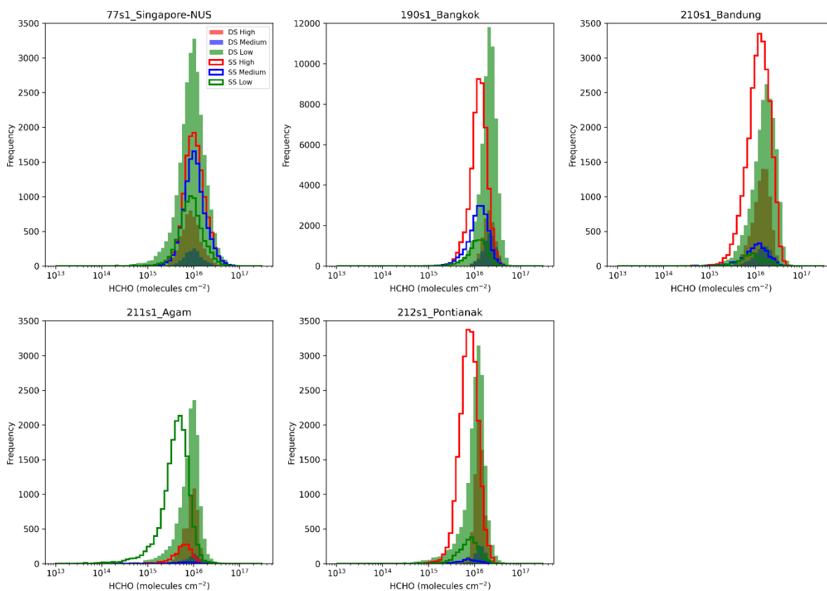
Figure 6. Frequency distributions of filtered HCHO vertical column densities (molecules \text{cm}^{-2} ) for direct-sun (DS; shaded histograms) and sky-scan (SS; solid line histograms) observations across five stations. Each panel corresponds to a station, with HCHO data grouped by quality flag: high quality (red; QF = 0, 10), medium quality (blue; QF = 1, 11), and low quality (green; QF = 2, 12). The x-axis is shown on a logarithmic scale to capture the wide dynamic range of HCHO values. The y-axis represents the frequency of observations, with consistent limits applied across stations except for Bangkok, which has a higher observation count.
