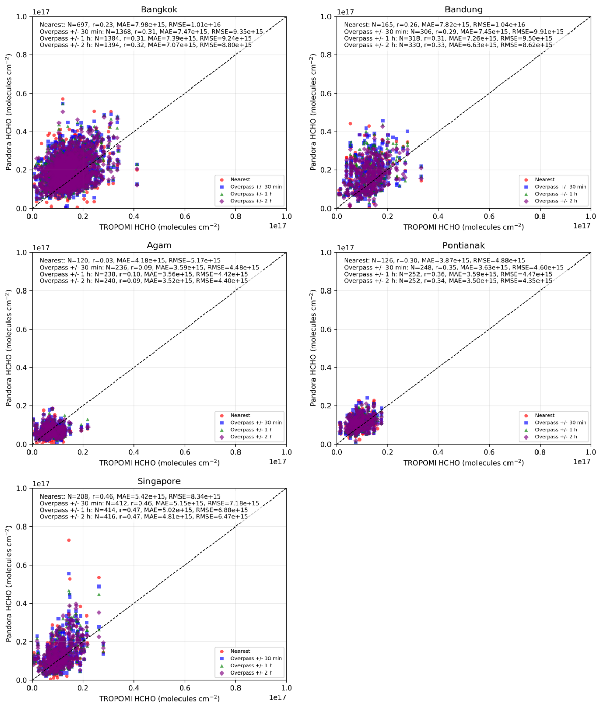
530 Figure 11. Scatter plots comparing Pandora and TROPOMI HCHO column retrievals for different temporal collocation strategies. Each panel corresponds to a measurement station and includes the 1:1 reference line. Reported statistics include sample size (N), mean absolute error (MAE), root-mean-square error (RMSE), and Pearson correlation coefficient (r).
