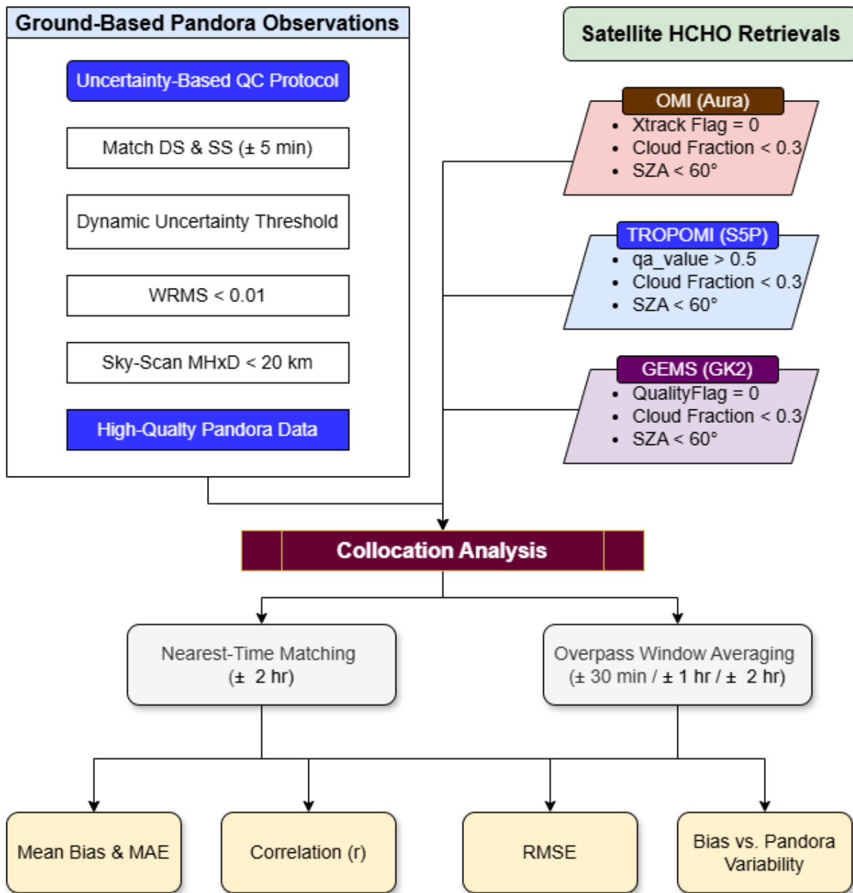
260 Figure 2. Flowchart illustrating the satellite–Pandora HCHO validation framework applied in this study. The methodology includes uncertainty-based quality control of Pandora observations following Rawat et al. (2025) , standard quality screening of OMI, TROPOMI and GEMS retrievals, temporal collocation using multiple overpass windows, and statistical evaluation of bias, error metrics, and representativeness effects in tropical environments.
