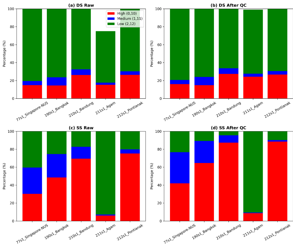
430 Figure 5. Percentage distribution of quality flags (QF) for Pandora HCHO observations at five Southeast Asian stations (Singapore, Bangkok, Bandung, Agam, and Pontianak). The stacked bar charts show the relative contributions of high- quality (QF = 0, 10), medium-quality (QF = 1, 11), and low-quality (QF = 2, 12) retrievals for both direct-sun (DS) and sky- scan (SS) measurements, before and after quality control (QC). Each panel represents a different dataset: (a) DS before QC, 435 (b) DS after QC, (c) SS before QC, and (d) SS after QC. Percentages are calculated relative to the total number of observations for each station.
