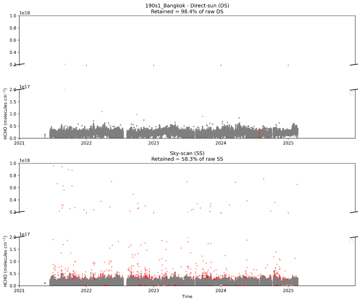
390 Figure 4. Time series of Pandora HCHO column amounts for direct-sun (DS) and sky-scan (SS) measurements following the Rawat et al. (2025, AMT) QC method at the Pandora Bangkok station. The upper panels show DS HCHO, and the lower panels show SS HCHO. Removed data points failing quality control (QC) are highlighted in red, while retained measurements are shown in gray. Broken y-axes are used to display both low and high concentration ranges. The percentage of removed points due to QC is indicated in the DS panel titles.
