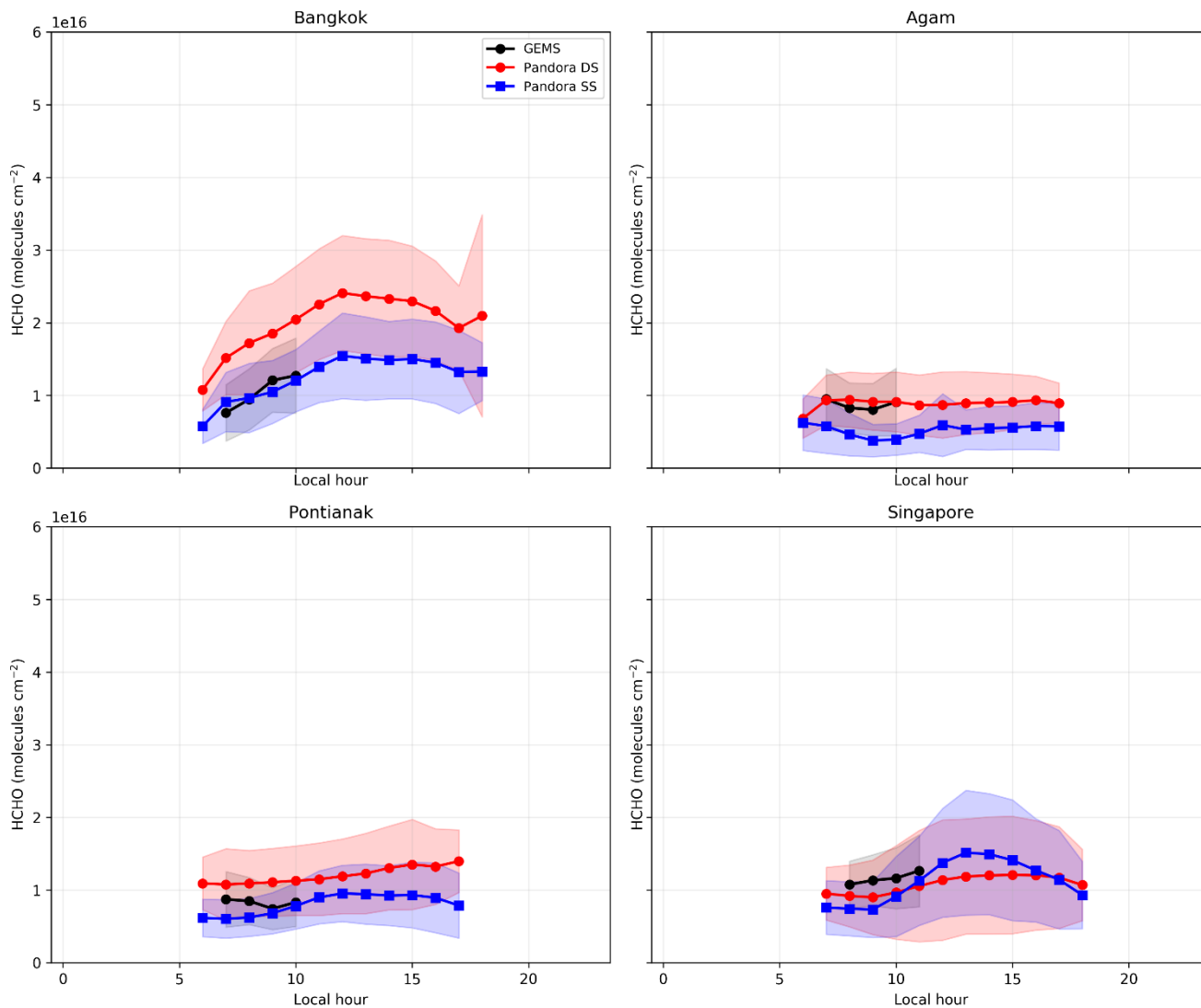
605 Figure 17. Diurnal composite of HCHO column concentrations from GEMS and Pandora observations at four Southeast Asian stations. GEMS observations are compared with Pandora direct-sun (DS) and sky-scan (SS) retrievals, averaged into local time bins to illustrate the daytime evolution of HCHO.
