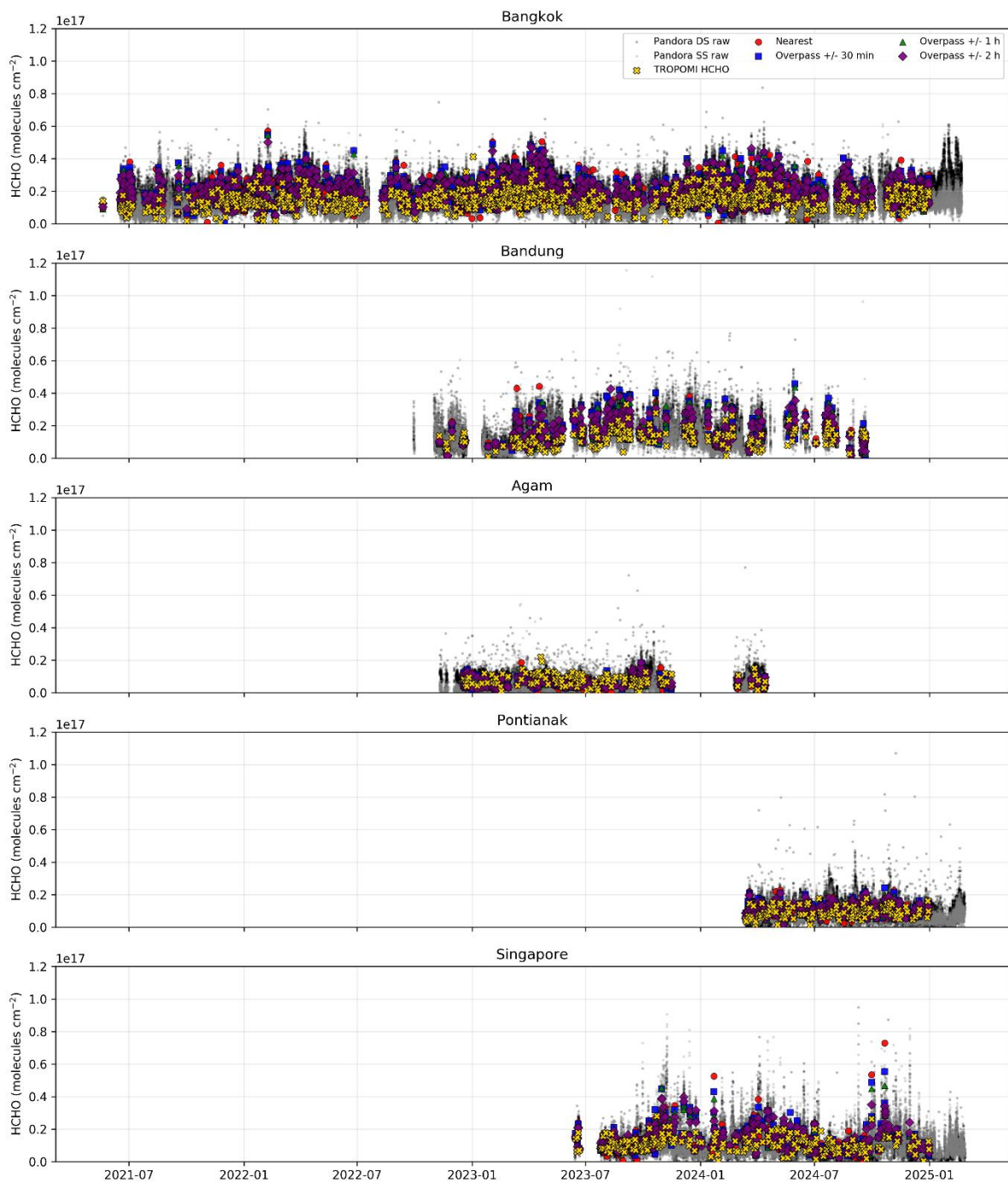
525 Figure 10. Time series of Pandora HCHO column measurements (DS and SS) and temporally collocated TROPOMI observations at five Southeast Asian stations. TROPOMI-Pandora data are shown for four collocation approaches: nearest-time matching and overpass-centred averaging windows of \pm 30 min, \pm 1 h, and \pm 2 h.
