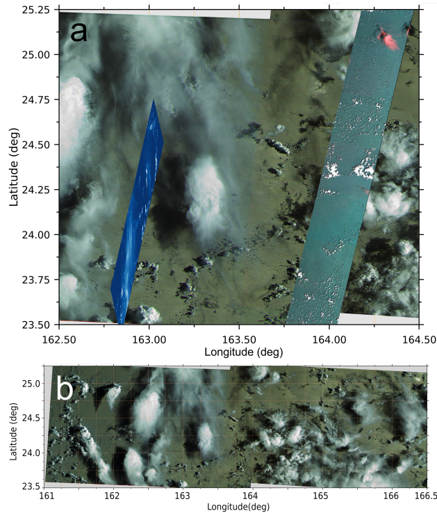
Figure 19. Map from two JANUS hyperspectral sequences superposing at around longitude 163.50^\circ . Images were built from red, blue and green filters, but the color is altered by the sun glint conditions of the observations. (a) Central region with PRISMA and EnMAP data. PRISMA data is shown in blue. EnMAP data is shown in color with RGB channels coming from observations at 940, 890 and 540 nm respectively. Red features in this image correspond to high thin clouds. (b) Full map showing the sun glint effects associated with the variation of color of the ocean over the images.
