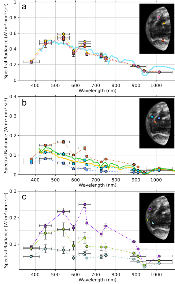
Figure 22. JANUS broadband spectra of various locations on the Earth. (a) Bright cloud systems. (b) Ocean. (c) Spectra over the Arabic peninsula, central Africa and Madagascar. Colored lines in (a) and (b) are EnMAP spectra of clouds and ocean shown previously. Insets show images of the Earth and specific locations from where each spectrum was obtained using colored circles. Spectra and images in this figure have been corrected from basic geometric effects using a Lambert correction. JANUS spectra was obtained from selected regions using a radius of 2 pixel in the Lambert corrected images.
