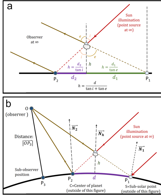
Figure 12. Geometry associated with shadow projections under extreme conditions of inclination i and e emission angles. (a) Simple geometry with no effects from parallax. (b) Geometry based on vector calculus. P_1 is the projected position of the bright cloud over the surface. P_2 is the position of the tail of the shadow observed over the planet's surface. The distance between P_1 and P_2 is the horizontal extent of the shadow. The figure has been greatly exaggerated, note that e is a small angle in the JANUS observations and that the distance \vec{OP}_3 is larger than the planetary radius and several orders of magnitude larger than the height h of the cloud sketched.
