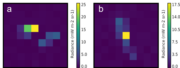
Figure 7. Linear streaks of pixels in JANUS image 0777503922_0015_01. Panel a is centered at longitude 105.20° and latitude 11.40°. Panel b is centered at longitude 104.83° and latitude 12.07°. Note the two different color scales for these two features. Pixel scale is 158 m and exposure time is 25 ms.
