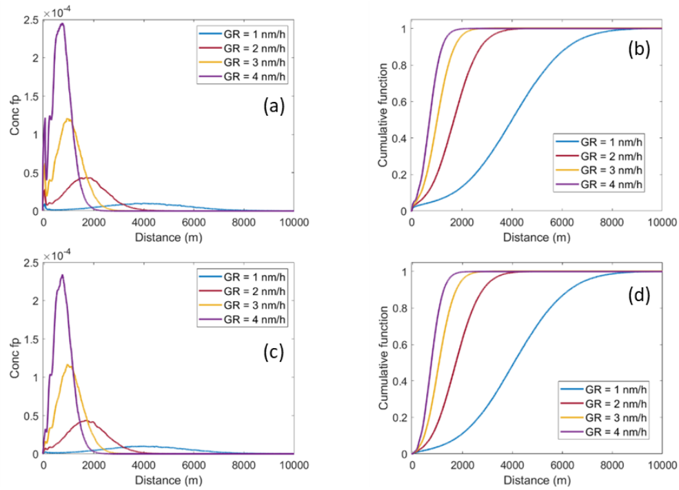
Figure 8. Source contribution functions (b,d – normalized cumulative) at 0.5 m height (a, b) and at 4 m (c, d), agricultural field. Initial aerosol distribution function is the same as for forest calculations ( d = 1.75 nm and \sigma = 0.07 nm). Moving average with the window 101 m is applied to the functions in panels (a) and (c).
