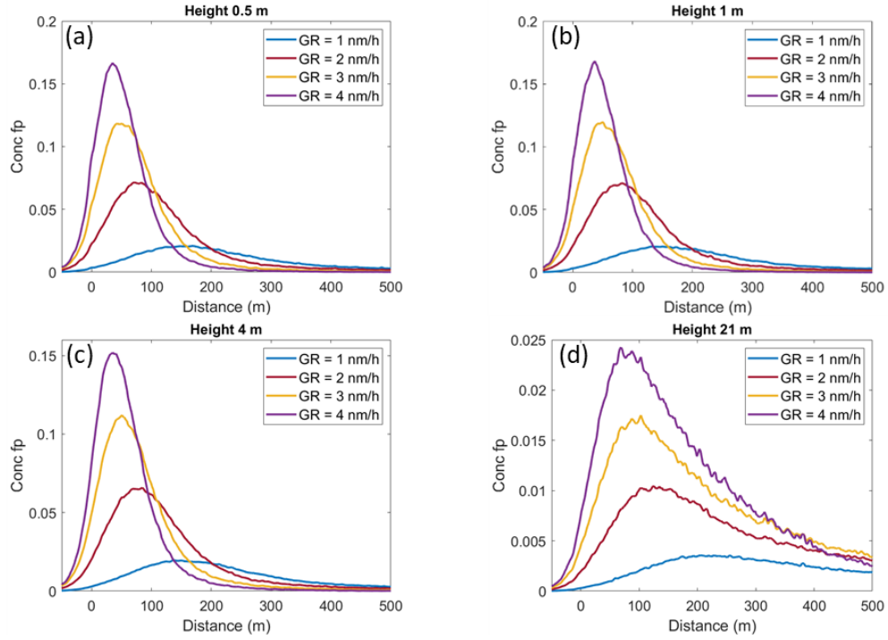
Figure 5. Source contribution areas of the local aerosol production for different measurement heights (see figures' titles) and different aerosol growth rates (different colors and figure legends). Moving average with the window of 3 m is applied to all the functions.
