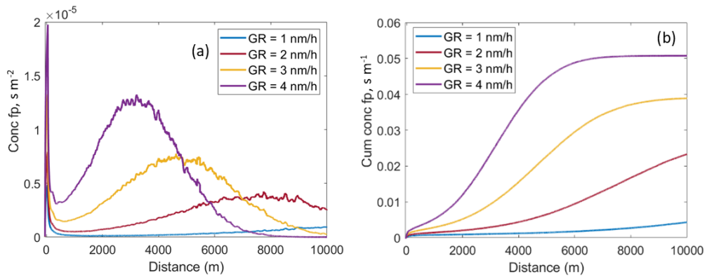
Figure 11. Source contribution functions for the initial sub 2-nm distribution with d = 1.15 nm and \sigma = 0.25 nm (Case 2, Fig. 9). Measurement height is 0.5 m. Moving average with the window 101 m is applied to the functions in the left panels. The cumulative functions are not normalized because functions at the lowest GR do not saturate at 10 km.
