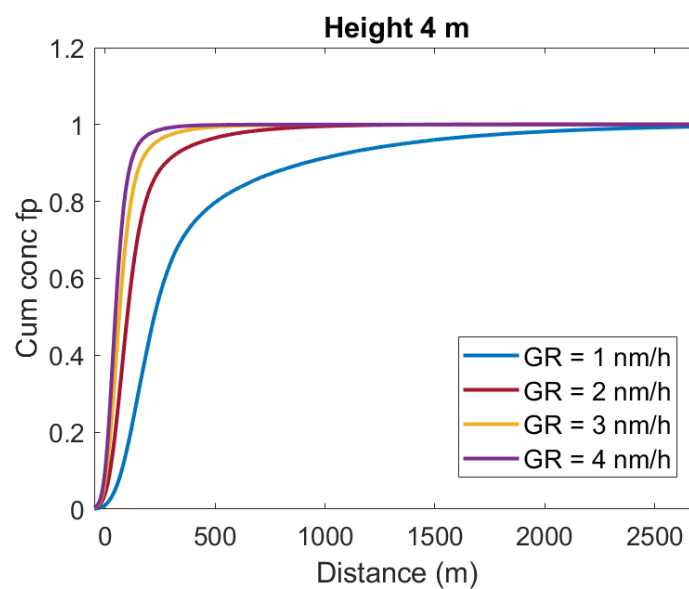
Figure 6. Example of the normalized cumulative source contribution function for the measurement height of 4 m. The 80% cumulative footprint for aerosol production of 2-2.3 nm diameter particles is the distance where the cumulative function is equal to 0.8 ( Table 1).
