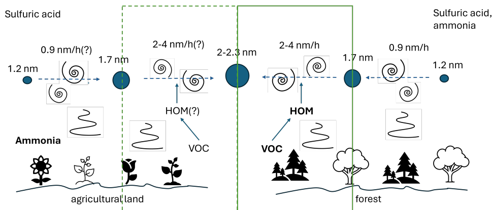
Figure 1. Schematic illustration of the processes contributing to formation and growth of 2.0-2.3 nm ions over agricultural land and forest. Agricultural land emits ammonia and volatile organic compounds (VOC), while forest emits mainly VOC. VOC in agricultural field and in the forest can differ. VOC are oxidized to form highly oxygenated molecules (HOM), i.e. condensable organic vapors. Sulfuric acid is assumed to be formed from sulfur compounds present as background in the atmosphere, ammonia is also present as background. Vortices show turbulence in the atmosphere. 1.2 nm is a representative diameter where sub-2-nm ion distribution typically has a maximum. Aerosol clustering and stabilization (up to 1.7 nm) as well as activation (1.7-2.3 nm) phases in the forest are sketched in accordance with Kulmala et al (2013), respective growth rates of \sim 0.9 nm/h and \sim 2-4 nm/h are estimated from observations. Green rectangular zone focuses on the processes accounted in the calculation of a source contribution function in this study. Note that for forest, the sketched process of aerosol formation and growth can occur both above and under canopy.
