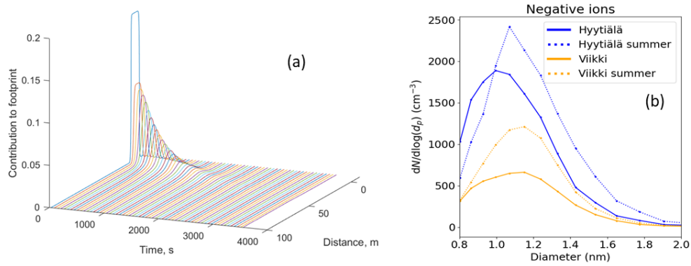
Figure 3. (a) Example of contributions to the inert scalar concentration footprint as a function of the parcel travel time, t , (cf Fig. 2) and distance, x , to the measurement source f(x,t) calculated for the measurements below forest canopy; (b) median annual and summer sub-2 nm aerosol particle number-size distributions (SMEAR II forest site and SMEAR-Agri agricultural site).
