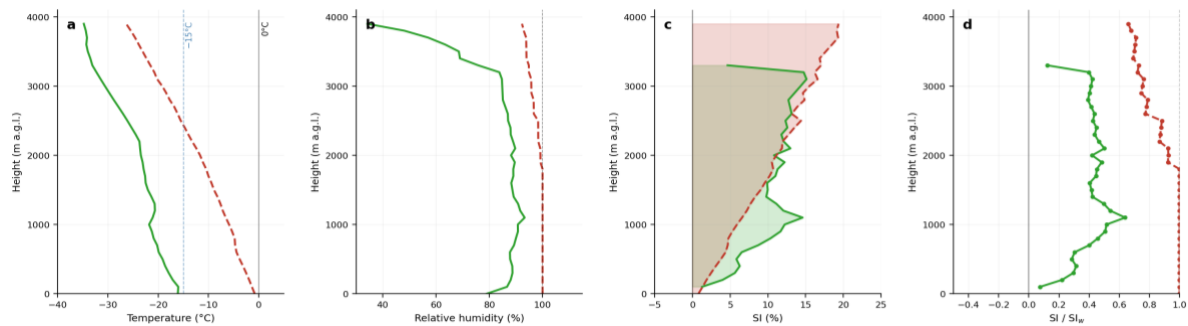
Figure 10. Height-resolved profiles of T, RH, SI and \text{SI}/\text{SI}_w during Dumont d'Urville precipitation events on 29 May 2019 (green curves) and 23 Jul 2019 (red curves).
