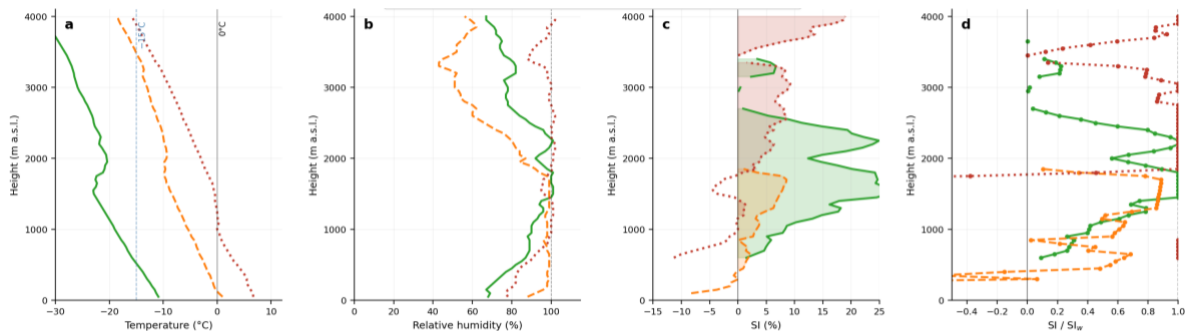
663 Figure 8 Height-resolved profiles of T, RH, SI and SI/SI w during Ny-Ålesund precipitation events on 12 Feb 2016 (green 664 curves), 31 Aug 2014 (orange curves) and 19 Jul 2014 (red curves).
