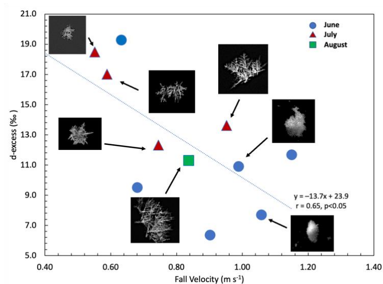
430 Figure 2. d-excess versus average fall velocity measured with a MASC at Summit. Selected photographs of particles for 431 which the fall velocity was measured are also shown. The dotted line shows the best fit linear regression line.
