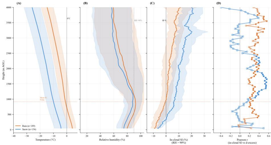
Figure 7. Mean vertical profiles of (A) air temperature, (B) relative humidity, (C) in-cloud SI, and (D) Pearson correlation coefficient ( r ) for the linear regression of d-excess and height-resolved mean in-cloud SI from radiosonde measurements at Ny-Ålesund during rain (red) or snow (blue) precipitation days. Open symbols in D indicate p > 0.05 (statistically insignificant) and solid symbols indicate p < 0.05 (statistically significant).
