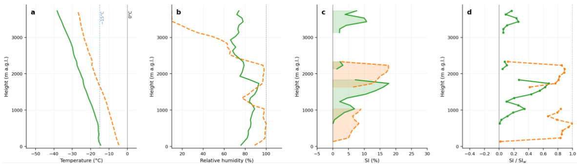
Figure 5 Height-resolved profiles of T , RH , SI and SI/SI_w during Summit precipitation events on 2 Jul 2012 (green curves) and 26 Jul 2013 (orange curves).
