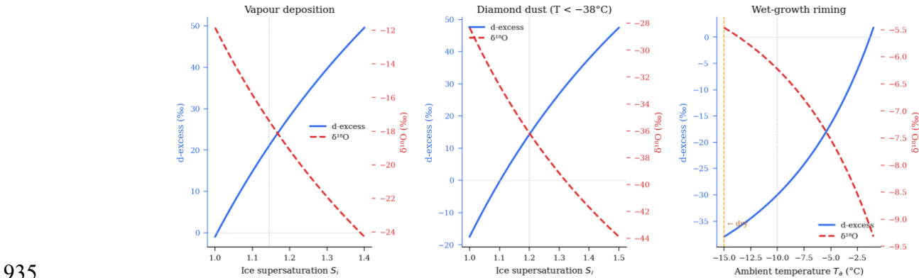
Figure 12. Dominant parameters and their effect on the calculated d-excess of end-members. Input parameters were: for vapor deposition ( \delta^{18}\text{O}_v = -30\text{‰} , d_v = 10\text{‰} , T_c = -20^\circ\text{C} , f=0.997 ); for diamond dust ( \delta^{18}\text{O}_v = -50\text{‰} , d_v = 15\text{‰} , T_c = -40^\circ\text{C} ); for wet-growth riming ( \delta^{18}\text{O}_v = -20\text{‰} , d_v = 10\text{‰} , \text{LWC} = 0.5 \text{ g m}^{-3} , E = 0.8 , R = 3 \text{ mm} , V = 1 \text{ m s}^{-1} ).
