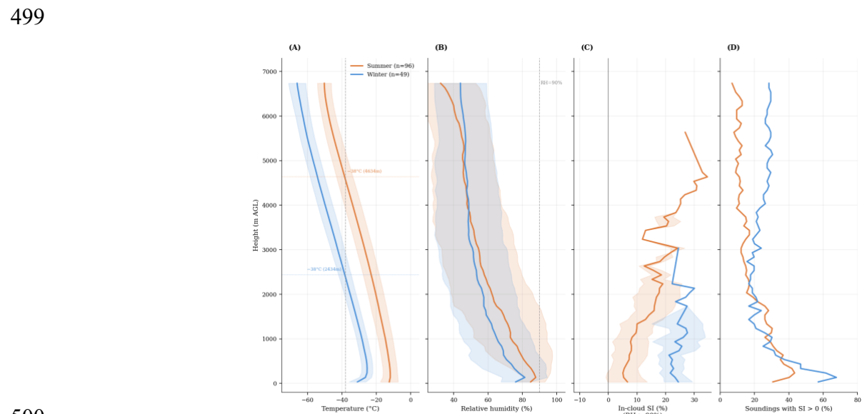
500 501 Figure 4. Mean vertical profiles of air temperature (A), relative humidity (B), and in-cloud ice supersaturation (C) from 502 radiosonde measurements at Summit during summer (brown) and winter (blue). Panel D shows percentage of soundings 503 when \text{SI} > 0 for at least one radiosonde level. 504
