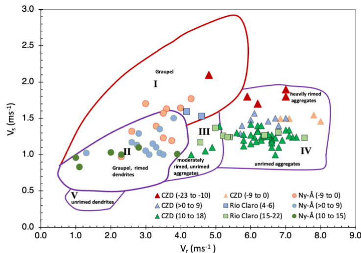
Figure 11. Classification of rimed and unrimed particles based on fall velocities above ( V_s ) and below ( V_r ) the melting layer. The boundaries for Categories I to V are as proposed by Weiss et al. (1977): I. Graupel (lump and conical, hexagonal) and graupel-like snow; II. Graupel, graupel-like snow, moderately to densely rimed dendrites, assemblages of dendrites, and columns, aggregates of unrimed side planes, bullets and columns; III. Moderately rimed to unrimed aggregates of dendrites; unrimed aggregates of bullets, side planes and columns; IV. Moderately rimed to unrimed aggregates and radiating assemblages of dendrites; V. Unrimed dendrites. Graupel with varying density plots in multiple fields (highest density in category I). For categories II, III and IV, unrimed particles plot towards the bottom and densely rimed towards the top. Also plotted are the rainfall samples from Cazadero (CZD; triangles), Rio Claro (squares) and Ny-Ålesund (circles). Symbol colors correspond to the range of d-excess values (red < -10%, pink = -9 to 0%; blue = > 0 to +9%; green > +10%) as shown in the legend.
