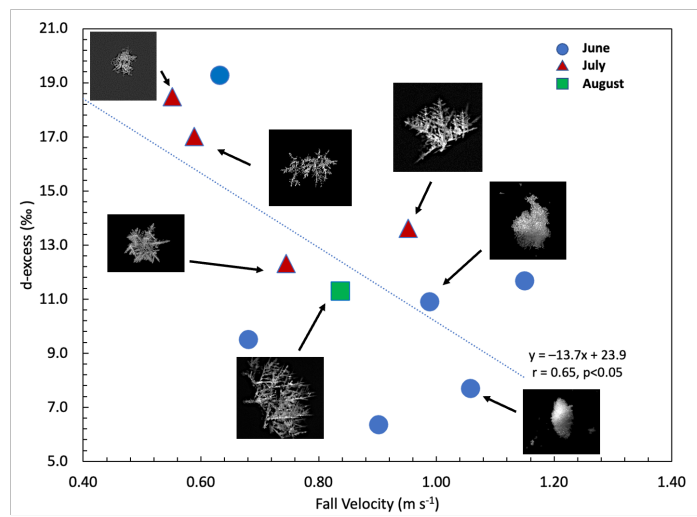
Figure 2. d-excess versus MASC-measured average fall velocity at Summit. Selected photographs of particles for which corresponding to the measured fall velocity was measured are also shown. The dotted blue line is the best fit linear regression line.
