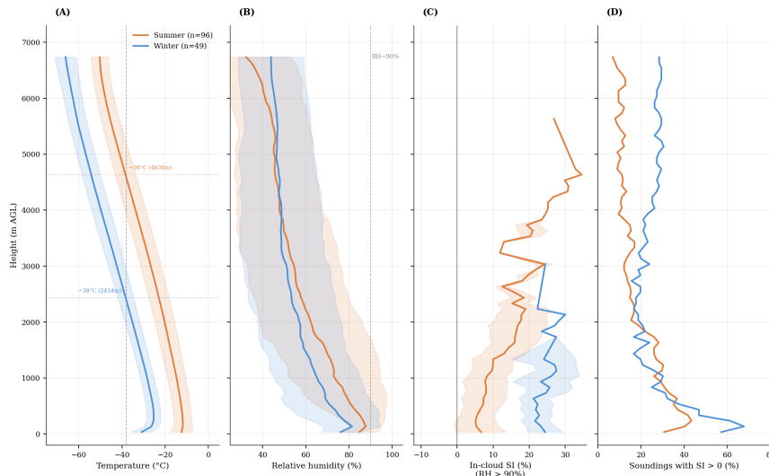
Figure 4. Mean vertical profiles of air temperature (A), relative humidity (B), and in-cloud ice supersaturation (C) from radiosonde measurements at Summit during summer (brown) and winter (blue). Panel D shows percentage of soundings when \text{SI} > 0 for at least one radiosonde level.
