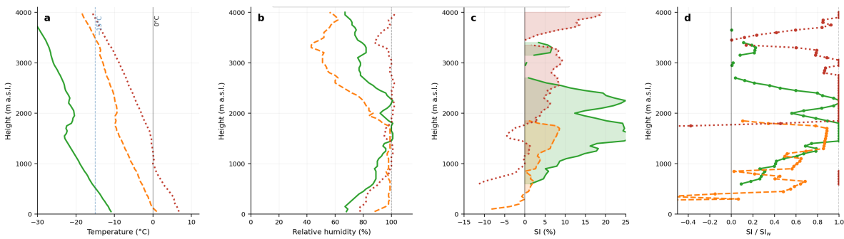
Figure 8 Height-resolved profiles of T, RH, SI and SI/SI w during Ny-Ålesund precipitation events on 12 Feb 2016 (green curves; d-excess/MDV = +34.5‰ / 0.71 m s -1 ), 31 Aug 2014 (orange curves; +13.9‰ / 0.99 m s -1 ) and 19 Jul 2014 (red curves; -4.6‰ / 1.31 m s -1 ).
