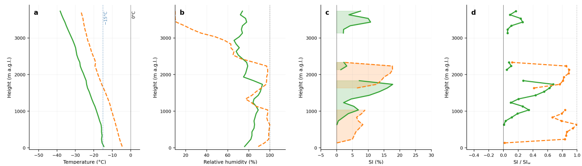
Figure 5 Height-resolved profiles of T , \text{RH} , \text{SI} and \text{SI}/\text{SI}_w during Summit precipitation events on 2 Jul 2012 (green curves; \text{d-excess}/\text{MDV} = +23.6\text{‰} / 0.89 \text{ m s}^{-1} ) and 26 Jul 2013 (orange curves; +14.7\text{‰} / 1.14 \text{ m s}^{-1} ).
