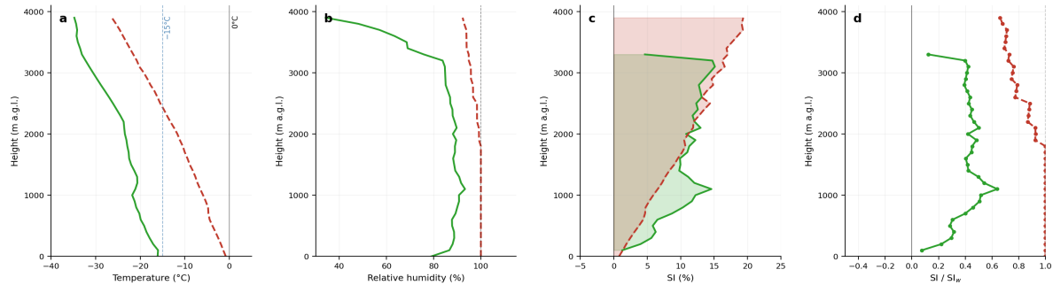
Figure 10. Height-resolved profiles of T, RH, SI and SI/SI w during Dumont d'Urville precipitation events on 29 May 2019 (green-curves; d-excess/MDV = +14.0‰ / 1.05 m s -1 ) and 23 Jul 2019 (red-curves; +4.8‰ / 1.54 m s -1 ).
