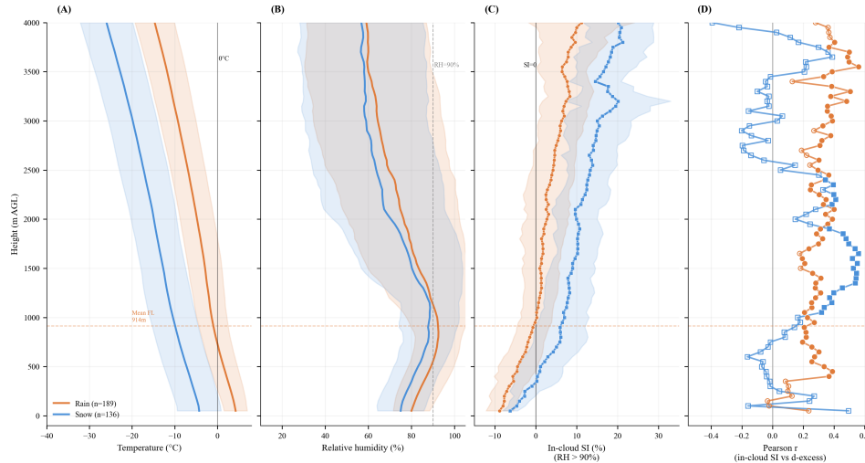
Figure 7. Mean vertical profiles of (A) air temperature, (B) relative humidity, (C) in-cloud SI, and (D) Pearson correlation coefficient ( r ) for the linear regression of d-excess and height-resolved mean in-cloud SI from radiosonde measurements at Ny-Ålesund during rain (red) or snow (blue) precipitation days. Open symbols in D indicate p > 0.05 (statistically insignificant) and solid symbols indicate p < 0.05 (statistically significant).
