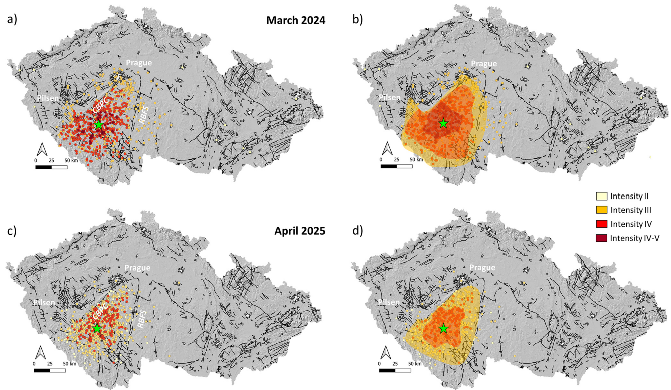
Figure 3. The Mirovice earthquakes. (a, b) The M_L 3.5 event in March 2024; (c, d) the M_L 3.1 event in April 2025. (a, c) Spatial distribution of macroseismic observations (color-coded by individual intensities) collected by IG CAS. (b, d) macroseismic intensity according to the EMS–98 scale. The epicentres are marked in green. CBPC, Central Bohemian Plutonic Complex; RBFS, Röd–Blanice Fault System.
