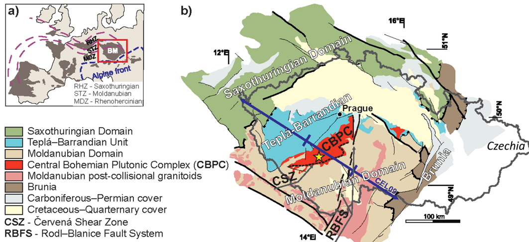
Figure 1. (a) Schematic sketch of the European Variscides with the Bohemian Massif (red box) in the eastern edge. (b) Simplified geological map of the Bohemian Massif with individual tectonic units (modified after Machek et al., 2022). The Mirovice earthquakes are marked by a yellow star; the violet line marks the CEL09 seismic profile from the CELEBRATION 2000 experiment (Hrubcová et al., 2005). The Czechia border is indicated by a grey curve. TS1
