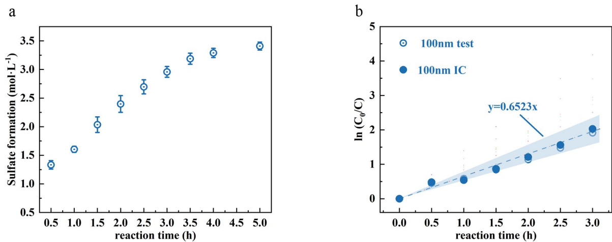
295 Figure 4. (a) Sulfate concentration and (b) \ln (C_0/C) of 100 nm NaCl droplets formed at 80 % RH as a function of reaction time.
