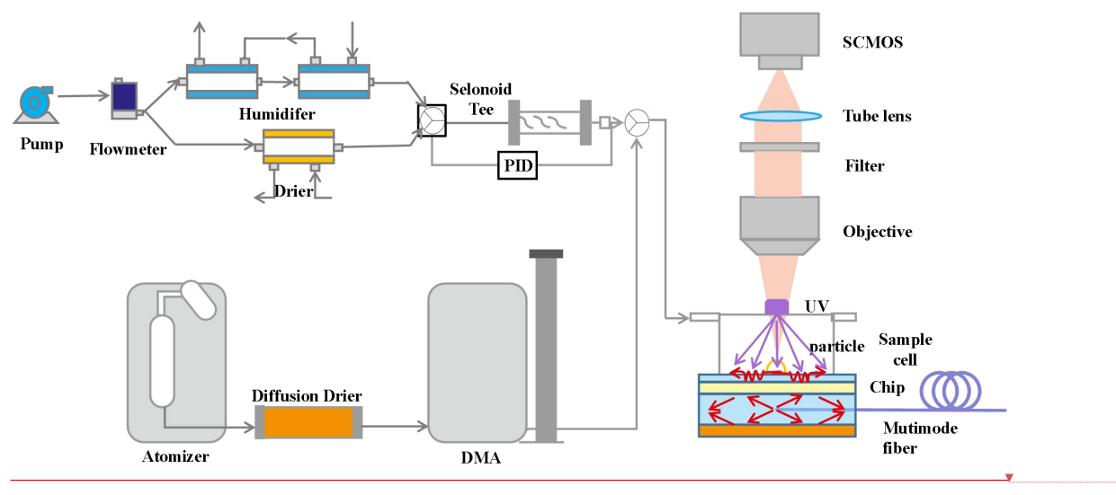
Figure 1. Schematic diagram of the system for generation, aging, and hygroscopic growth measurements based dark-field imaging for single nanoparticles.
