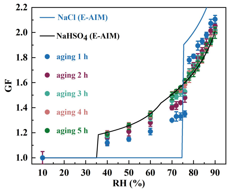
220 Figure 3. GFs of 100 nm NaCl particles after reaction times of 1 h, 2 h, 3 h, 4 h, and 5 h, together with the predicted GFs of NaCl and NaHSO 4 .
