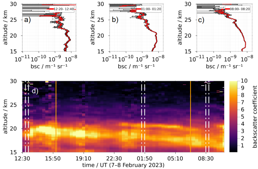
Figure 4. The BSC from a 16-hour 21-hour measurement on 7–8 February 2023, Kühlungsborn. (a), (b), (c): Mean BSC for selected time periods. (d): Temporal and dynamic evolution of the Junge layer over the entire measurement period. The vertical dash-dotted lines indicate the time intervals corresponding to measurements (a), (b), and (c). The vertical solid orange lines denote sunset (16:05 UT, 7 February 2023) and sunrise (06:47 UT, 8 February 2023), respectively.
