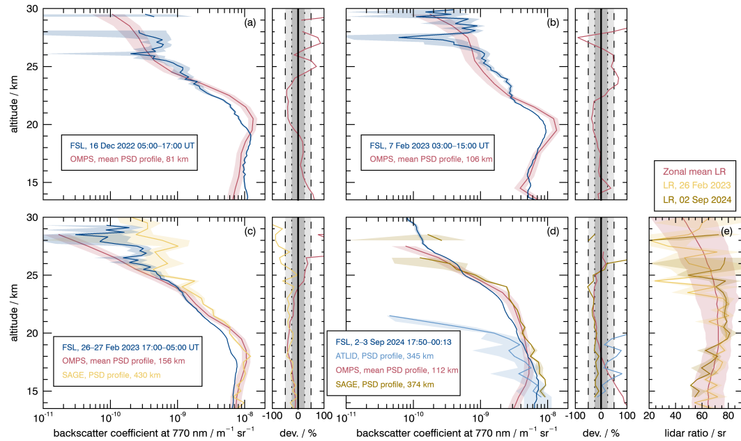
Figure 5. Comparison of the BSC from four FSL measurements (in blue) averaged over several hours with the derived BSC at 770 nm from collocated satellite measurements in (a–d). The lidar ratios (LR) used are shown in (e) in the corresponding colours. The mean spatial distance of these collocated measurements from Kühlungsborn is given in km. For OMPS-LP, the calculated BSC for a zonal lidar ratio profile averaged over the duration of the SAGE III/ISS mission (see Sec. 2.3) is shown in red. The SAGE III/ISS BSC calculated with a variable lidar ratio depending on the PSD of the measurement is shown in yellow. A mean ATLID BSC profile, converted to 770 nm, is shown in light blue. The percentage deviation of the FSL from the satellite measurements is shown on the right-hand side of each subplot. The range of a deviation of 50 % and 25 % is indicated by a dashed and dotted line, respectively.
