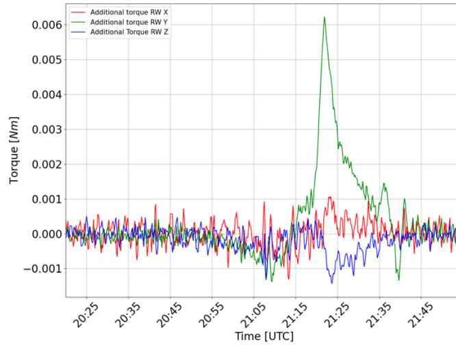
Fig. 12 Additional torques exerted by reaction wheels (RW) on the spacecraft along body fixed reference frame X (red), Y (green), Z (blue).
