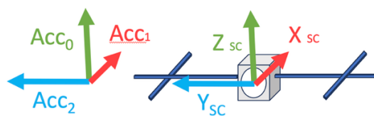
190 Fig. 2 HAA (left) and JUICE SPACECRAFT (right) reference frames
