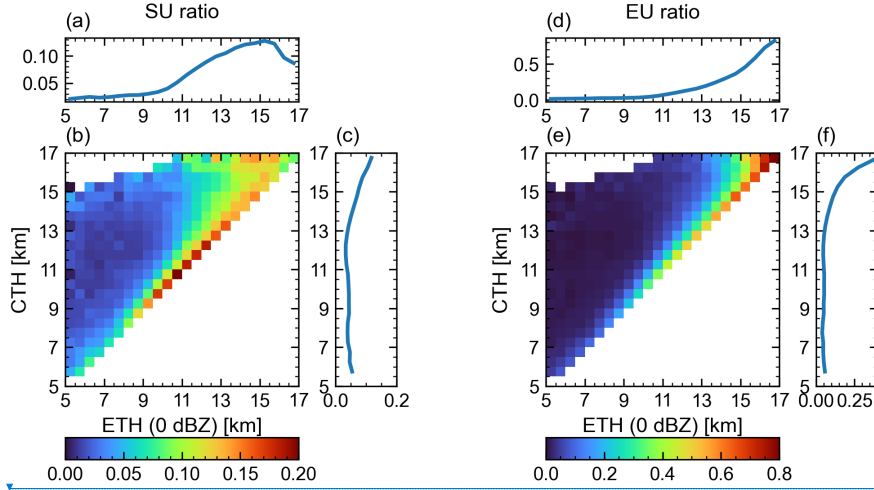
463 Figure 6: Occurrence ratios of SU columns and EU columns as functions of ETH(0) and CTH. (a–c) SU ratio and (d–f) EU ratio. 464 The SU ratio is defined as the number of non-folded columns with \text{Max}V_d > 2.0 \text{ m s}^{-1} divided by the total number of selected 465 convective columns in each bin. The EU ratio is defined as the number of folded columns divided by the same denominator. Note 466 that the SU and EU panels use different color scales. Panels (b) and (e) show two-dimensional ratios in the CTH–ETH(0) phase 467 space; marginal ratios are shown as functions of ETH(0) and CTH.
