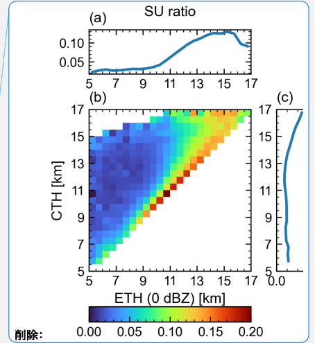
Figure 6: Occurrence ratios of SU columns and EU columns as functions of ETH(0) and CTH. (a–c) SU ratio and (d–f) EU ratio. The SU ratio is defined as the number of non-folded columns with \text{Max}V_d > 2.0 \text{ m s}^{-1} divided by the total number of selected convective columns in each bin. The EU ratio is defined as the number of folded columns divided by the same denominator. Note that the SU and EU panels use different color scales. Panels (b) and (e) show two-dimensional ratios in the CTH–ETH(0) phase space; marginal ratios are shown as functions of ETH(0) and CTH.
