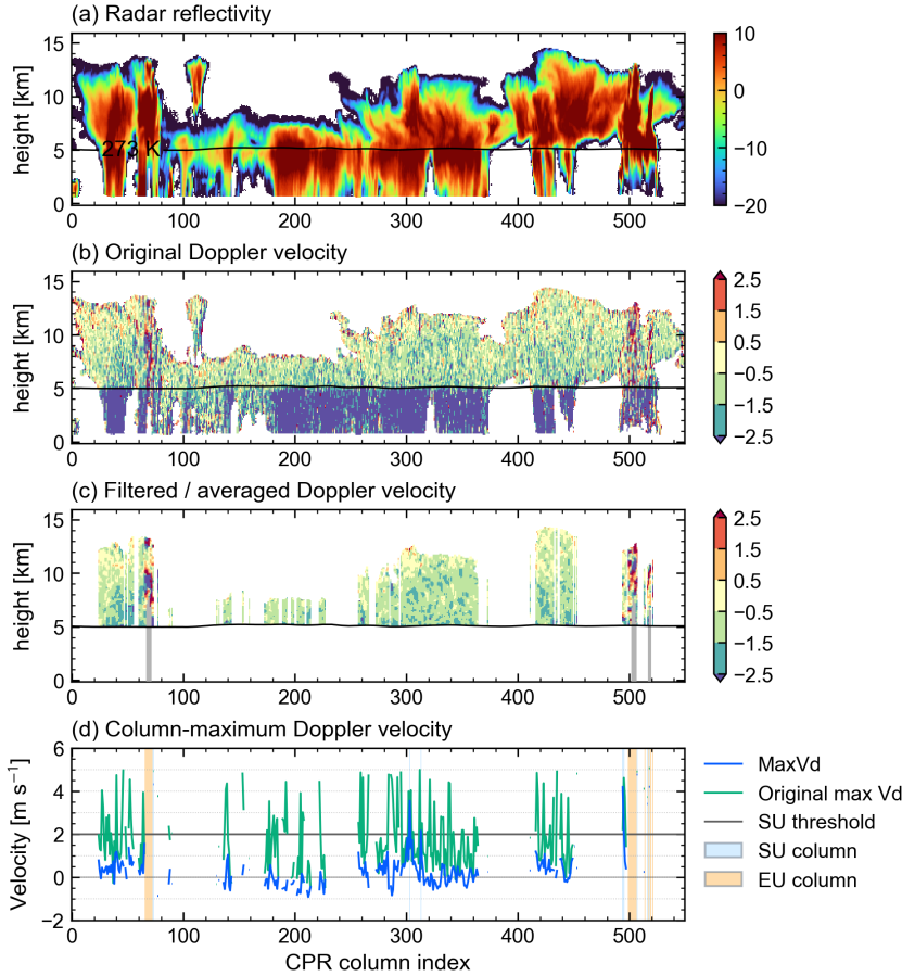
265 Figure 1: Example illustrating Doppler-velocity quality control, folding detection, and the definition of the updraft metric \text{Max}V_d 266 for an EarthCARE/CPR scene. (a) Radar reflectivity factor (Ref; dBZ). (b) Input CPR_CLP Doppler velocity ( V_d ; \text{m s}^{-1} ) after 267 applying only the cloud-mask threshold (cloud mask \geq 20 ); positive values indicate upward motion. The black line marks the 273.15 268 K isotherm. (c) V_d after applying the column-selection criteria and quality control. Gaps indicate columns or gates for which no 269 valid V_d remains after column selection and quality control. Grey shading near column indices approximately 70, 500, and 510 270 denotes gates flagged as being affected by multiple scattering. (d) Column-maximum V_d as a function of column index, computed 271 from the input field in (b) for visual comparison (“Original”; green) and from the filtered and averaged field in (c) for the 272 quantitative metric (“ \text{Max}V_d ”; blue). Light-orange shading denotes columns flagged as folded and classified as extreme-updraft 273 (EU) candidate columns. Light-blue shading denotes columns with \text{Max}V_d > 2.0 \text{ m s}^{-1} , classified as strong-updraft (SU) columns.
