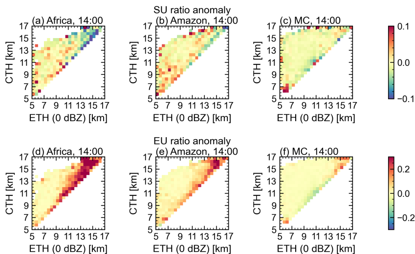
Figure 10: Deviations in Doppler-based occurrence ratios conditioned on cloud-top height (CTH) and the 0 dBZ echo-top height [ETH(0)] for early afternoon (~14:00 LT). (a–c) show deviations in the MaxV d -based SU ratio, and panels (d–f) show deviations in
