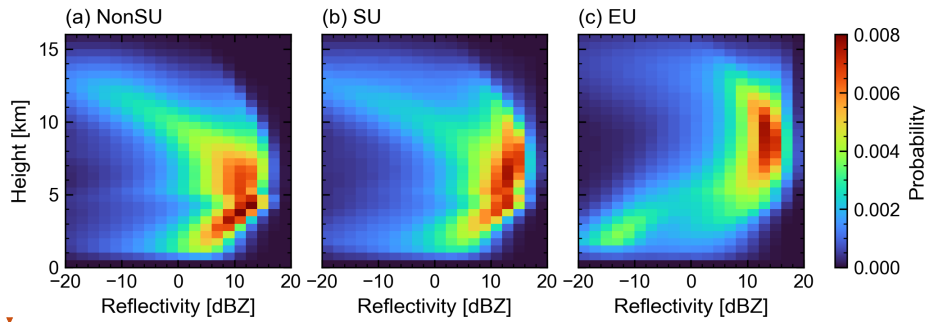
Figure 3: Normalized frequency-by-altitude diagrams (CFADs) of EarthCARE/CPR radar reflectivity (Ref; dBZ) for (a) non-strong-updraft (NonSU) columns, (b) strong-updraft (SU) columns, and (c) extreme-updraft (EU) candidate columns. Reflectivity is binned in 2 dBZ intervals, and the vertical coordinate is binned in 500 m intervals. Each panel is normalized by its total number of height-reflectivity samples such that the color indicates probability (i.e., the sum over all bins in each panel equals 1).
