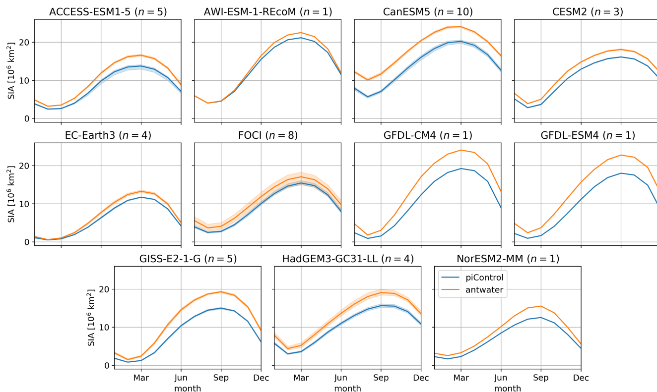
Figure 2. Ensemble-mean seasonal cycle of Antarctic sea ice area for each model. Results are computed as the total Antarctic sea ice area for each month averaged over the final 30 years of the 100 year simulations. The piControl is shown in blue and antwater is shown in orange. Shading denotes the range across ensemble members for the models with more than one ensemble member.
