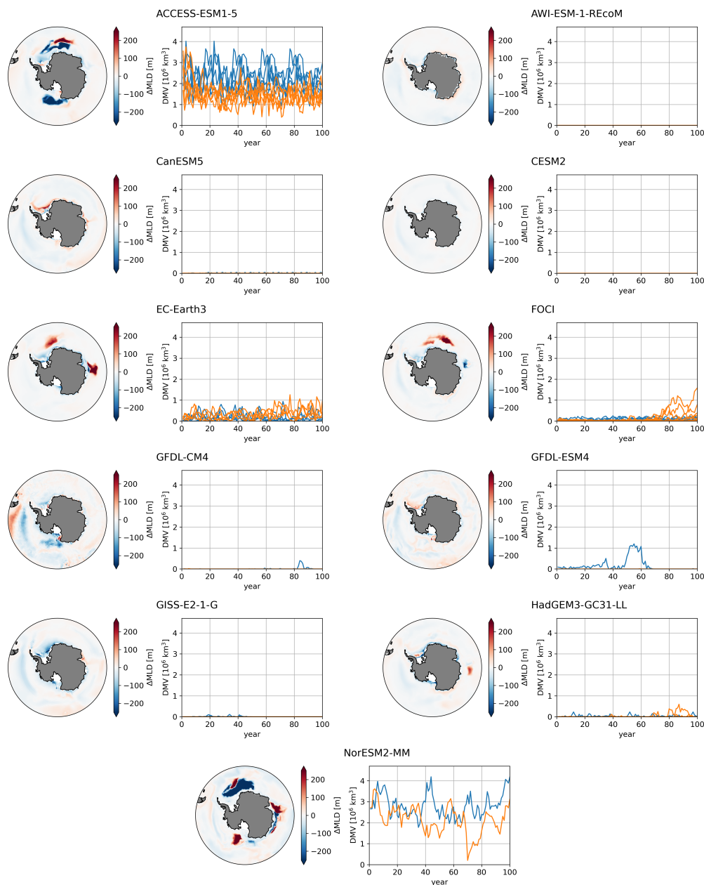
Figure 8. Annual-mean mixed-layer depth response and deep mixed volume (DMV) for the piControl (blue) and antwater (orange) experiments for each of the models. DMV is computed as the product of mixed-layer depth and grid cell area for all grid cells south of 55°S with mixed-layer depth greater than 2000 m. Mixed-layer depth response is the difference between antwater and piControl averaged over the final 30 years of 100-year simulations.
