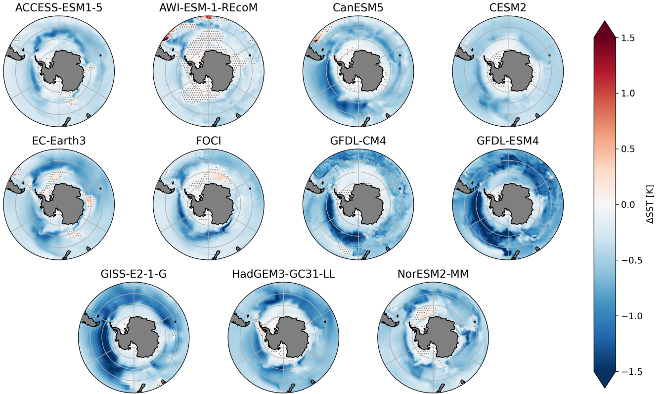
Figure 6. Ensemble-mean annual-mean sea surface temperature response for each of the models. Results are presented as the average over the last 30 years of the 100 year simulations. Stippling denotes where the response is not statistically significant at the 95% confidence level.
