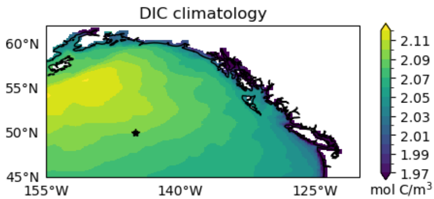
Figure S1: Climatology of DIC from the model. The star indicates the location of OSP.
