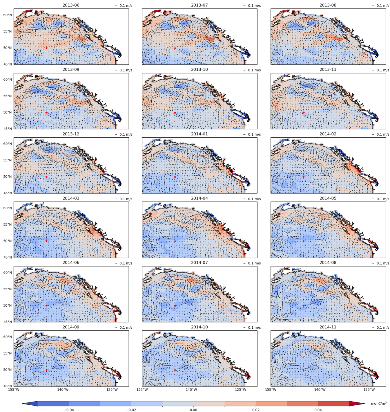
Figure S2: Surface velocity (vectors) and DIC (colored shading) anomalies relative to 2010–2017, from June 2013 to November 2014. All variables have been detrended and deseasonalized. Velocities are smoothed using a 3-month moving average.
