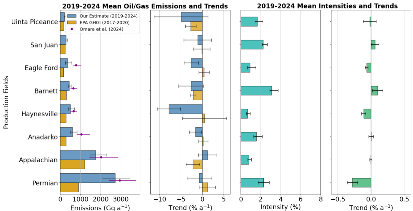
455 Figure 6: 2019-2024 mean oil/gas production, emissions, emission intensities, and trends for the top eight oil/gas production fields in CONUS. Emissions and emission intensities are from the mean of our posterior estimates, with error bars representing the ranges from the inversion ensemble (for the 2019-2024 mean panels) or the standard error on the regression slopes (for the trends). Emission estimates from Omara et al. (2024) are for 2021 emissions. Trends are calculated using OLS regression on results for individual years. Production data were derived from the Enverus prism platform (Enverus, 2025). 460 MMBBL is million barrels of oil and MMBOE is million barrels of oil equivalent. Oil/gas field boundaries are based on definitions in Omara et al. (2024).
