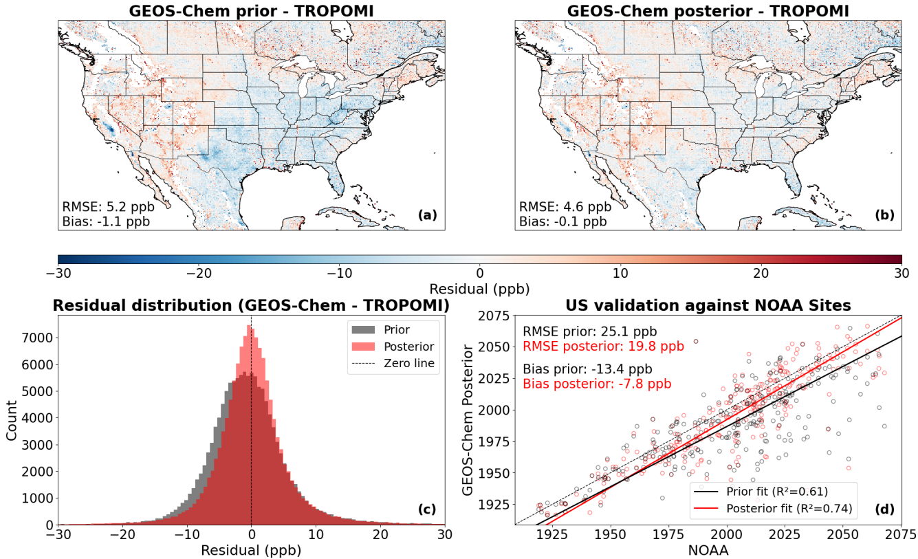
Figure 2: Evaluation of the prior and posterior emission estimates when implemented in the GEOS-Chem simulation. The top panels show the gridded annual mean residuals between GEOS-Chem and the TROPOMI observations for the (a) prior and (b) posterior simulations. Panel (c) shows the tightening of the residual distribution in the posterior estimate (red) versus the prior estimate (grey). Panel (d) shows comparison with independent NOAA site observations, where each point represents an annual afternoon mean. Root-mean-square errors (RMSE), mean biases, and reduced-major-axis regression lines are inset.
