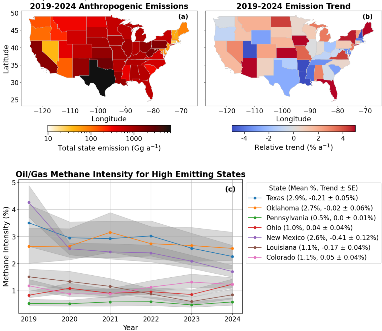
Figure 5: Mean 2019-2024 anthropogenic emissions, trends, and intensities for individual states. Panel (a) shows mean anthropogenic emissions on a log scale. Panel (b) shows the percent change per year from a linear regression of the emissions for each state. Panel (c) shows methane intensities from the oil/gas sector for the six states dominated by oil/gas emissions and Colorado. The trends and standard errors (SE) are from ordinary least squares regression of the mean intensity for each year. EIA data on individual state dry production for 2024 was unavailable at the time of writing, so we estimate dry production from marketed gas using the ratio of dry production to marketed gas in 2023.
