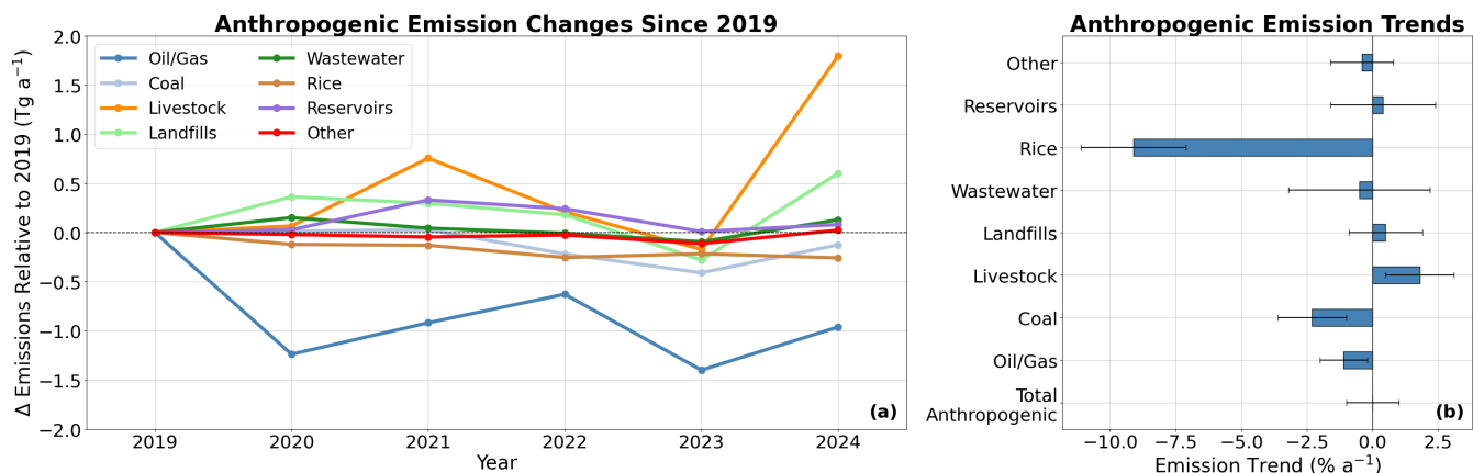
Figure 3: Changes in CONUS anthropogenic methane emissions relative to 2019 and trends by sector, 2019-2024. Values are show the change in the annual mean posterior estimates relative to 2019 from our inversion ensemble . Trends are derived from ordinary least squares regression of emissions for individual years, and error bars are the standard error.
