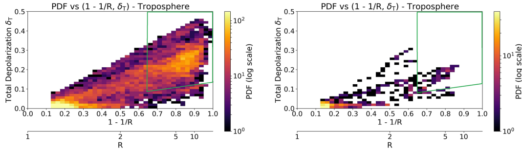
Figure 5. Normalized point-density PDF of tropospheric clouds in the (1 - 1/R) , \delta_T phase space. Left: full dataset. Right: Young-optimized subset. Cirrus follow a continuous branch with increasing depolarization and backscatter enhancement, bounded by particle-depolarization isolines. The area bounded by green lines selects the well-developed ice clouds in the upper troposphere for further analysis. The reduced number of Young-optimized profiles mainly reflects the lower signal-to-noise ratio of the tropospheric channel rather than a microphysical selection.
