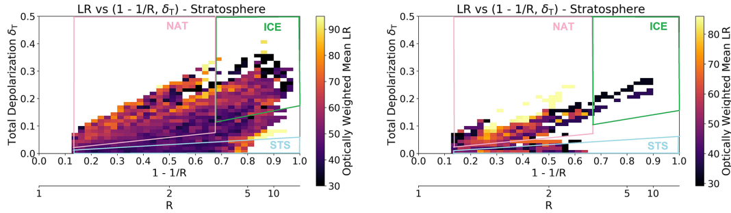
Figure 2. Optically weighted mean lidar ratio (LR) in the (1 - 1/R, \delta_T) phase space for PSC. Left: full dataset. Right: Young-optimized subset. Higher LR values are more frequently found in portions of the phase space associated with stronger backscatter enhancement and depolarization, although the relationship is not monotonic and shows substantial variability. In the Young-optimized subset most high-LR ice PSC disappear, likely because these layers do not satisfy the Young-optimization conditions.
