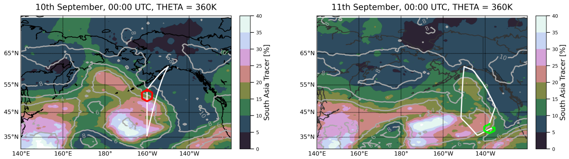
Figure 2. CLaMS South Asia tracer (= 'ECH' + 'TIB' + 'NIN' + 'IND' + 'BoB' + 'NIO', see Fig. 1) at 360K potential temperature. PV values are shown as gray isolines. Left: Initial flight on 10 September 2023 UTC. A large filament with increased mixing ratios of South Asian air is projected to be in range of HALO research flights from the base in Anchorage. The first hexagon is located towards the end of the flight near the edge of the filament and is marked in red. Right: Follow-up flight on 11 September 2023 UTC. The filament 'rolls over' southeastwards. The second hexagon (marked in green) is located inside the outflow from the first hexagon (see Fig. 3) at that time.
