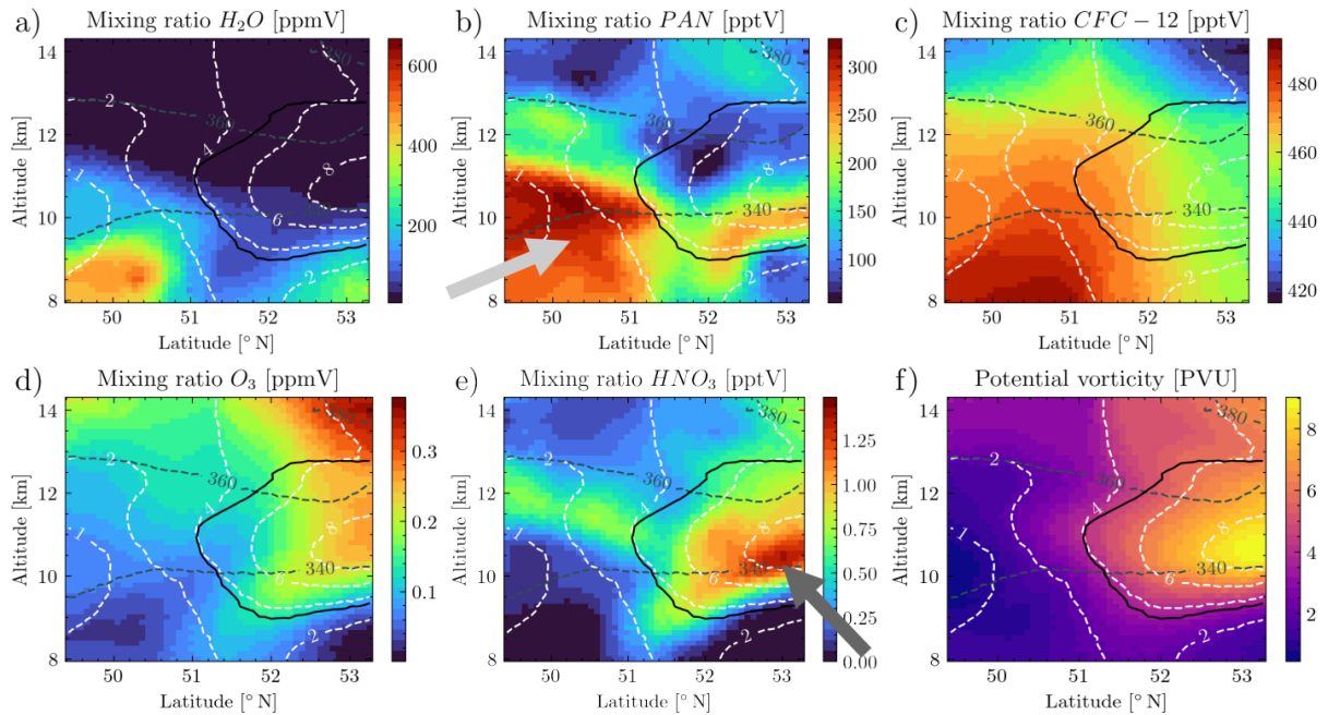
Figure 6. (a - e): Retrieved trace gas species inside the first hexagon (10 September 2023 UTC). f ): Potential vorticity derived from ERA5 reanalysis. The cross-section shown is the same as in Fig. 5a. The backgrounds are interpolated along constant longitude of 160°W. The dynamical tropopause and PV-isolines are indicated as black and white lines, respectively.
