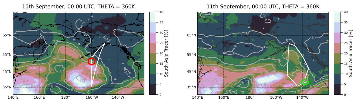
Figure 2. CLaMS South Asia tracer (= 'ECH' + 'TIB' + 'NIN' + 'IND' + 'BoB' + 'NIO', see Fig. 1) at 360K potential temperature. Synoptic situation during the measurement flights. Flight paths are shown as white lines. PV values are shown as gray isolines. The South Asia surface-origin tracer ('ECH' + 'TIB' + 'NIN' + 'IND' + 'BoB' + 'NIO', see Fig. 1) mixing ratios are shown in color. Left: Initial flight on 10 September 2023 UTC. A large filament with increased mixing ratios of South Asian air is projected to be in range of HALO research flights from the base in Anchorage. The first hexagon is located towards the end of the flight near the edge of the filament and is marked in red. Right: Follow-up flight on 11 September 2023 UTC. The filament 'rolls over' southeastwards. The second hexagon (marked in green) is located inside the outflow from the first hexagon (see Fig. 3) at that time.
