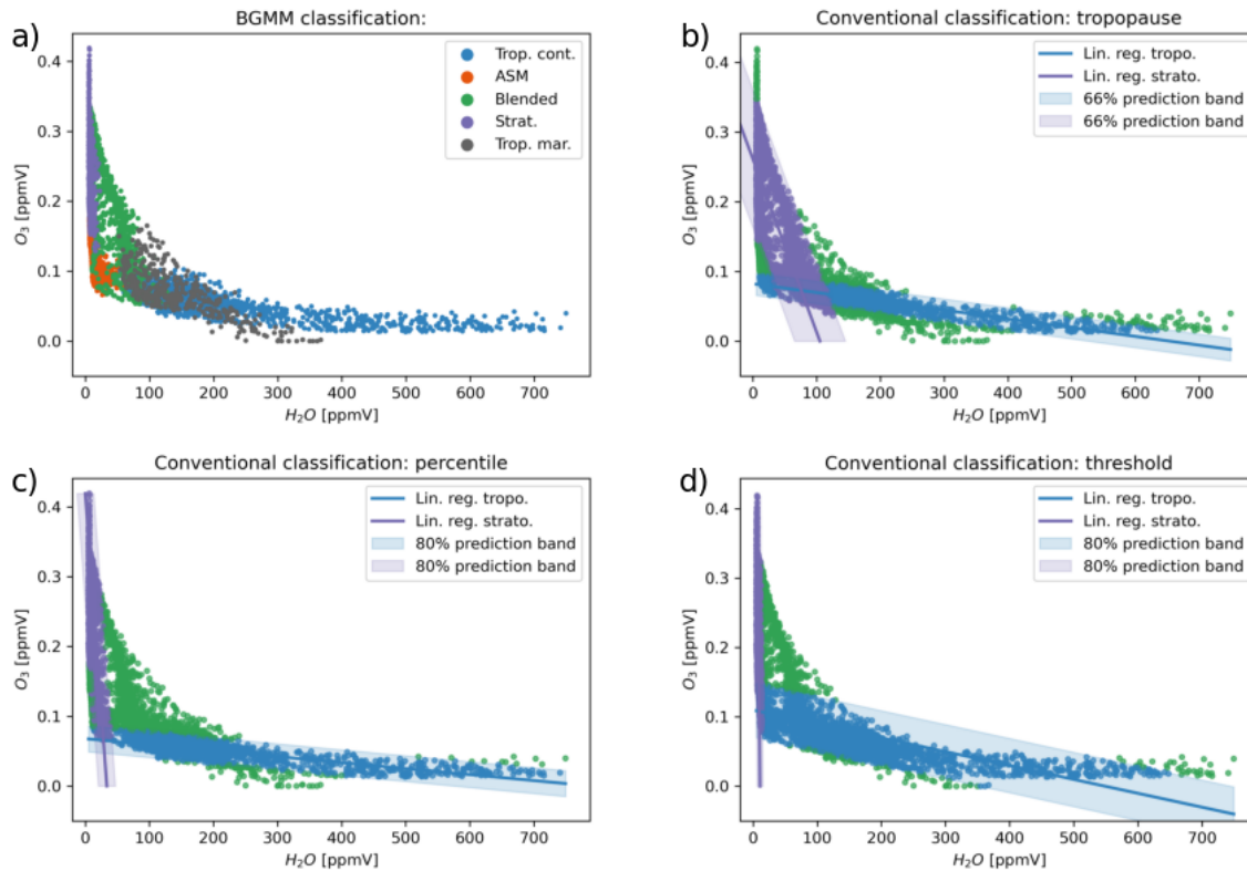
Figure B6. Comparison to conventional classification methods. Panel a: the BGMM classification presented in this study as a reference. Panel b: classification based on the thermal tropopause. The tropospheric (blue), stratospheric (purple) and mixed (green) regimes are determined by linear regression based on the trace gas species H_2O and O_3 above and below the tropopause. Panel c: classification based on thresholds determined by percentiles (80%) of the measured data. Panel d: classification based on commonly used thresholds. The conventional classifications include tropospheric air, stratospheric air and mixed air.
