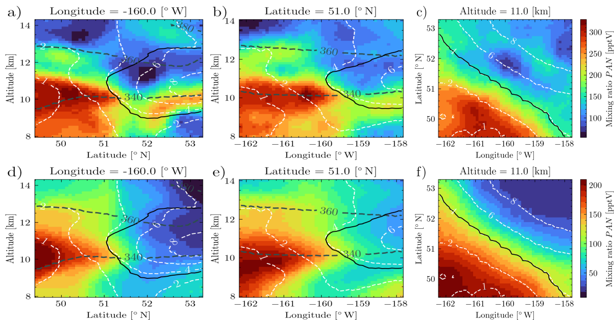
Figure 5. PAN mixing ratios inside the first hexagon on 10 September 2023 (upper row: GLORIA retrievals; lower row: CAMS model values predictions ). Shown are two vertical cross-sections (left and middle) and one horizontal one (right). PV isolines are shown as white dashed lines, potential temperature isolines are shown as gray dashed lines. The dynamical tropopause adapted from Kunz et al. (2015), which determines the PV-value depending on the potential temperature based on climatological data , is indicated as black line in all panels.
