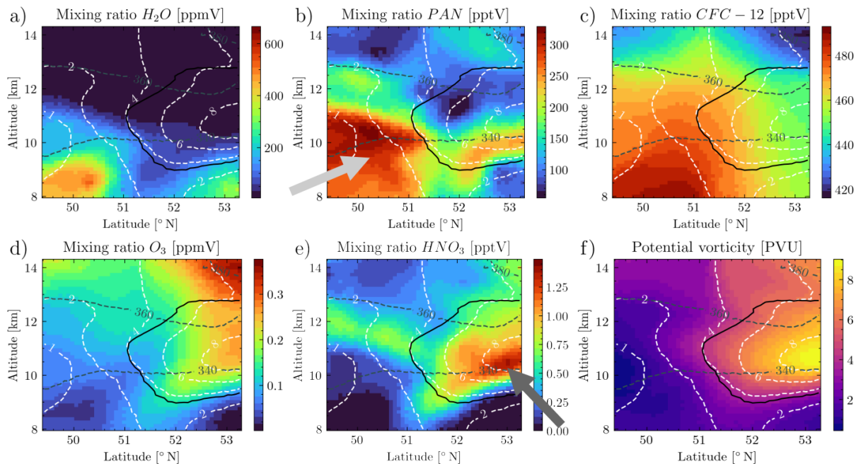
Figure 6. (a - e): Retrieved trace gas species inside the first hexagon (10 September 2023 UTC). f): Potential vorticity derived from ERA-5/ERA5 reanalysis. The cross-section shown is the same as in Fig. 5a. The backgrounds are interpolated along constant longitude of 160°W. The dynamical tropopause and PV-isolines are indicated as black and white lines, respectively.
