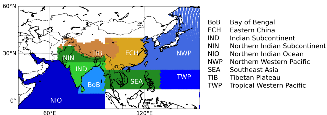
Figure 1. Definition and names Map of origin-surface-origin tracers used in CLaMS simulations associated with the PHILEAS campaign . Based on the work of Vogel et al. (2025) . Trajectories were calculated using ERA-5 data with 1^\circ \times 1^\circ horizontal resolution. global 3-dimensional CLaMS simulation for 2023 .
