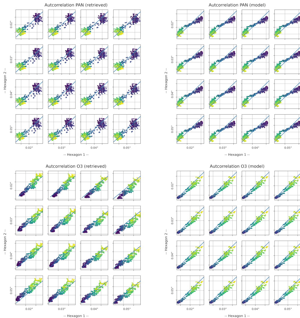
Figure A1. Comparison of different elevation angles on trajectory matching. Left hand side: retrieval results in hexagon 1 vs. hexagon 2 given a combination of elevation angles for PH13 and PH14. Right hand side: Same, but for model values. Shown are PAN and O 3 representatively.
