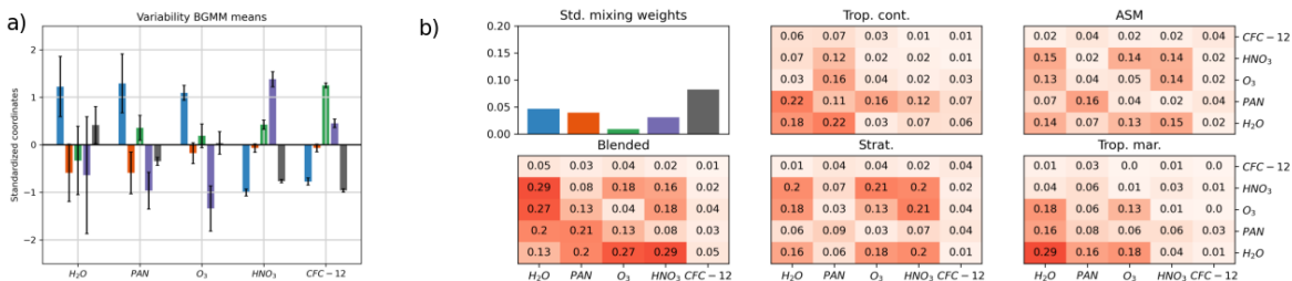
Figure B7. Robustness estimation for determined BGMM parameters. A total of 100 fits were performed and standard deviations of each parameter were determined. Panel a: Variability of the cluster centers. The standard deviation is shown as errorbar for each component of each cluster. Panel b: Variability of mixing weights (first plot) and the covariance matrices for each cluster. The scale of the standard deviations is indicated in color-code.
