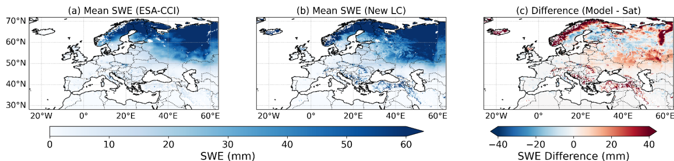
265 Figure 4: Maps of mean SWE values at altitudes below 1500 m across the whole of Europe from 2010 to 2022 derived from: (a) CCI SWE, (b) New LC, and (c) the difference between New LC and CCI SWE.
