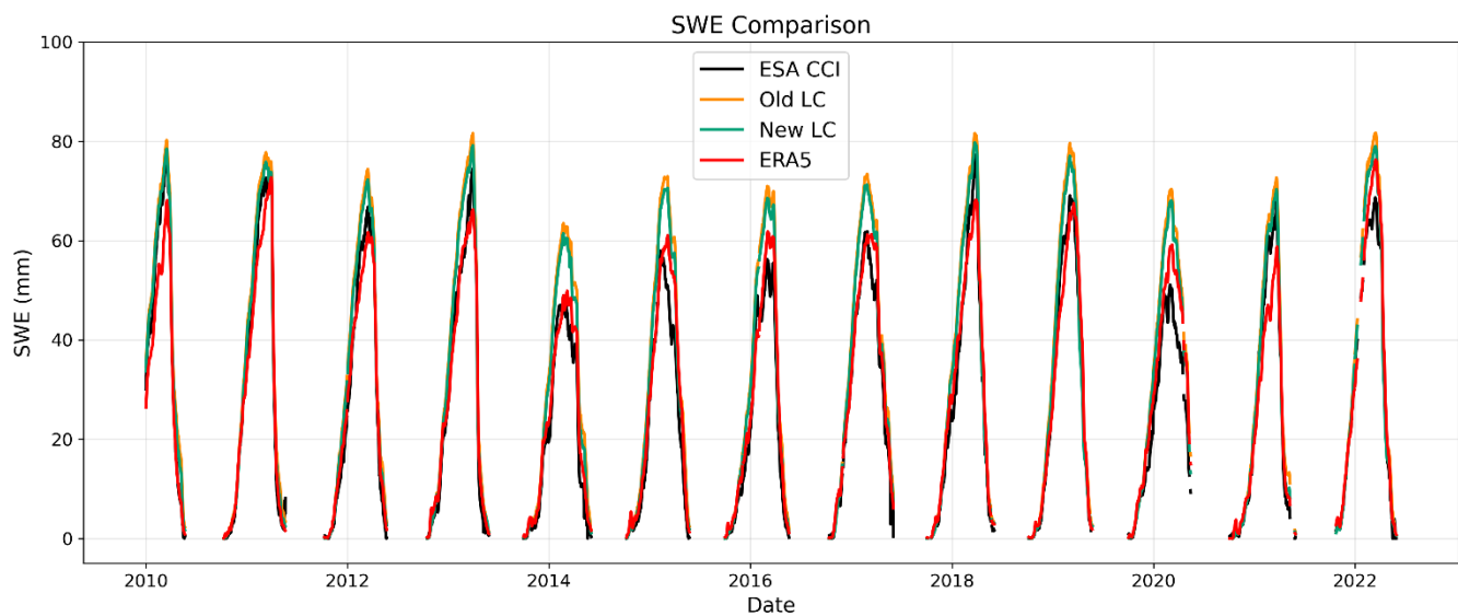
255 Figure 3: Time series of daily mean SWE values over the whole European domain from 2010 to 2022, based on the CCI SWE dataset, New LC, Old LC, and the ERA5 SWE.
