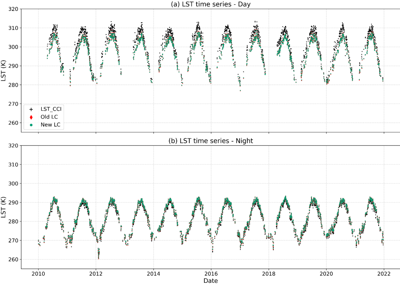
Figure 8: Time series of mean LST value over westernmost part of the domain (10°W-30°E, 28.125°N-71.875°N) from CCI LST, Old LC and New LC from 2010 to 2022: (a) daytime values at 13:30 LT for CCI LST, (b) nighttime at 01:30 LT, corresponding to ISBA simulations at 12:00 and 00:00 UTC, respectively.
