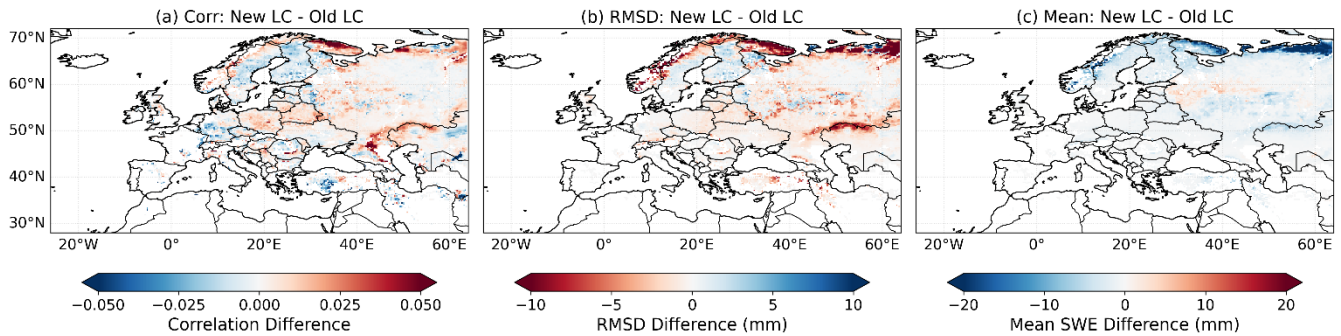
285 Figure 5: Spatial differences in the statistical performance metrics of New LC and Old LC SWE simulations with respect to CCI SWE over the whole European domain, over the 2010–2022 period: difference in (a) R, (b) RMSD and (c) mean difference of SWE between the two simulations. For R and RMSD, red zones indicate improvement (e.g. higher correlations or lower errors) when using New LC, while blue zones indicate degradation.
