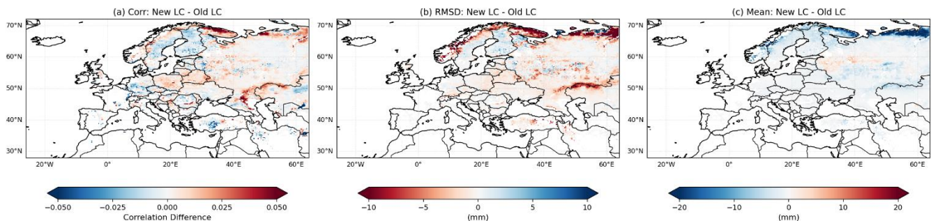
275 Figure 5: Spatial differences in the statistical performance metrics of New LC and Old LC SWE simulations with respect to CCI SWE over the whole European domain, over the 2010–2022 period: difference in (a) R , (b) RMSD and (c) mean difference of SWE between the two simulations. For R and RMSD, red zones indicate improvement (e.g. higher correlations or lower errors) when using New LC, while blue zones indicate degradation.
