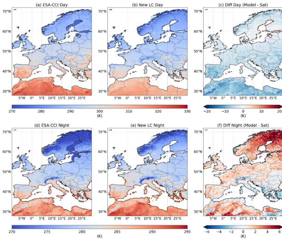
Figure 9: Maps showing the mean (a,b,c) daytime and (d,e,f) nighttime (bottom) LST values over westernmost part of the domain (10°W-30°E, 28.125°N-71.875°N) for the period 2010–2022, derived from (a, d) CCI LST, (b, e) New LC and (c, f) the difference between New LC and CCI LST.
