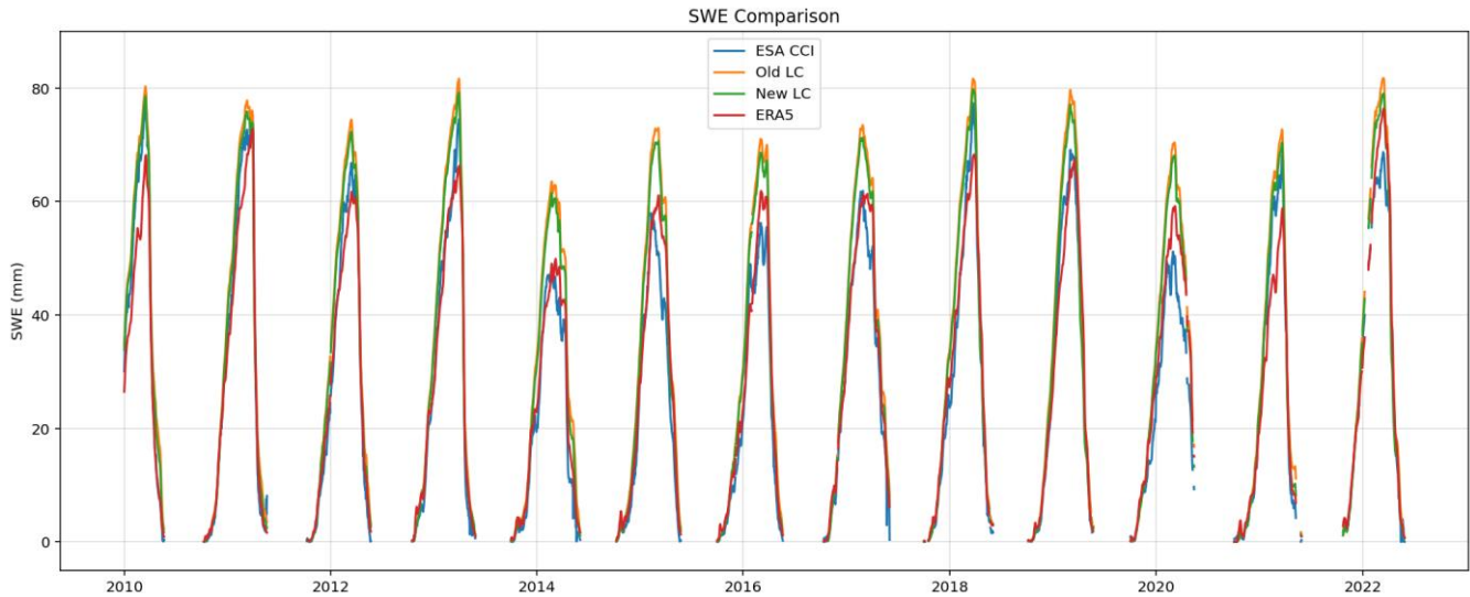
245 Figure 3: Time series of daily mean SWE values over the whole European domain from 2010 to 2022, based on the CCI SWE dataset, New LC, Old LC, and the ERA5 SWE.
