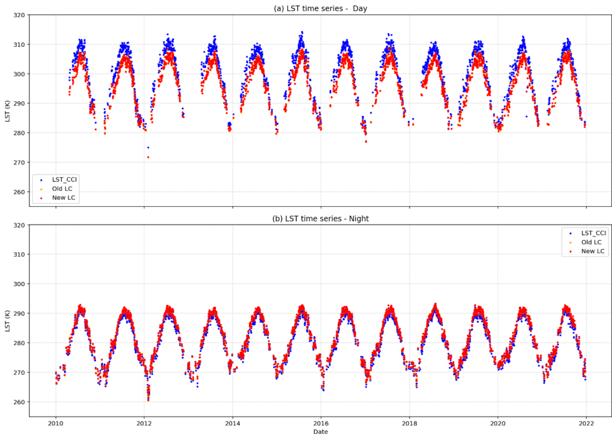
340 Figure 8: Time series of mean LST value over westernmost part of the domain (10°W-30°E, 28.125°N-71.875°N) from CCI LST, Old LC and New LC from 2010 to 2022: (a) daytime values at 13:30 LT for the observations CCI LST, (b) nighttime at 01:30 LT, corresponding to ISBA simulations at 12:00 and 00:00 UTC, respectively.
