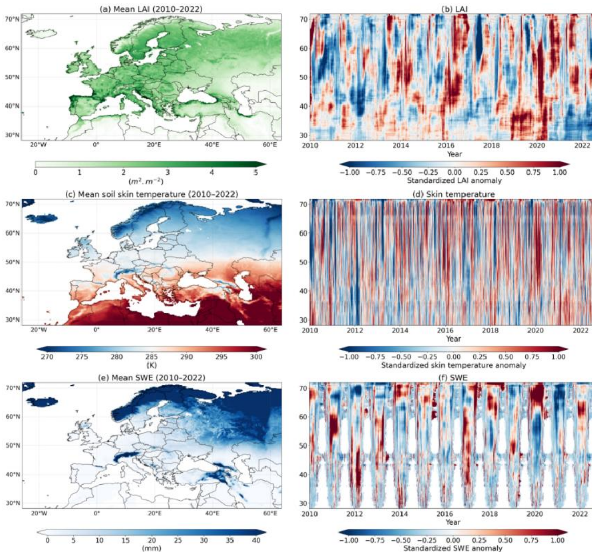
Figure 2: New LC simulations over the whole European domain forced by ERA5 atmospheric variables from 2010 to 2022 at a spatial resolution of 0.25 degree x 0.25 degree: Mean values (a, c, e) and Hovmöller plot (b, d, f) of scaled anomalies (z-score) of (a, b) LAI, (c, d) LST, and (e, f) SWE.
