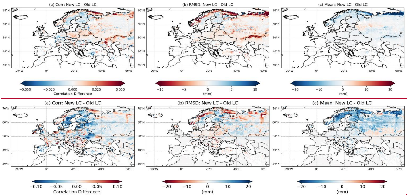
Figure 5: Spatial differences in the statistical performance metrics of New LC and Old LC SWE simulations with respect to CCI SWE observations over the whole European domain, over the 2010–2022 period: difference in (a) R , (b) RMSD and (c) mean difference of SWE between the two simulations. For R and RMSD, red zones indicate improvement (e.g. higher correlations or lower errors) when using New LC, while blue zones indicate degradation.
