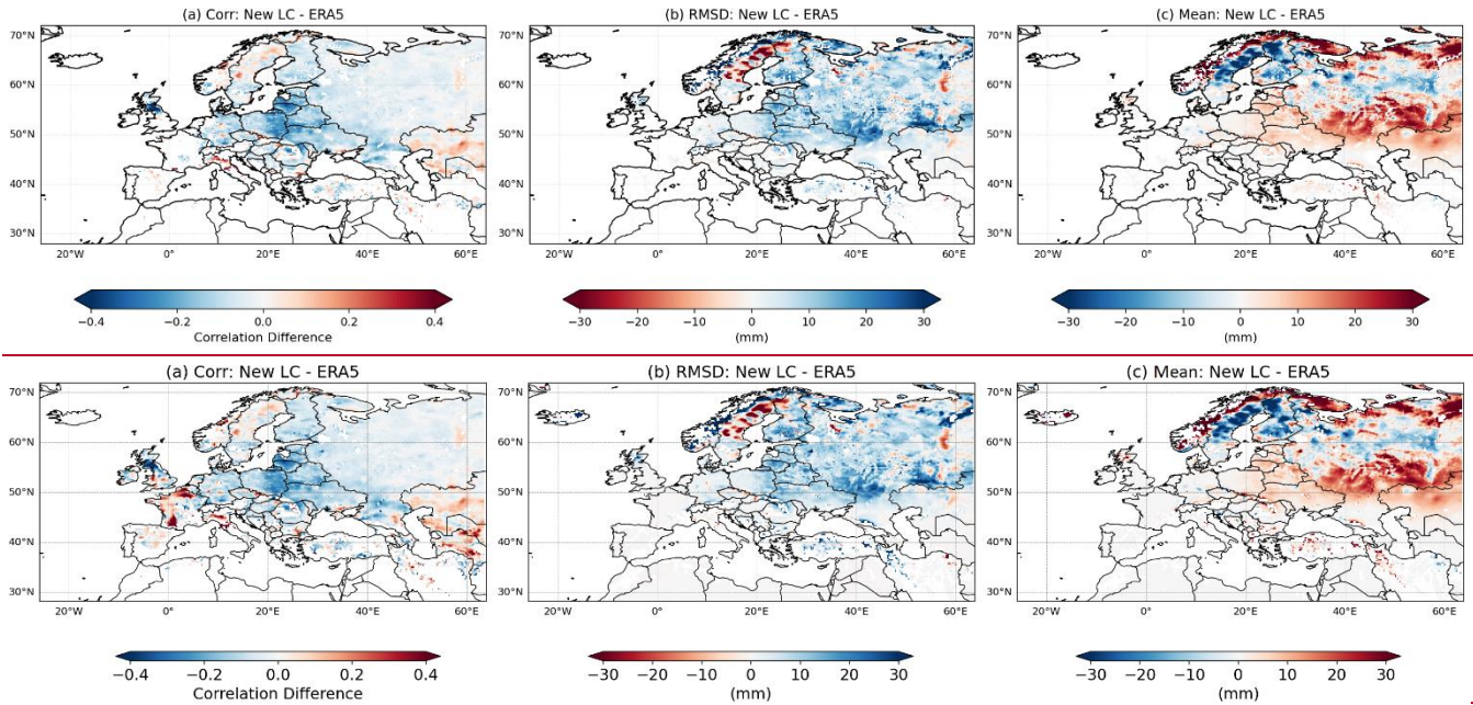
Figure 6: As in Fig. 5, except for differences between New LC and ERA5.
