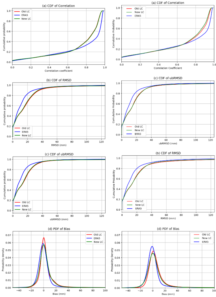
Figure 7: Cumulative distribution functions (CDFs) of (a) R , (b) RMSD, and (c) ubRMSD, alongside (d) the probability density function (PDF) of the bias, for SWE simulations from Old LC, New LC, and ERA5 (red, green, and blue, respectively), benchmarked against CCI SWE the whole European domain for the period 2010–2022.
