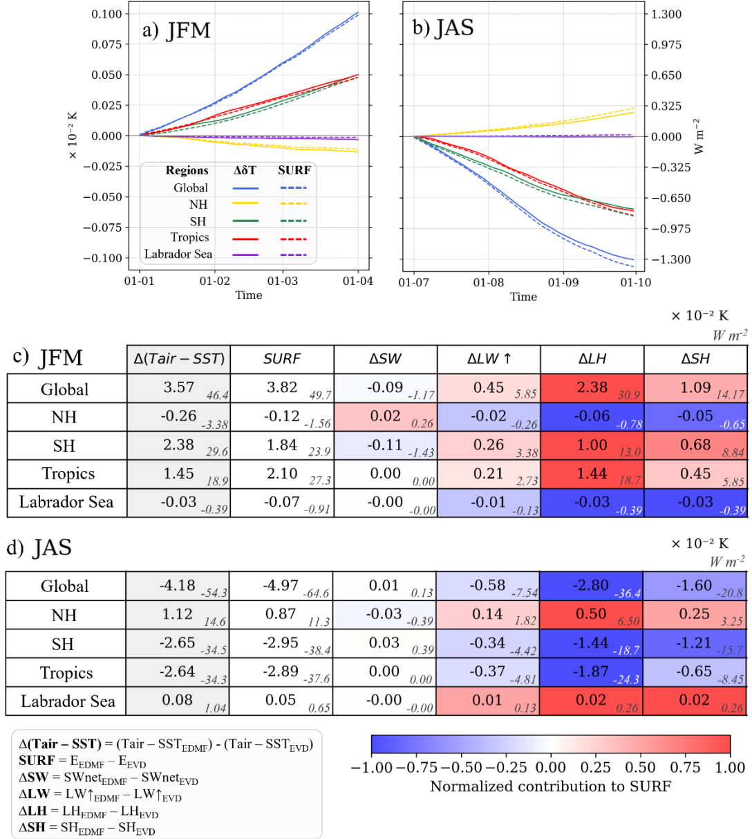
Figure 10: Time series of SURF ( 10^{-2} K on the left y-axis; W m^{-2} on the right y-axis) for the climatological seasons of JFM (a) and JAS (b), computed for the global, northern hemisphere (NH), southern hemisphere (SH), tropical oceans and the Labrador Sea. Corresponding cumulative values of SURF, \Delta SW , \Delta LW_{\uparrow} , \Delta LH , \Delta SH , expressed in 10^{-2} K and in W m^{-2} (in italics) for JFM (c) and JAS (d). The sign convention of these values is given in Eq. 13. The colorbar indicates the normalized contribution of each heat flux component to SURF.
