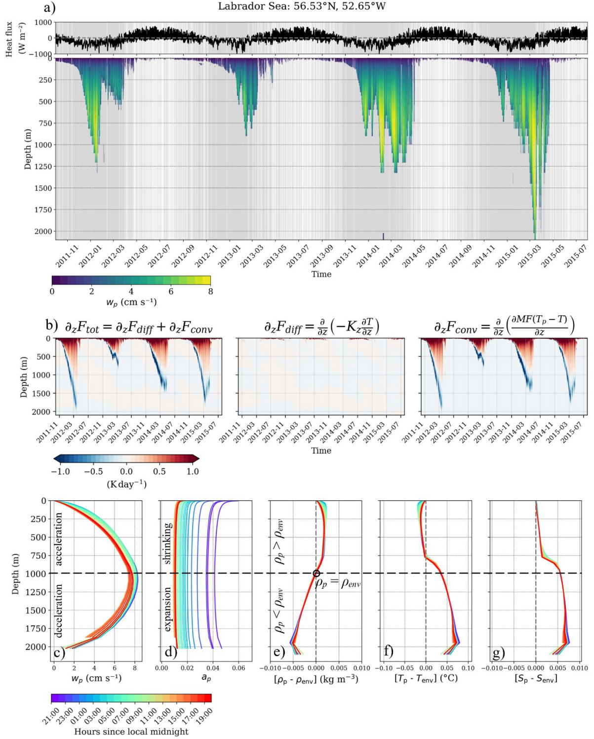
350 Figure 2: (a) Hourly time series of surface net heat flux ( \text{W m}^{-2} ) and plume w_p ( \text{cm s}^{-1} ) spanning October 2011 to July 2015 at mooring location 56.53°N, 52.65°W in the Labrador Sea. (b) Daily time series of temperature trend ( \text{K day}^{-1} ) from the divergence of the total ( \partial_z F_{\text{tot}} ), diffusive ( \partial_z F_{\text{diff}} ) and convective ( \partial_z F_{\text{conv}} ) heat flux from EDMF simulation. Fluxes are computed at the model grid cell containing the mooring location and over the same time window as shown in (a). 24-hours profiles of (c) w_p , (d) a_p , (e) \rho_p - \rho_{\text{env}} , (f) T_p - T_{\text{env}} and (g) S_p - S_{\text{env}}
