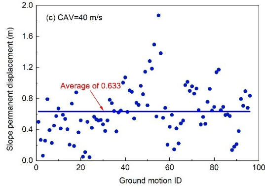
Fig. 5. Displacement response distribution of slopes under MAS. The horizontal axis (Ground motion ID) represents the serial number of ground motion records (ID = 1–96).
