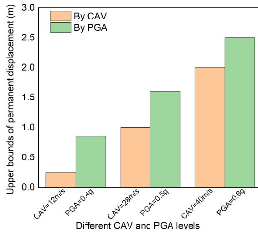
Fig. 6. Upper bounds of permanent displacement at different CAV and PGA levels
