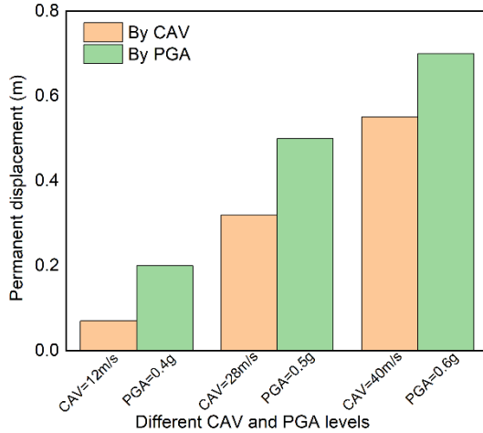
Fig. 8. Slope permanent displacement at a CDF of 50%
