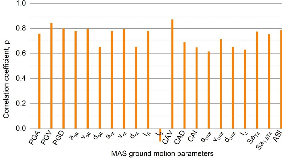
Fig. 2. Correlation coefficient of MAS ground motion parameters (PGA: peak ground acceleration; PGV: peak ground velocity; PGD: peak ground displacement; a_{sq} : squared acceleration; v_{sq} : squared velocity; d_{sq} : squared displacement; a_{rs} : root square acceleration; v_{rs} : root square velocity; d_{rs} : root square displacement; I_A : Arias intensity; t_d : significant duration; CAV: cumulative absolute velocity; CAD: cumulative absolute displacement; CAI: cumulative absolute impulse; a_{rms} : root-mean-square acceleration; v_{rms} : root-mean-square velocity; d_{rms} : root-mean-square displacement; I_c : characteristic intensity; Sa_{Ts} : response spectral acceleration at natural vibration period T_s ; Sa_{1.5Ts} : response spectral acceleration at 1.5T_s ; ASI: acceleration spectral intensity.)
