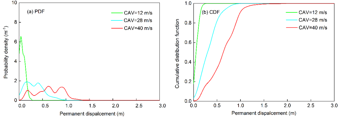
Fig. 7. Statistical analysis of slope permanent displacement probability under MAS. Probability Density Function (PDF), describing the probability density of permanent displacement, and Cumulative Distribution Function (CDF), representing the cumulative probability of permanent displacement.
