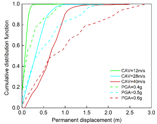
Fig. 9. Compared with the reliability results of slope displacement response in reference (Wang et al., 2022)
