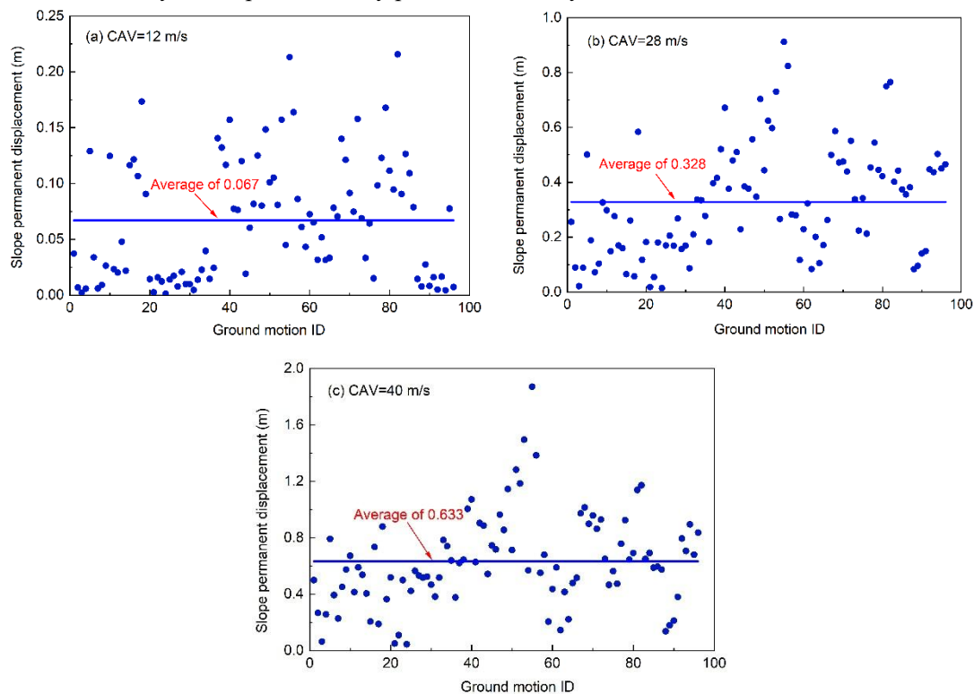
Fig. 5. Displacement response distribution of slopes under MAS. The horizontal axis (Ground motion ID) represents the serial number
