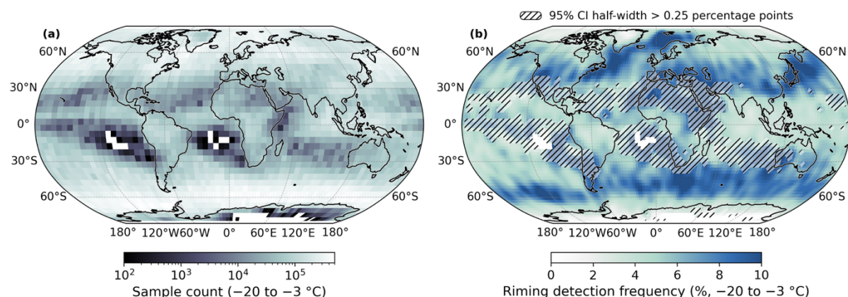
Figure 9: Global distributions of (a) sample count for the targeted echoes and (b) riming detection frequency in stratiform clouds between -20 and -3 °C during 2025. Both quantities are calculated on a 5^\circ \times 5^\circ grid. For visualization, the riming detection frequency in panel (b) is rendered at 2.5^\circ spacing with light smoothing. Hatching marks grid cells where the nominal 95% Wilson confidence interval (CI) half-width exceeds 0.25 percentage points (i.e., less precise estimates).
