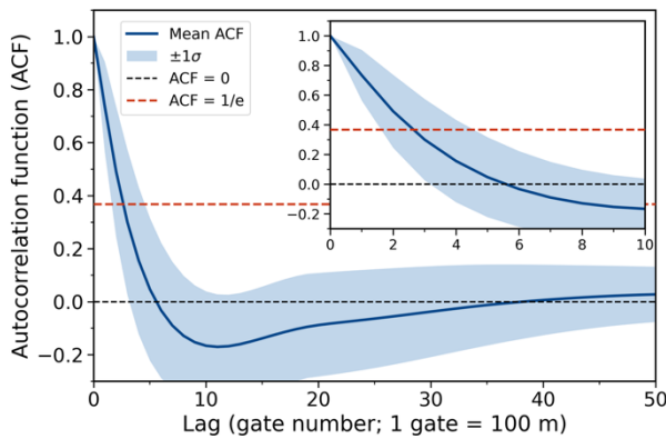
Figure B1: Autocorrelation function (ACF) of V_{SED} residuals calculated from one year of EarthCARE CPR data. The solid blue line indicates the mean ACF, while the shaded area represents the \pm 1\sigma variability. The dashed orange line denotes the 1/e decorrelation level. The inset provides a detailed view of the short-range correlation structure for lags 0 to 10.
