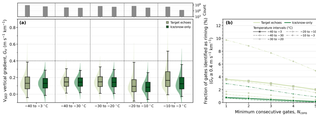
Figure 4: (a) G_V distributions for the targeted echoes used for riming detection (pale green) and the ice/snow-only subset (green) from one year of EarthCARE observations in 2025. The first pair of boxplots covers the temperature range considered for riming detection ( -40 to -3 °C), and the remaining pairs correspond to four temperature intervals. Bars above indicate the number of gates. Box and half violin plots
