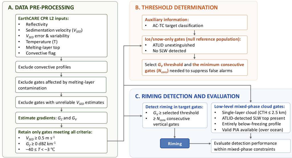
Figure 1: Overview of the CPR-based riming detection methodology, including data preprocessing, threshold determination, riming detection, and independent evaluation using SLW observations.
