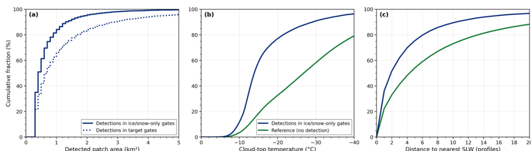
Figure C1: Cumulative distributions for detections in ice/snow-only gates between −10 and −3 °C. Panel (a) shows the area of connected detection patches in the ice/snow-only subset (solid line) and in the target gates (dotted line). Panels (b) and (c) show cloud top temperature and proximity to ATLID-detected SLW for profiles containing detections (blue) and reference profiles with no detection (green). The median reference distribution is shown.
