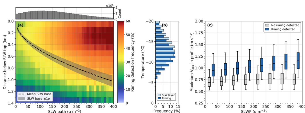
Figure 6: (a) Riming detection frequency for LLMPCs from one year of EarthCARE observations in 2025 as a function of distance below the SLW top and SLWP. Bin sizes are 100 \text{ m} and 10 \text{ g m}^{-2} , respectively. The black dashed line and gray shading indicate the estimated mean SLW base and its standard deviation. Bars above indicate the number of gates in each SLWP bin. (b) Temperature distributions of the SLW layer (between the SLW top and base; light blue) and detected riming (blue), using 1^{\circ}\text{C} bins. (c) Distributions of the maximum V_{SED} in profiles with and without riming detection (blue and gray, respectively) as a function of SLWP. Boxplots are presented in 50 \text{ g m}^{-2} SLWP bins and follow the format of Fig. 3f.
