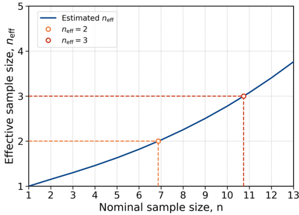
Figure B2: Effective sample size ( n_{\text{eff}} ) as a function of nominal regression window length ( n ), estimated from the mean ACF shown in Fig. B1 following Eq. (B2).
