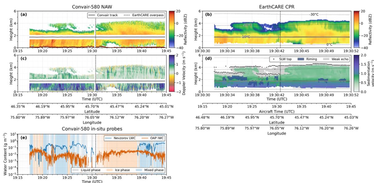
Figure 7: Collocated EarthCARE (Orbit/Frame ID: 04681D) and NRC Convair-580 observations acquired during ECALOT Flight 7 on 25 March 2025. Panels (a) and (c) show reflectivity and Doppler velocity from the NRC NAW, and panels (b) and (d) show EarthCARE CPR reflectivity and sedimentation velocity. EarthCARE observations are mapped to the nearest position along the Convair-580 flight track. The horizontal solid and vertical dashed lines denote the flight altitude and the point of satellite–aircraft coincidence, respectively. In panel (d), detected riming is shown as blue hatched areas. Black dots indicate the ATLID-detected SLW top. Panel (e) shows liquid water content (LWC; blue line) from the Nevzorov probe and ice water content (IWC; orange line) from the optical array probes (OAP). Background shading indicates cloud phase based on LWC and IWC thresholds of 0.01 and 0.001 g m -3 , respectively.
