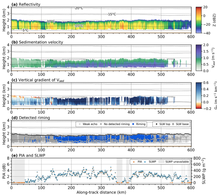
440 Figure 5: Example of a low-level mixed-phase cloud (LLMPC) observed by EarthCARE over the Southern Ocean on 12 January 2025 (Orbit/Frame ID: 03550H). Panels (a)–(d) show reflectivity, sedimentation velocity, the vertical gradient of sedimentation velocity, and the detected riming (blue areas), respectively. Filled and open circles in panel (d) indicate the ATLID-detected SLW top and the estimated SLW base. Panel (e) shows path-integrated attenuation (PIA; orange dots) and the corresponding supercooled liquid water path (SLWP; teal dots) where available. In this case, areas without an SLWP estimate (gray shading) are mostly found where PIA is 0 dB.
