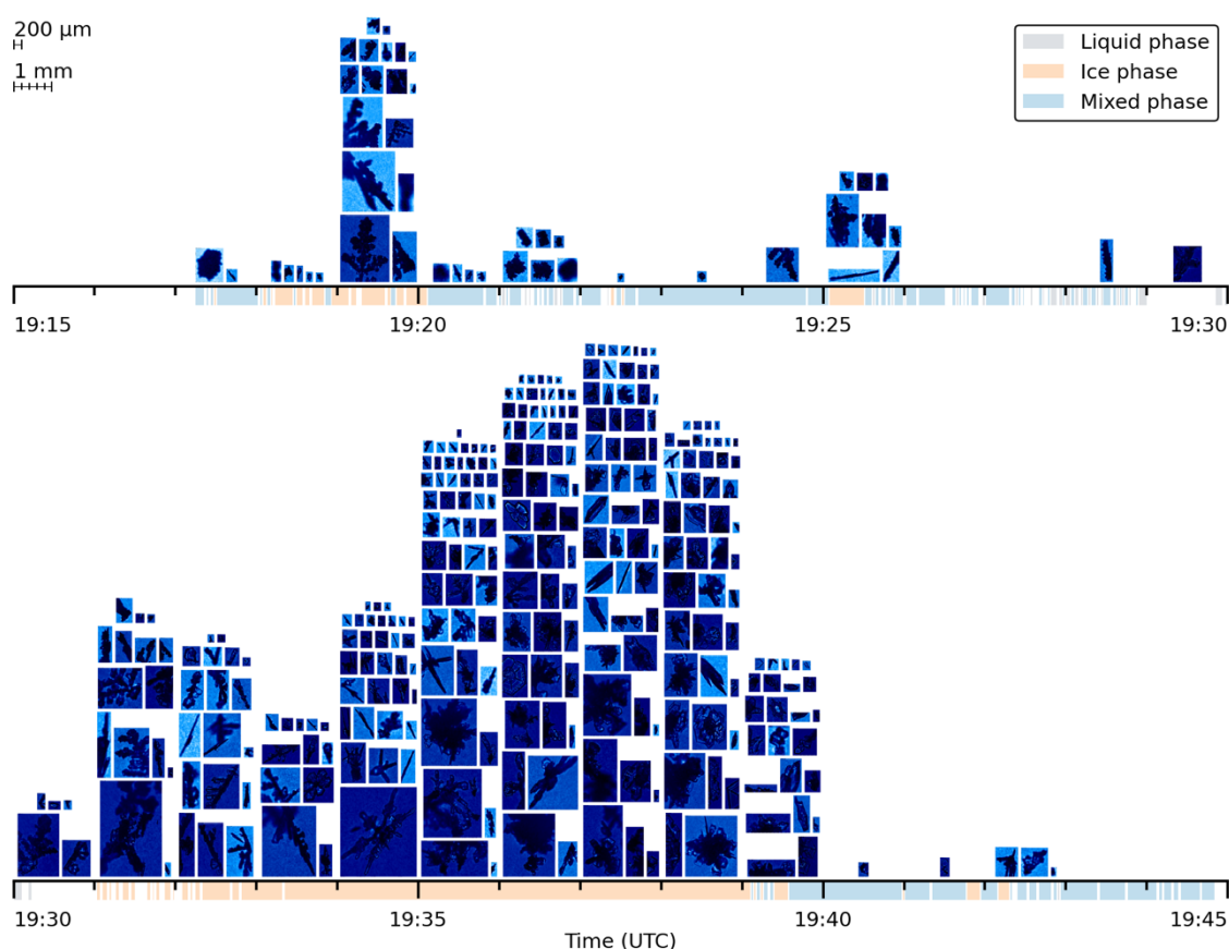
Figure 8: Cloud particle imager (CPI) images of ice particles from the flight transect shown in Fig. 7. Images observed within each 1 min interval are shown together, where larger images are generally placed toward the bottom. The colored strip beneath the time axis indicates the cloud phase from Fig. 7c.
