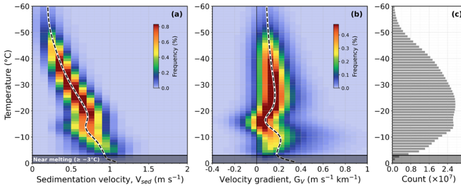
Figure 2: Joint distributions of EarthCARE CPR (a) sedimentation velocity ( V_{SED} ) and (b) its vertical gradient ( G_V ) against temperature for stratiform ice clouds where reflectivity increases downward. One year of data from January to December 2025 is used. Panel (c) shows the number of samples in each temperature bin. The dashed black lines represent the mean values at each temperature bin. The shaded area warmer than -3 \text{ }^\circ\text{C} indicates the region excluded to avoid melting layer contamination.
